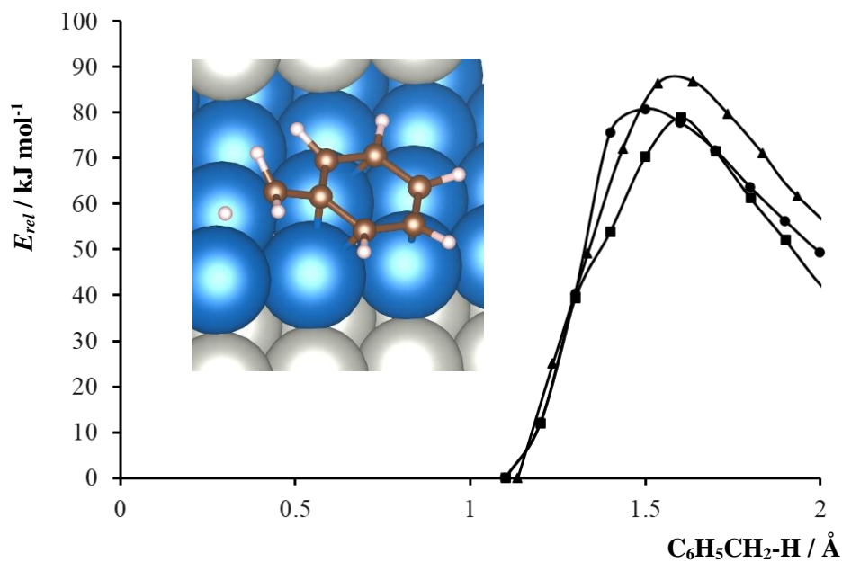
Figure 7. Calculated barriers for C 6 H 5 CH 2 -H bond cleavage over Pd(111) (circles), Pd(211) step (triangles) and Pd(211) terrace (squares). Energy is taken relative to the adsorbed toluene state in each case. Inset graphic shows the calculated transition state for Pd(211) terrace. Atom colours: Pd : grey, with terrace atoms blue, C : Brown, H: white.
