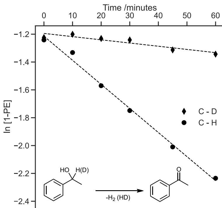
Figure 1 – Kinetic Isotope Effect of Deuteration of the \alpha -carbon in 1-phenylethanol Acceptorless Dehydrogenation
