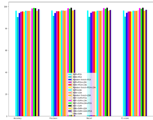
Figure 5. Evaluation diagrams of machine learning methods and RBF model
