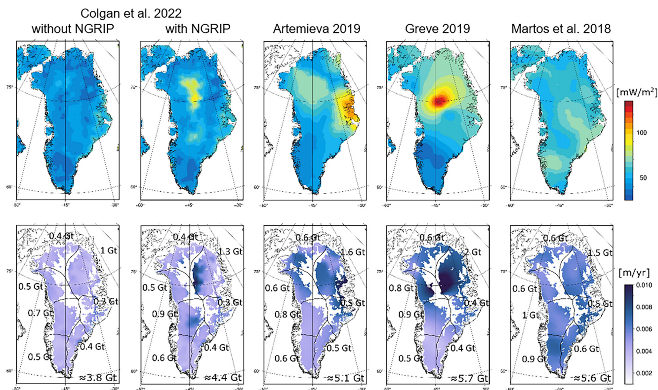
Fig. 2. Estimates of Greenland's GHF (top row) and associated basal melting (bottom row) for a suite of models. Corresponding GHF model sources are listed above each column. Areas considered as being frozen are masked. (Note the wide range of basal melt estimates, from 3.8 to 5.7 Gt a -1 .) Source: all basal melting estimates were calculated following the method of Karlsson et al. (2021) .
