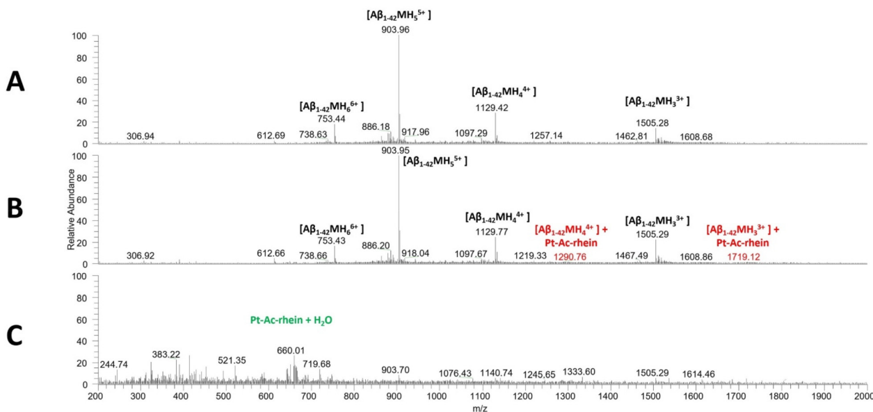
Fig. 3 ESI-MS spectra of Aβ 1-42 (A) in the absence and (B) presence of Pt-Ac-rhein, and (C) the spectrum of the latter compound alone.
