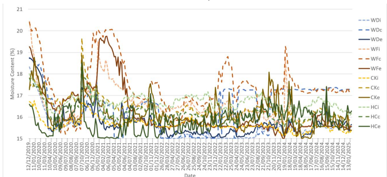
Figure 6. Wood Moisture Content at horizontal junction between Lime-Hemp finished panels and timber frame 12/12/2019 – 05/02/2025.
