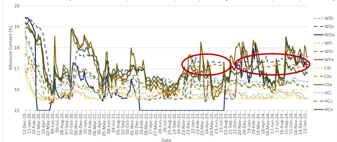
Figure 4. Wood Moisture Content at mid-point of Lime-Hemp finished panels 12/12/2019 – 05/02/2025. High moisture content at centre of Wattle & Daub (WDe) and Wood Fibre (WFc) panels highlighted.
