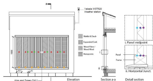
Figure 2. Monitoring positions in elevation (Red-centre of panel, Orange-midpoint of horizontal junction, Green-midpoint of vertical junction) and section (Cyan-interface external render and infill, Blue-midpoint of infill, Purple-interface internal render and infill).
