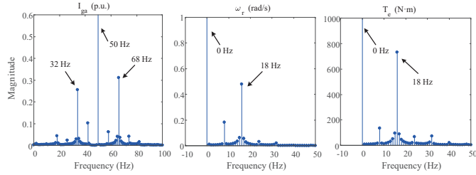
Fig. 11. Frequency-domain spectra of the weak-grid-tied PMSG system showing that oscillations take place at 68 Hz and 32 Hz.
