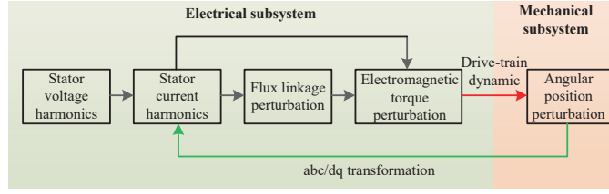
Fig. 7. Electro-mechanical coupling effect illustration in PMSG-WT.
