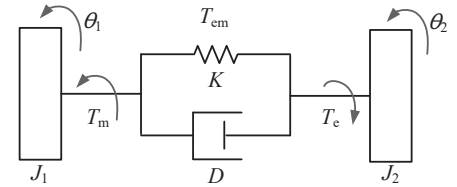
(b) Two mass-spring mechanical subsystem model.
