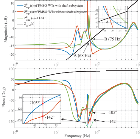
(a) Bode plot of system impedance.
