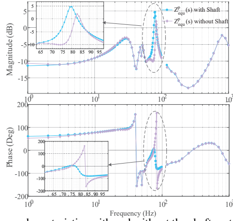
Fig. 5. Comparison between the impedance characteristics with and without the shaft system model. Lines: analytical model. Dots: simulation measurement.
