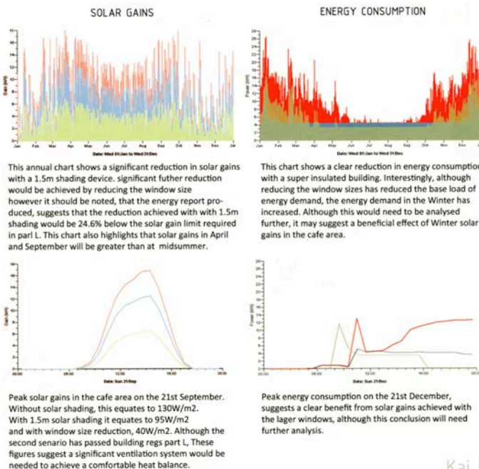
Figure 6: Energy / thermal comfort models by student Kai Edwards, TECN201, May 2013
