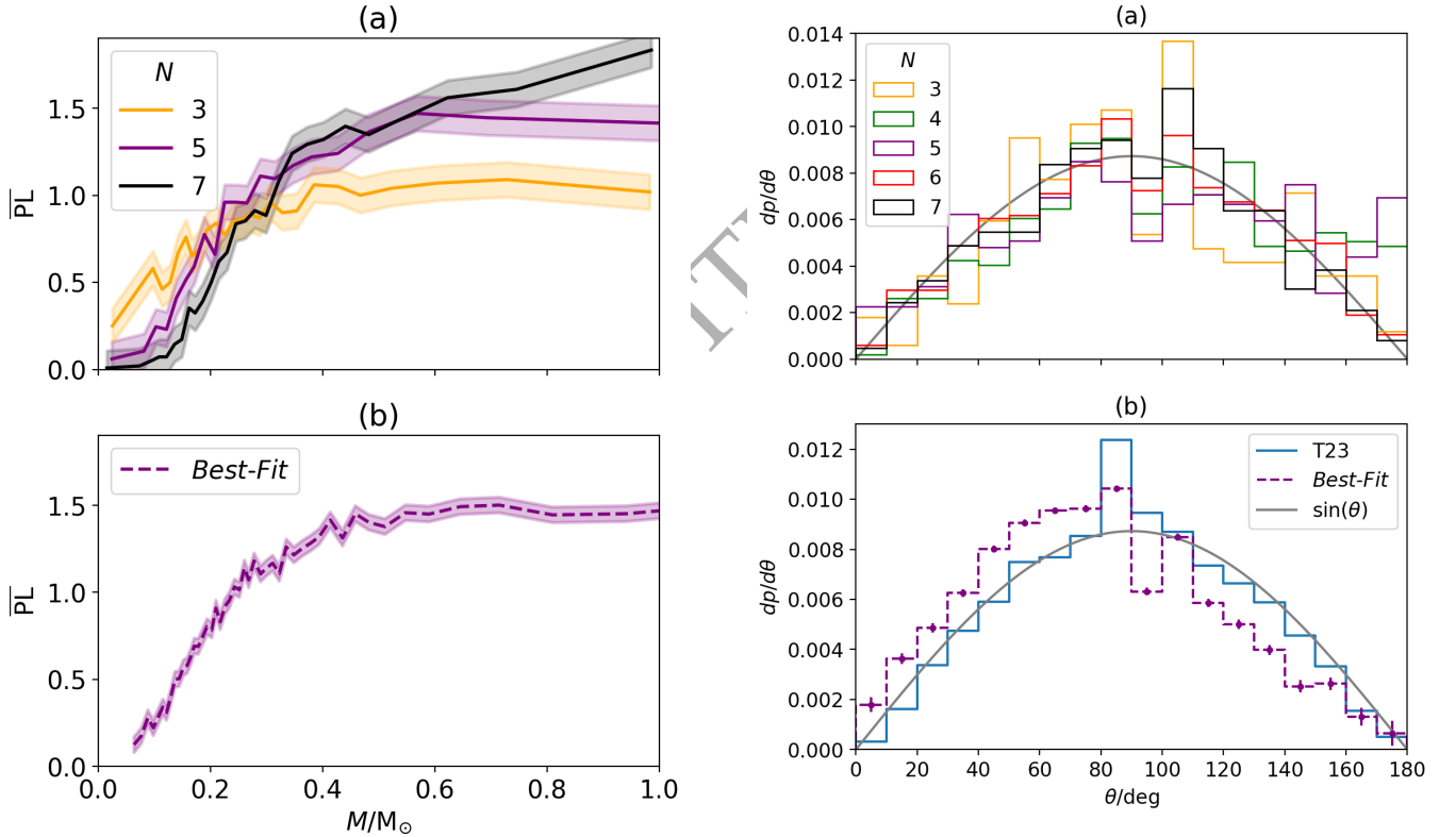
Figure 7. The specific probability distributions of mutual orbital inclination, \theta , for \theta_o in degrees. (a) The Fiducial Case with N=3, 4, 5, 6, 7 . (b) The Best-Fit Case and for the observed systems in the T23 catalogue. Figure 7a is produced using 2000 realizations for each N value, in order to improve signal-to-noise.
