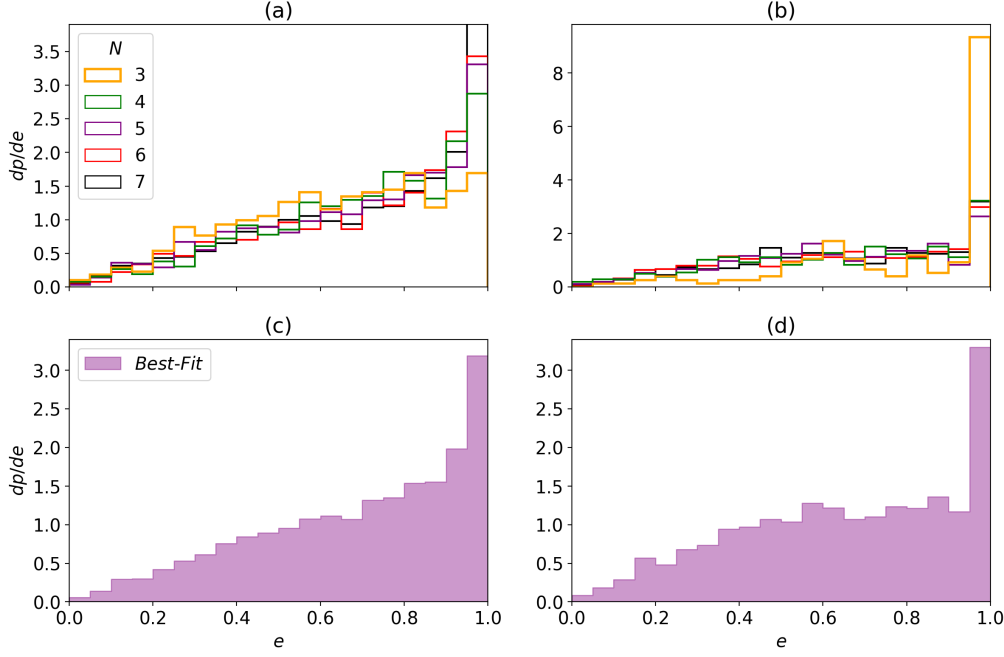
Figure 10. The specific probability distributions of eccentricity, e . (a) S2 orbits, (b) S1 orbits, for the Fiducial Case with N=3, 4, 5, 6, 7 . (c) S2 orbits, (d) S1 orbits, for the Best-Fit Case .
