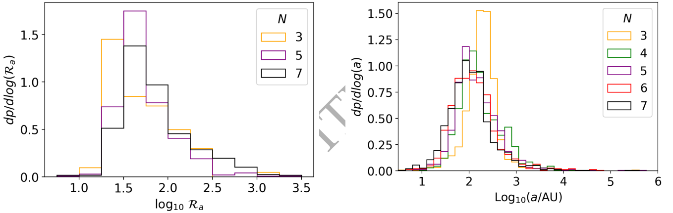
Figure 3. The specific probability distributions of semi-major axis, a , for S2 orbits from the high-rotation case discussed in Section 3.1.3 (i.e. \alpha_{\text{rot}} = 0.99 , \alpha_{\text{law}} = \text{SOL} , \alpha_{\text{seg}} = 0 , so almost all the kinetic energy in solid-body rotation, and no mass segregation) with N=3, 4, 5, 6, 7 .
