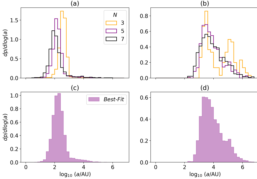
Figure 1. The specific probability distributions of semi-major axis, a , for (a) S2 orbits, and (b) S1 orbits, in the Fiducial Case with N=3, 5 and 7 ; the results for N=4 and 6 are omitted to avoid confusion. (c) and (d) show the specific probability distributions for the Best-Fit Case .
