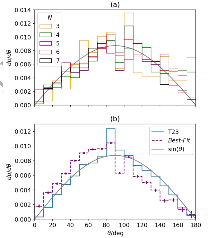
Figure 7. The specific probability distributions of mutual orbital inclination, \theta , for \theta_o in degrees. (a) The Fiducial Case with N=3, 4, 5, 6, 7 . (b) The Best-Fit Case and for the observed systems in the T23 catalogue. Figure 7a is produced using 2000 realizations for each N value, in order to improve signal-to-noise.
