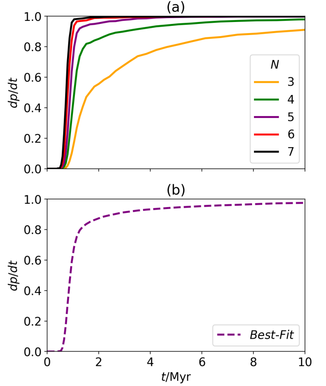
Figure 13. The cumulative probability distributions of the first ejection as a function of the elapsed time. (a) The Fiducial Case with N=3, 4, 5, 6, 7 . (b) The Best-Fit Case .
