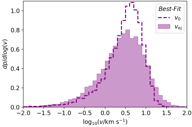
Figure 12. The specific probability distributions of initial velocity ( v_0 ) and ejection velocity ( v_{ej} ) for all stars in the Best-Fit Case .
