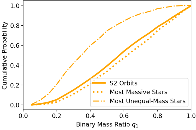
Figure 4. The cumulative probability distributions of mass ratio, q_1 . Solid Line: S2 orbits of systems formed dynamically in the Fiducial Case with N = 3 . Dotted Line: values obtained by simply pairing the 2 most massive stars. Dash-Dotted Line: values obtained by pairing the most and least massive stars.
