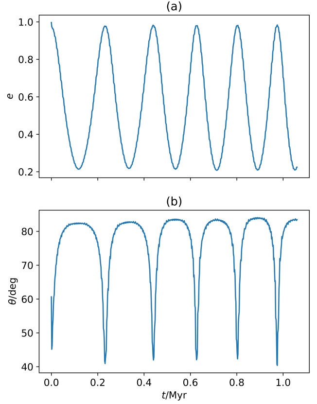
Figure 9. An hierarchical triple system undergoing von Zeipel-Lidov-Kozai cycles. (a) The eccentricity, e , of the inner S2 orbit, as a function of time. (b) The corresponding mutual orbital inclination, \theta .
