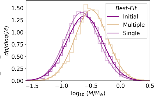
Figure 11. The mass distributions for all stars, for those that end up in multiples, and for those that end up single, in the Best-Fit Case . Means and standard deviations are given in Table 2.
