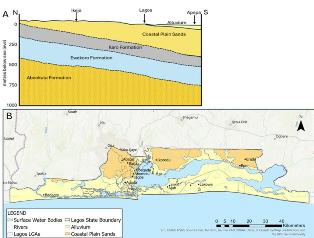
Figure 1: (a) generalised schematic geological cross-section for Lagos State. Vertical exaggeration applied, accentuating the apparent dip of the formations. (b) surface geology of Lagos State (geological shapefile modified after Olabode & Comte, 2024). LGA = Local Government Areas. Basemap: Esri, CGIAR, USGS, TomTom, Garmin, FAO, NOAA, USGS © OpenStreetMap contributors, and the GIS User Community. BGS © UKRI 2025.
