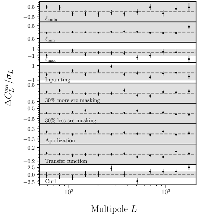
FIG. 7. Comparison of difference bandpowers ( \Delta C_L^{\kappa\kappa} ) between the baseline analysis and those where we vary a given analysis setting, scaled by the uncertainties of the respective \phi^{TT} bandpowers. The error bars represent the standard deviations of the shifts for 340 simulations with the same analysis choice change. The shaded gray regions represent the 1\sigma bands of the \phi^{TT} estimators.
