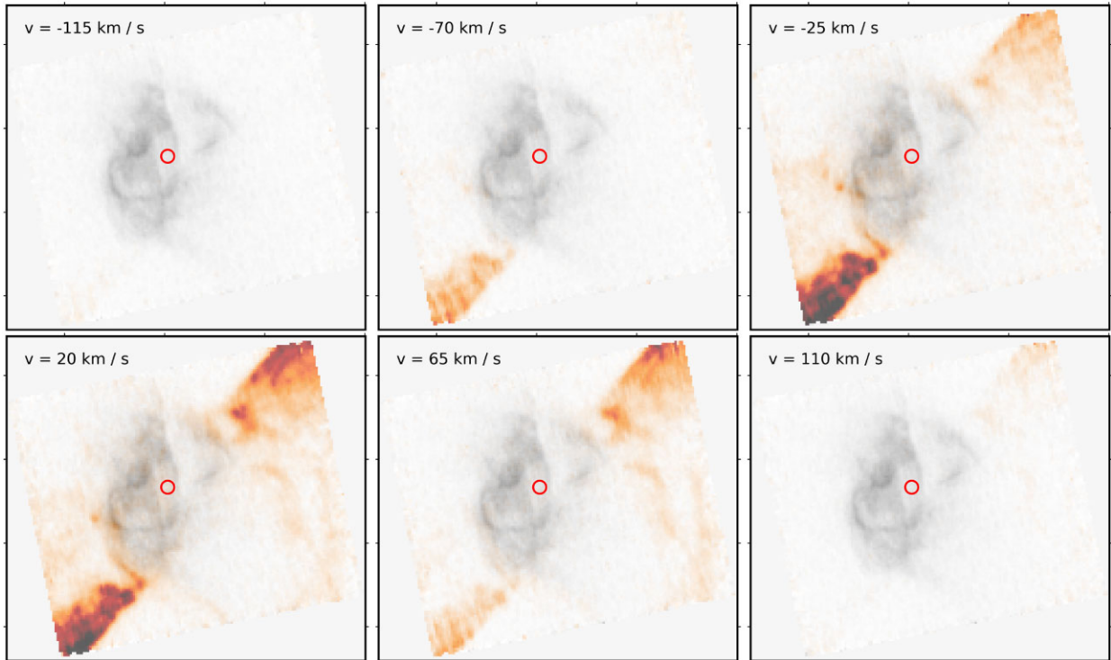
Figure 5. The MIRI channel map of the 5.3\ \mu\text{m} [Fe II] jet is shown. The jet, highlighted in red, extends from the south-east and the north-west edges of the outer bubble. The south-eastern part of the jet is blueshifted, while the north-western part is redshifted. The velocity labels represent rest-frame velocities in the LSR, obtained by subtracting the radial velocity of NGC 6302 from the velocities measured with MIRI. For positional reference, the integrated image of the 5.13\ \mu\text{m} H I 10–6 line is plotted in grey. The red circle shows the position of the central source. The orientation is north at the top, and east to the left. The declination grid is marked at intervals of 5 arcsec. Video version of the jet is available online.
