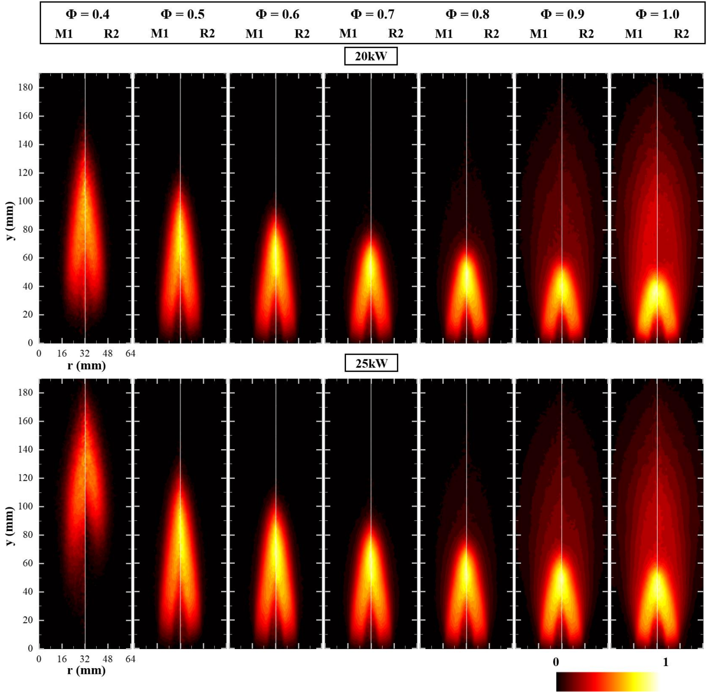
FIGURE 8: ABEL TRANSFORMED OH* CHEMILUMINESCENCE IMAGES FOR 20 KW [TOP] AND 25 KW [BOTTOM] THERMAL POWERS OVER A RANGE OF \Phi . COLORMAP NORMALIZED TO MAXIMUM OH* INTENSITY IN EACH HALF IMAGE. M1 RESULTS SHOWN ON THE LEFT AND R2 RESULTS SHOWN ON THE RIGHT FOR EACH CONDITION.
