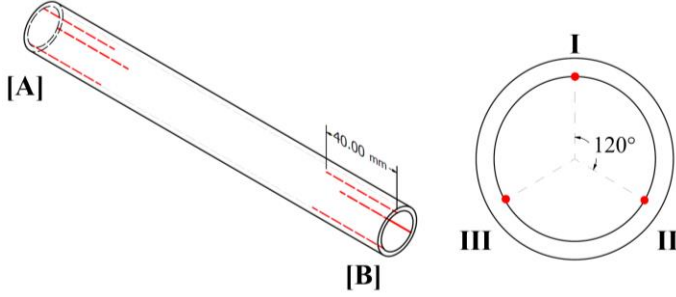
FIGURE 4: SURFACE ROUGHNESS MEASUREMENT LOCATIONS ON M1 AND R2 INSERTS.
