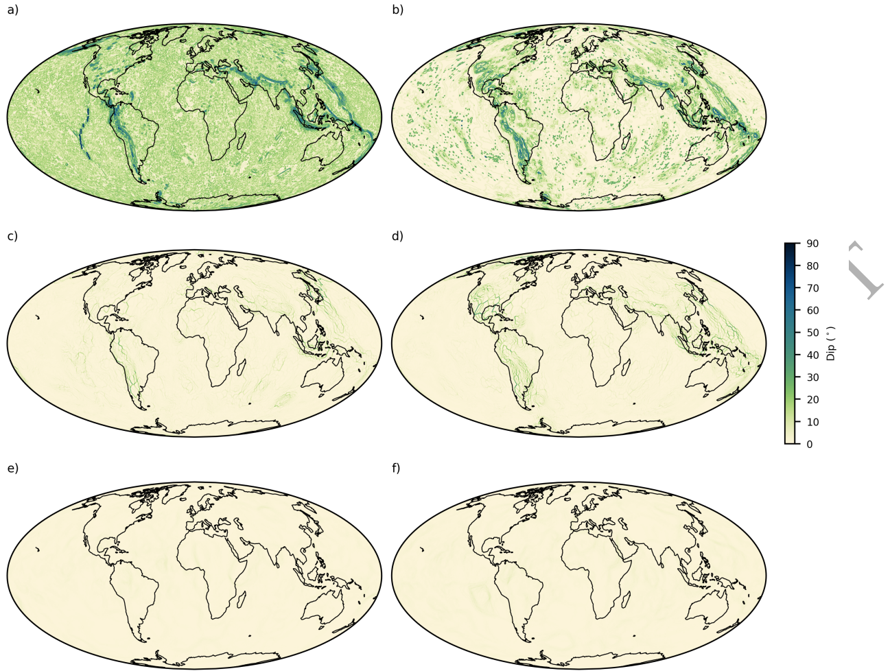
Figure 6. Dip of surface of (a, c, & e) d410 and (b, d, & f) d660 for unfiltered predicted topography (TC3MM) (a & b), filtered (500 km radius bouncepoint spherical cap) predicted topography (c & d), Waszek et al. (2021b) topography model (e & f)
