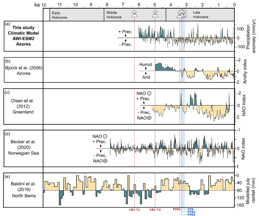
Figure 3. Paleoclimate reconstructions for the North Atlantic over the Holocene. (a) Simulated mean annual precipitation at the Azores obtained from the global climate model AWI-ESM2 (Table S4, https://doi.org/10.5281/zenodo.17079274 ), (b) aridity index reconstructed using lake sediments from Pico Island, Azores (Björck et al., 2006), (c) NAO index reconstructed using a lake sediment record from southwestern Greenland (Olsen et al., 2012), (d) NAO index reconstruction based on southeastern Norwegian Sea sediment cores (Becker et al., 2020), and (e) precipitation variability based on North Iberian speleothems (Baldini et al., 2019). Red (magmatic) and blue (phreatomagmatic) lines mark the timing of Flores' Holocene eruptions.
