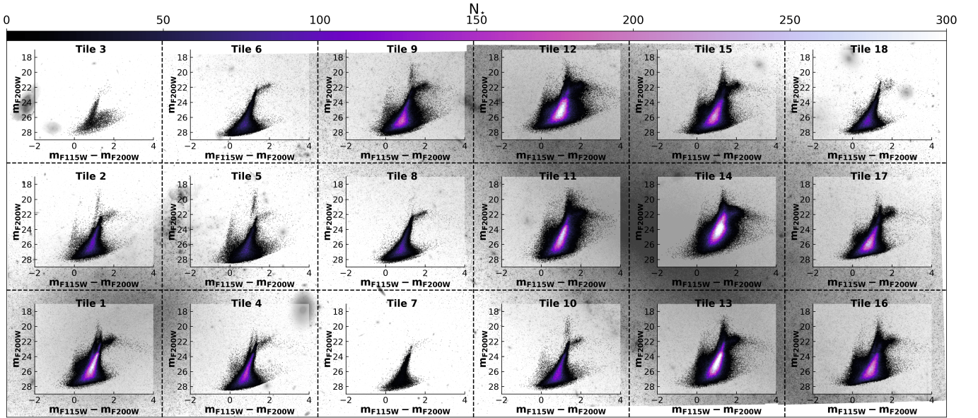
Figure 4. m_{F200W} vs. m_{F115W} - m_{F200W} CMDs for each tile, displayed on top of the F200 W reference image of the NGC 4485/NGC 4490 system. The high-density regions of the CMDs have been binned and color coded according to the number of stars in each bin (see colorbar on the top).
