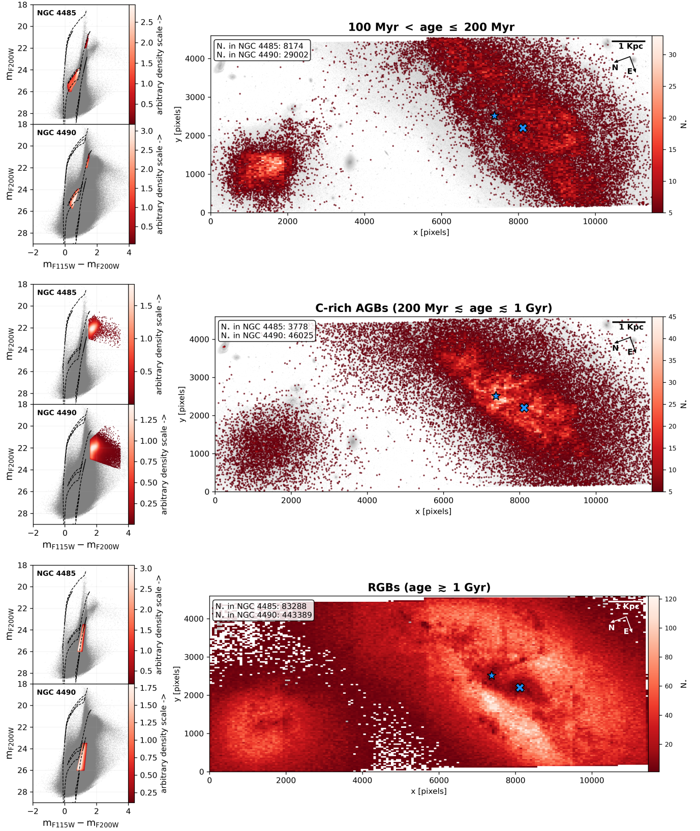
Figure 10. Same as Figure 9, but for selected bona-fide stars with ages between \sim 100 Myr and \sim 200 Myr, intermediate age C-rich AGBs between 200 Myr and 1 Gyr, and RGB stars older than 1 Gyr.
