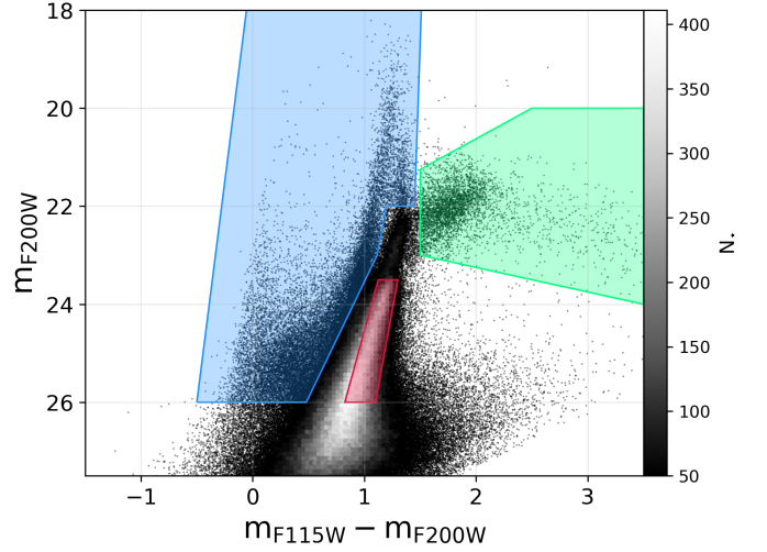
Figure 8. CMD of NGC 4485 (i.e., tile 1, 2, 3, 4, and 5) showing our selection of three different stellar populations, tracing different epochs in the life of the galaxy. MS, BL, RSG, and O-rich AGB stars younger than 200 Myr in blue. C-rich AGBs between \sim 200 Myr and \sim 1 Gyr in green, and RGB stars older than \sim 1 Gyr, and potentially as old as \sim 13 Gyr, in red.
