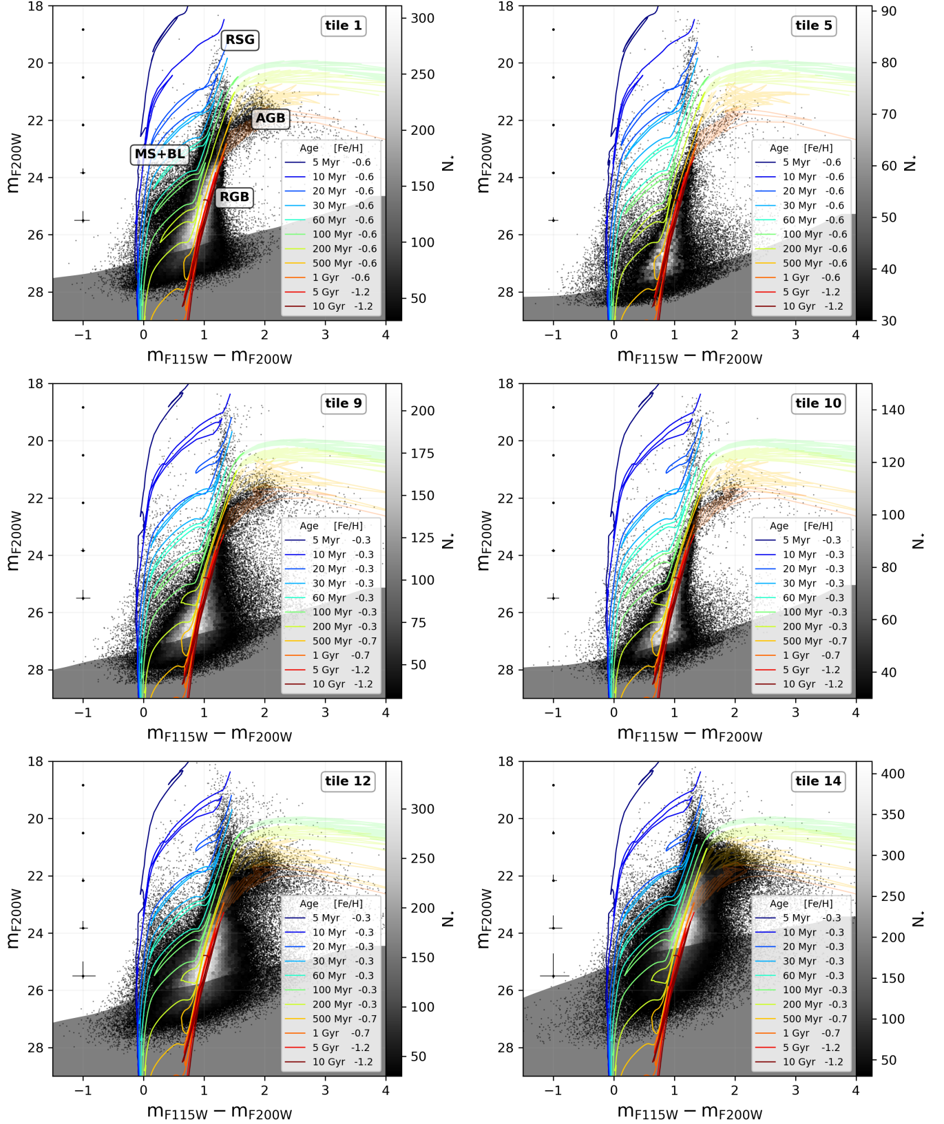
Figure 6. CMDs of tile 1, 5, 9, 10, 12, and 14 covering different regions of both NGC 4485 and NGC 4490. Each CMD is binned and color coded according to the density of stars. Different sets of PARSEC-COLIBRI isochrones are also plotted, assuming a distance modulus of (m - M)_0 = 29.70 and a reddening of E(B - V) = 0.15 , color-coded according to age and metallicity (see legend on the bottom right of each panel). The TPAGB phase is shown with a lower \alpha value. Photometric errors estimated from ASTs are shown on the left-hand side. The shaded area marks the 50% completeness limit. Some of the stellar evolutionary phases mentioned in the text are labeled in tile 1 CMD.
