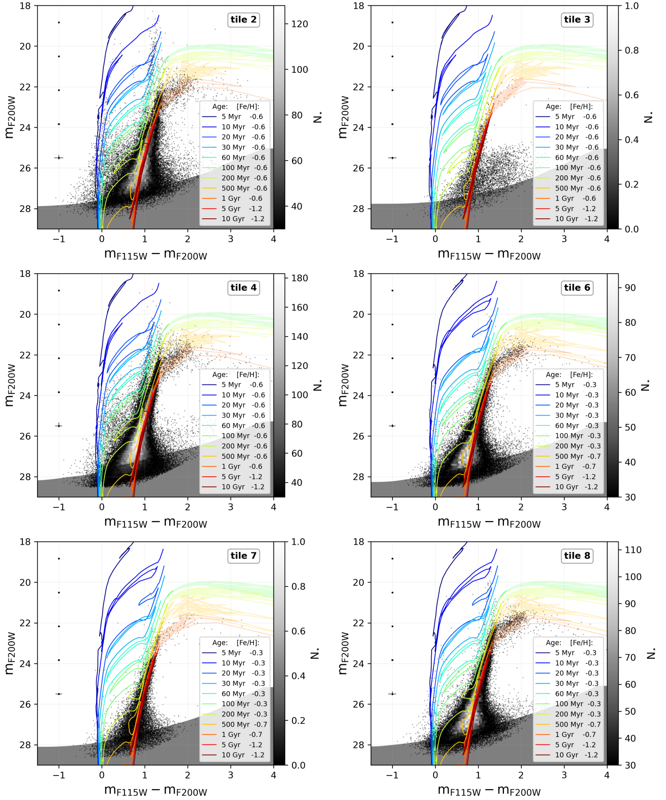
Figure 12. CMDs of tile 2, 3, 4, 6, 7, and 8. See Figure 6.
