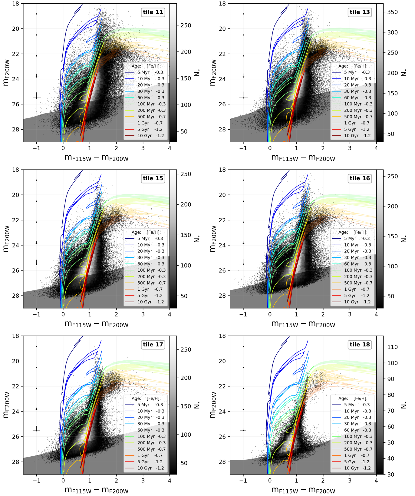
Figure 13. CMDs of tile 11, 13, 15, 16, 17, and 18. See Figure 6.
