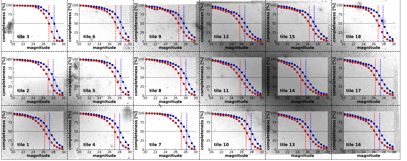
Figure 3. NIRC Cam ’s F200 W image, with superimposed for each tile the completeness of the photometry as a function of magnitude, derived from our ASTs, in both the F115 W (blue) and F200 W (red) filters. The 50% completeness level is marked by the dashed-gray line, while the magnitude at which this limit is reached in each filter is marked by the dashed-vertical lines.
