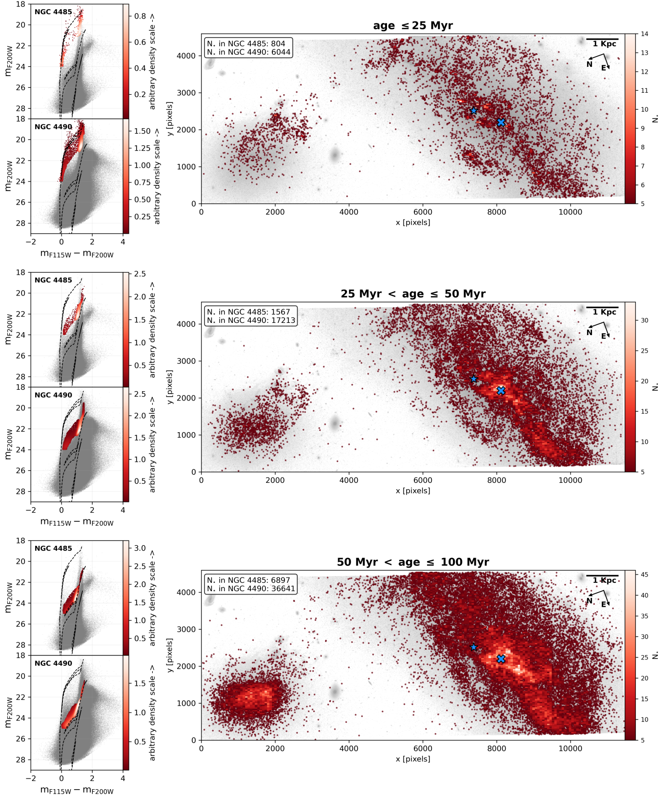
Figure 9. CMDs and spatial distributions of NGC 4485/NGC 4490 stars in different age intervals: age \leq 25 Myr, 25 Myr < age \leq 50 Myr, and 50 Myr < age \leq 100 Myr. Left panels: NGC 4485 (upper panel) and NGC 4490 (lower panel) CMDs, with the stars in the selected age intervals marked in red, and with the PARSEC-COLIBRI 10 Myr, 100 Myr, and 1 Gyr isochrones in dashed-black lines. Right panels: Spatial distribution of the stars in the selected age intervals, overlaid on the F200W reference image. In the high-density regions, the data are binned and color coded according to the number of points (see the color-bar on the right hand-side of each panel). The cross and star symbols mark the position of the optical and infrared nuclei, as reported by Lawrence et al. (2020). The number of stars in the selected age interval for both NGC 4485 and NGC 4490 is reported in the upper left.
