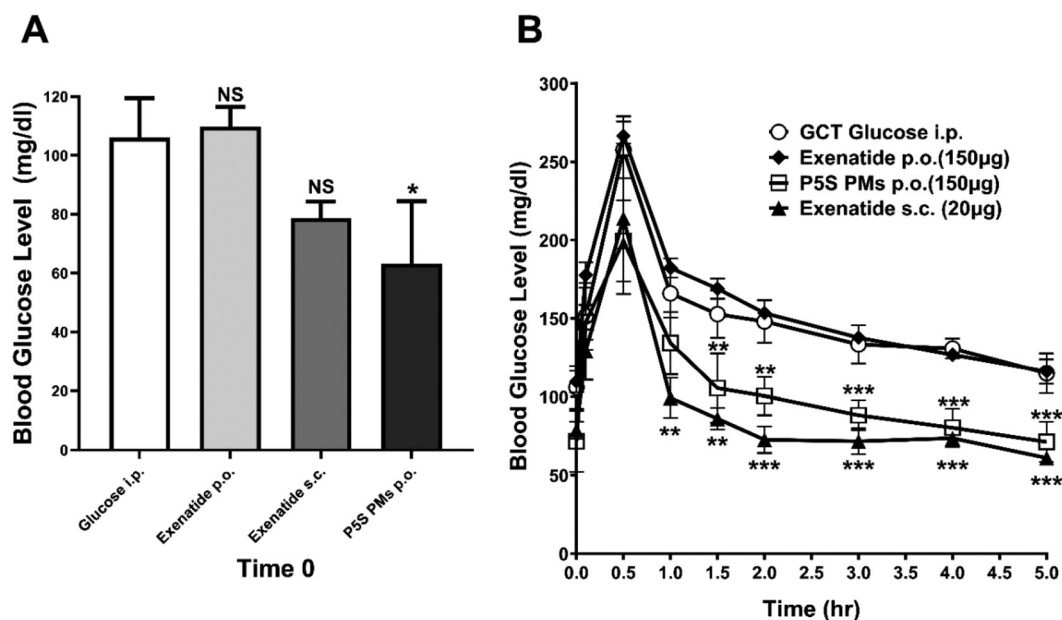
Fig. 8 The PD study based on the measurement of blood glucose levels in response to a glucose challenge test ( i.p. GCT 'no treatment' control). The exenatide treatments always preceded the i.p. glucose (GCT) administrations. For each individual formulation, the time period following exenatide administration prior to the i.p. GCT was optimised so as to correspond to peak (near-peak) exenatide plasma levels at the point of i.p. GCT administration; for s.c. exenatide this was 10 min, while for oral solution exenatide ( Exenatide p.o. ) and for the sulfobetaine polymeric micelles ( P5S PMs p.o. ) this was 4 h. [A] Endogenous glucose levels at time zero immediately before i.p. glucose administration. The orally administered exenatide–sulfobetaine PMs (administered 4 h previously) reduced endogenous blood glucose levels significantly greater than any other treatment arms. [B] Blood glucose levels following the i.p. glucose challenge test for the treatments. Exenatide oral solution ( Exenatide p.o. 150 \mu g) given 4 h before the i.p. GCT showed no effect on the glucose levels. Exenatide delivered orally by P5S sulfobetaine PMs ( P5S PMs p.o. 150 \mu g) showed a significant decrease in glucose levels throughout the 1.5 h to 5 h post-GCT period. Similarly, s.c. exenatide solution ( Exenatide s.c. 20 \mu g) significantly reduced blood glucose levels over the 1 h to 5 h post-GCT period. From 0.5 h to 5 h post-GCT challenge no statistical differences were observed between the glucose levels in the oral exenatide–sulfobetaine PMs and the s.c. exenatide solution administration. Data represent the mean \pm SD ( N = 4 or each glucose time profile). Statistically significant differences were observed (** P < 0.01 ), (***) \leq 0.001 ) when comparing data with those of the glucose challenge test alone (glucose i.p. ).
