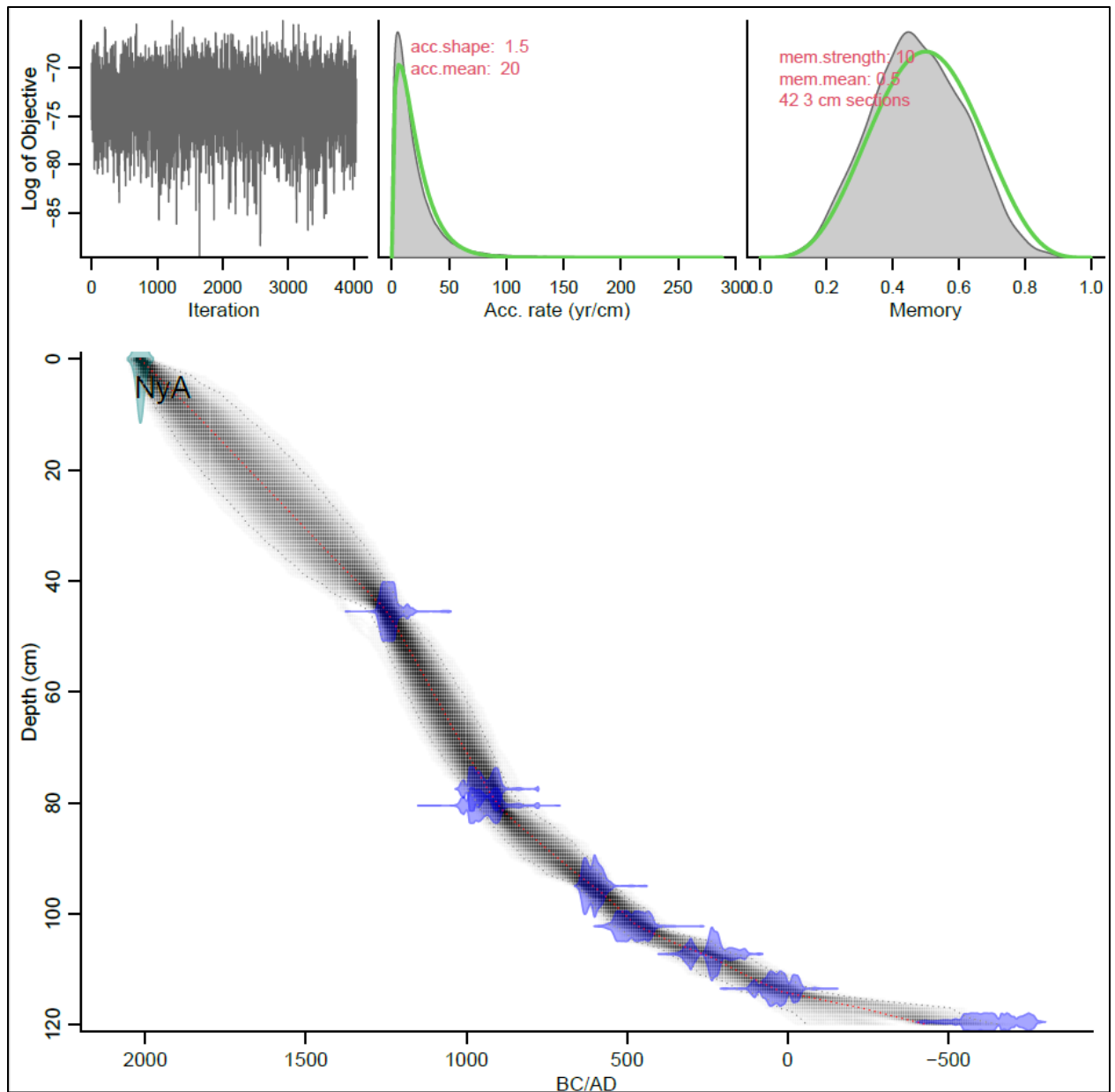
Figure 4: Age-depth model for Nant yr Argae (produced using “Bacon 4.0.5” - Blaauw & Christen 2011) (Figure by Tudur Davies).
