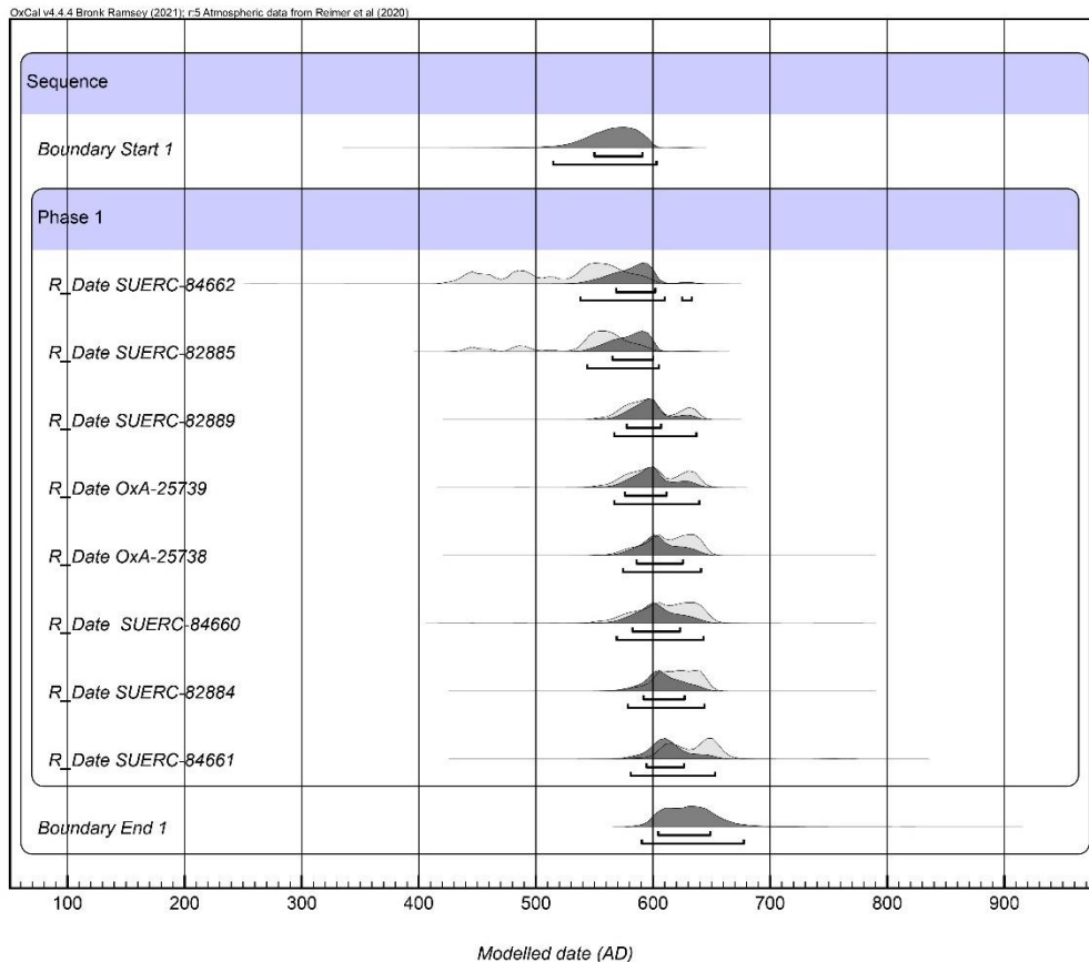
Figure 4: Single-phase model for radiocarbon dates from Dinas Powys (Campbell et al. 2023). Modelled in OxCal 4.4 using the IntCal 20 curve (Bronk Ramsey 2009; Reimer et al. 2020) (Figure by Andy Seaman).
