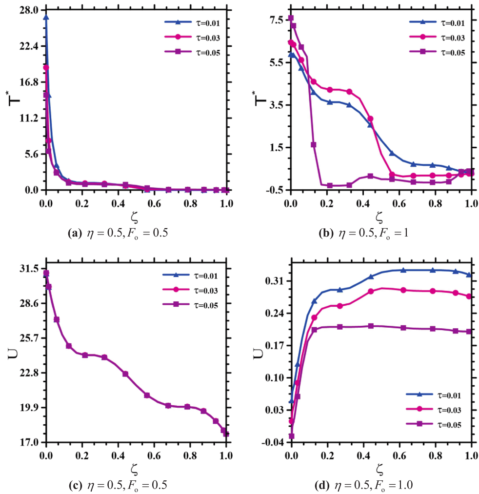
Fig. 13. Effects of the relaxation time on the through-the-thickness variations of the non-dimensional temperature and radial displacement for clamped multilayer truncated conical shell with the GPLRC-FS and GPLRC-PC [ W_{GPL} = 0.3\% , e_0 = 0.4 , porosity type 1, \beta = 15^\circ , u^* = 1 (cm/s)].
