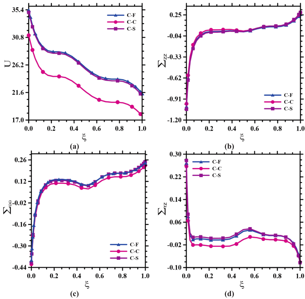
Fig. 19. Effects of the boundary conditions on the through-the-thickness variation of the results of the multilayer truncated conical shell with the GPLRC-FS and GPLRC-PC [ W_{GPL} = 0.3\% , \eta = 0.5 , Fo = 0.5 , e_0 = 0.4 , porosity type 1, \beta = 15^\circ , u^* = 1 (cm/s), \tau = 0.03 ].
