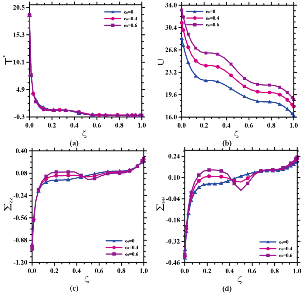
Fig. 9. Effects of porosity amounts on the through-the-thickness variation of the results of the clamped multilayer truncated conical shell with the GPLRC-FS and GPLRC-PC [ W_{GPL} = 0.3\% , \eta = 0.5 , Fo = 0.5 , porosity type 1, \beta = 15^\circ , u^* = 1 (cm/s), \tau = 0.03 ].
