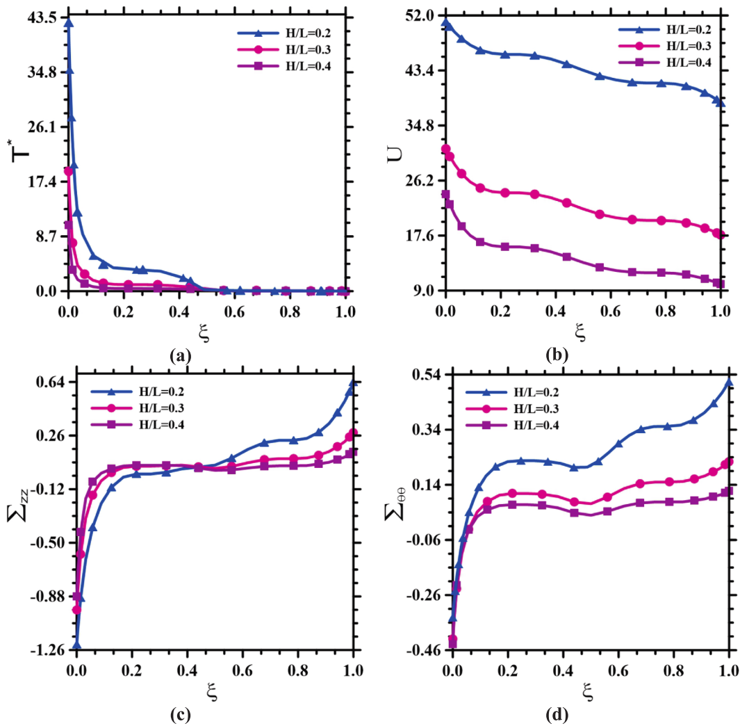
Fig. 16. Effects of the thickness-to-length ratio on the through-the-thickness variation of the results of the clamped multilayer truncated conical shell with the GPLRC-FS and GPLRC-PC [ W_{GPL} = 0.3\% , \eta = 0.5 , Fo = 0.5 , e_0 = 0.4 , porosity type 1, \beta = 15^\circ , u^* = 1 (cm/s), \tau = 0.03 ].
