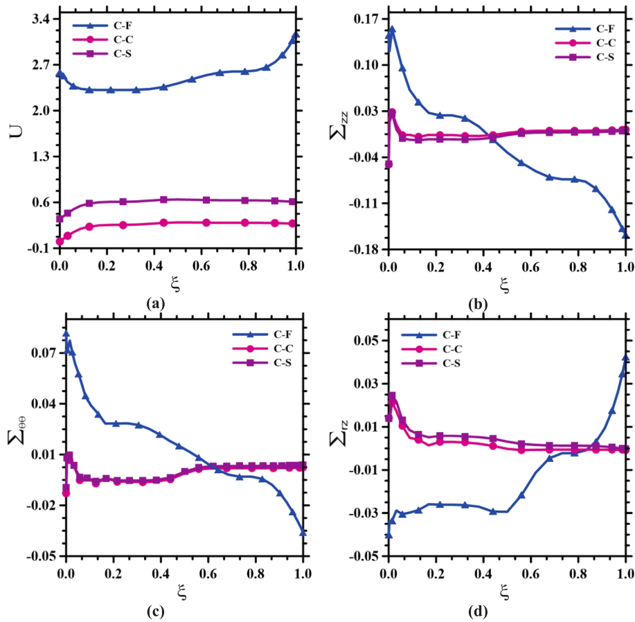
Fig. 18. Effects of the boundary conditions on the through-the-thickness variation of the results of the multilayer truncated conical shell with the GPLRC-FS and GPLRC-PC [ W_{GPL} = 0.3\% , \eta = 0.5 , F_0 = 1 , e_0 = 0.4 , porosity type 1, \beta = 15^\circ , u^* = 1 (cm/s), \tau = 0.03 ].
