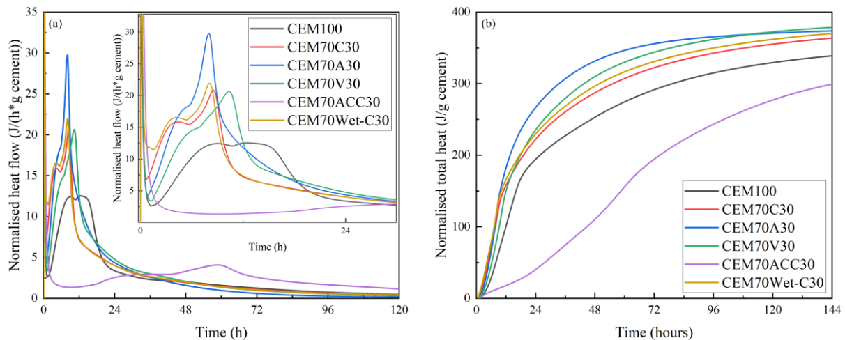
Figure 3: (a) Heat flow and (b) total heat of cement pastes blended with different \text{CaCO}_3
