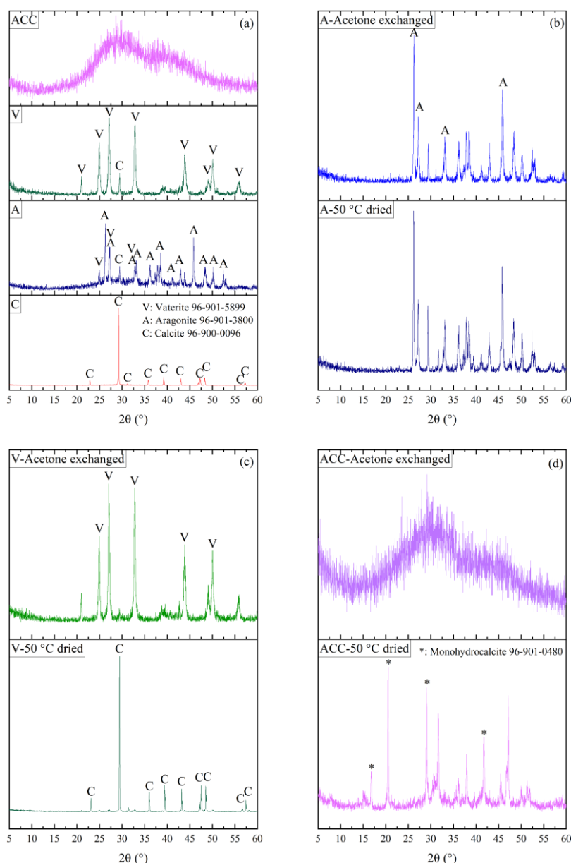
Figure 1: XRD patterns of (a) freshly synthesised samples of different \text{CaCO}_3 , and samples of (b) A, (c) V, and (d) ACC after drying at 50 °C or solvent exchange with acetone
