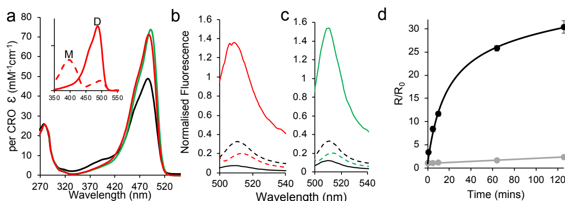
Fig. 2. Dimerisation of sfGFP C148 variants. (a) Absorbance spectra of sfGFP WT (black), dGFP-diS1 (red) and dGFP-diS2 (green). Inset is the change in absorbance on conversion of mGFP-S1 (dashed red line) to dGFP-diS1 (solid red line). The full absorbance spectra are shown in Fig. S2. Emission spectra of (b) GFP-diS1 and (c) GFP-diS2, with red and green representing the dimers, respectively, and black the monomer. Solid and dashed lines represent excitation at either the optimal CRO-B wavelength (490-497nm) or CRO-A wavelength (400 nm), respectively. (d) Rate of dimerisation of GFP-diS1 (grey) and GFP-diS2. The data shown are for 10 \mu\text{M} of starting monomer with R/R_0 representing the change in fluorescence emission ratio on excitation at either 388 nm or 483 nm.
