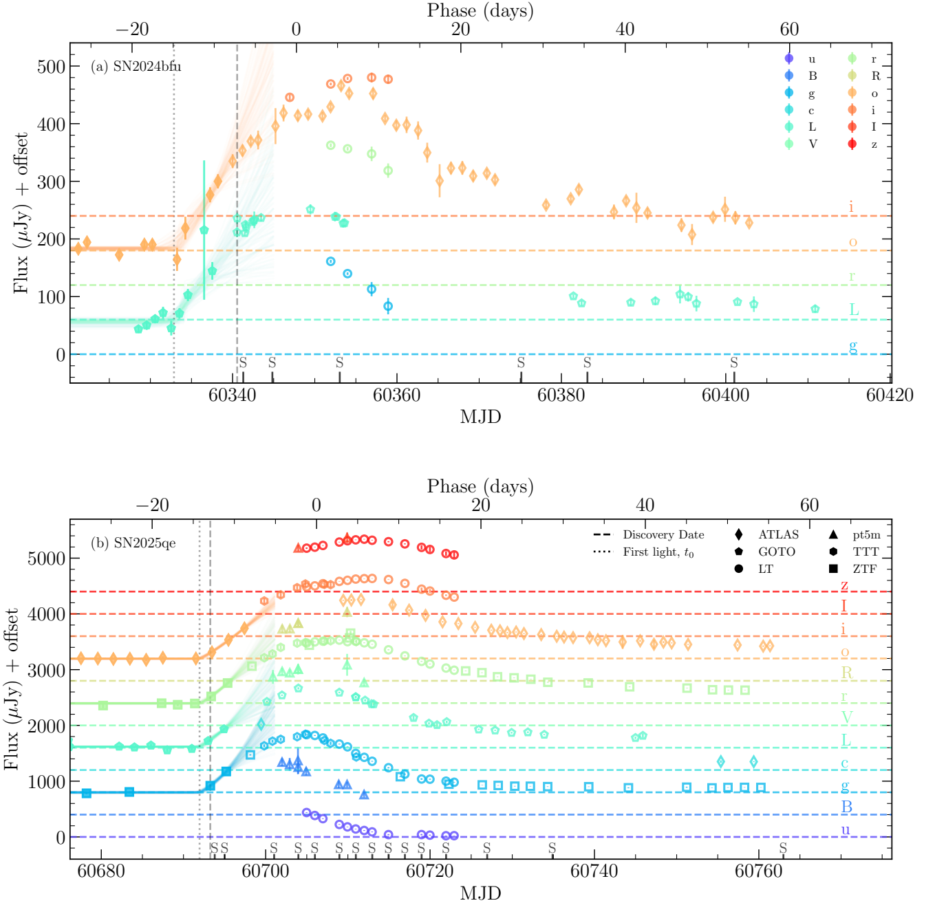
Figure 2. Light curves of SN 2024bfu (Panel a) and SN 2025qe (Panel b). Fits to the observations using Eqn. 1 are shown as coloured lines based on randomly sampled the posterior distributions. Observations included in the fits are shown as filled points, while those not included are shown unfilled. Offsets are applied to each filter for clarity and are given by horizontal lines. Observations from different facilities are denoted by different symbols. The epochs of discovery (dashed) and first light (dotted) are marked as vertical lines. Epochs of spectroscopy are denoted by ‘S’. Phases are given relative to the GOTO L -band maximum.
