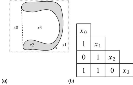
Fig. 2. (a) Using virtual components to represent semi-bounded components in space. (b) Adjacency matrix for the shape in (a).
