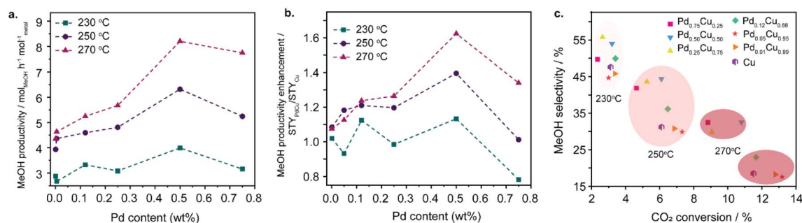
Fig. 3 Performance of PdCu/ZnO catalysts with a variety of Pd : Cu molar ratios and fixed total loadings of 1 wt%. (a) MeOH productivity; (b) enhancement in MeOH productivity for Pd x Cu y catalysts vs. monometallic Cu; (c) MeOH selectivity vs. \text{CO}_2 conversion.
