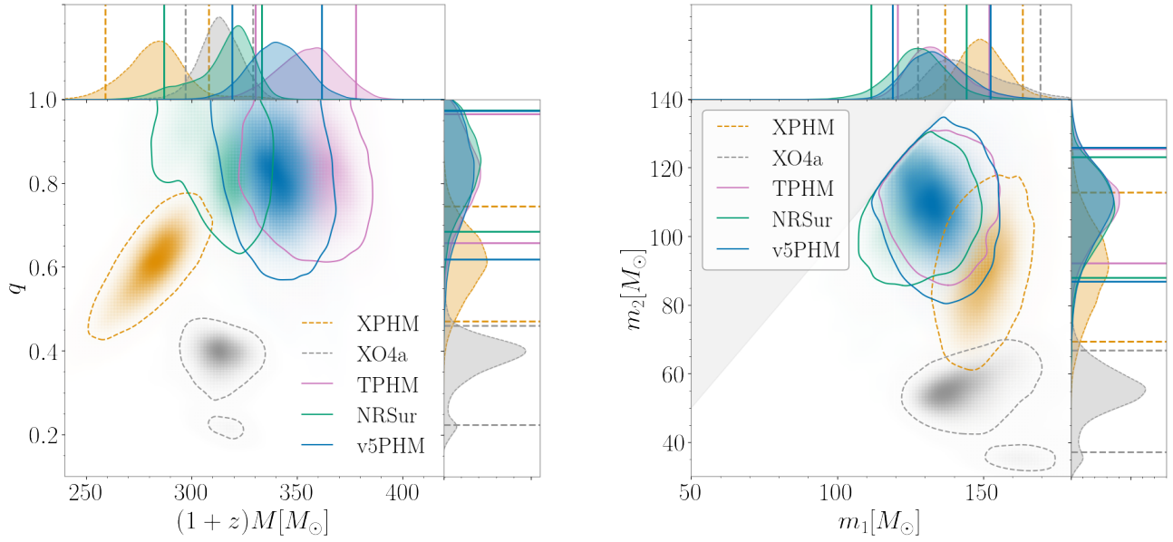
Figure 7. Marginalized posterior probability for (left) the redshifted (detector-frame) total binary mass and mass ratio and (right) the primary and secondary source-frame masses, inferred from GW231123 for each of the five models considered. Each contour, as well as the colored horizontal and vertical lines, shows the 90% credible intervals.
