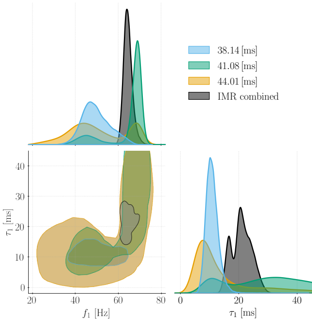
Figure 5. 2D frequency and damping time posterior distribution (90% credible levels), when starting the analysis at late times and assuming a single damped sinusoid with positive frequency; the combined IMR estimates for the longest-lived \ell mn = 220 QNM are shown for comparison. For visualization purposes, we display up to \tau_1 = 45 ms, while the posterior tail extends up to \tau_1 = 80 ms.
