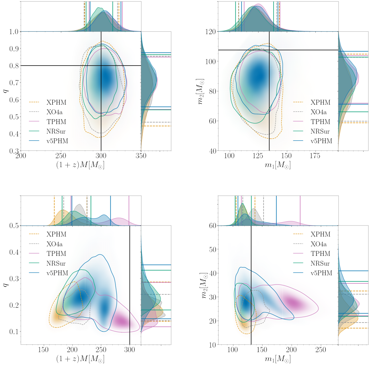
Figure 8. Marginalized posterior probability for (left column) the redshifted (detector-frame) total binary mass and mass ratio and (right column) the primary and secondary source-frame masses, inferred from two highly spinning precessing NR simulations with (detector-frame) total binary mass of 300 M_{\odot} , observed approximately edge on. The top row shows the results for SXS:BBH:0483 (M. Boyle et al. 2019), with masses m_1 \sim 135 M_{\odot} , m_2 \sim 110 M_{\odot} , and mass ratio q = 0.8 . The bottom row shows the results for SXS:BBH:4030 (M. A. Scheel et al. 2025), with masses m_1 = m_2 \sim 130 M_{\odot} . The five models used to analyze GW231123 were also used to analyze these simulations. Each contour, as well as the colored horizontal and vertical lines, shows the 90% credible intervals. The black vertical and horizontal lines indicate the true source properties. In some panels, the true value is beyond the axis range of the figure.
