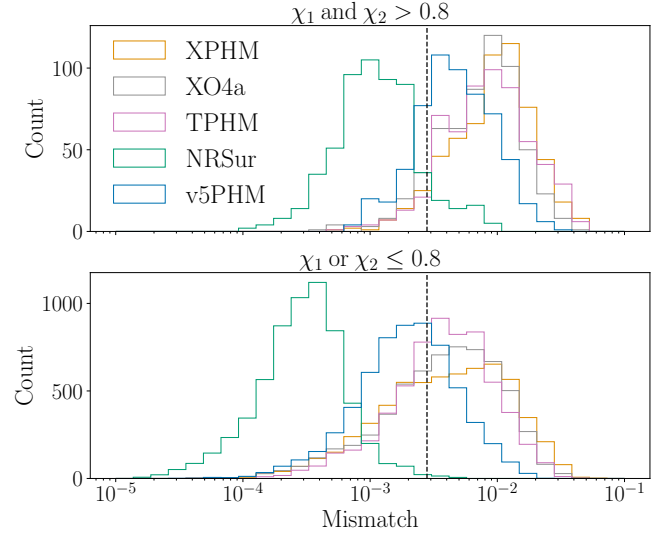
Figure 2. Mismatch accuracy of the waveform models considered in this Letter against 1123 NR simulations at a total mass of 300 M_\odot and a range of inclinations between \iota = 0 and \pi/2 . The vertical dashed line at a mismatch of 0.0028 shows the conservative criterion discussed in the text.
