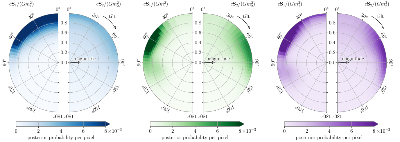
Figure 9. Posterior probabilities for the dimensionless component spins cS_1/(Gm_1^2) and cS_2/(Gm_2^2) , relative to the orbital angular momentum axis \hat{L} . From left to right, we compare the posterior probabilities obtained when analyzing LIGO Hanford data only (blue), LIGO Livingston data only (green), and a coherent analysis of LIGO Hanford and LIGO Livingston data (purple). In all cases, we show the posterior distribution resulting from equally combining samples from the five waveform models. The tilt angles are 0^\circ for spins that are aligned with the orbital angular momentum and 180^\circ for spins that are antialigned. Probabilities are marginalized over the azimuthal angles. The pixels have equal prior probability, being equally spaced over the spin magnitudes and the cosines of the tilt angles. The spin orientations are defined at a fiducial GW frequency of 10 Hz.
