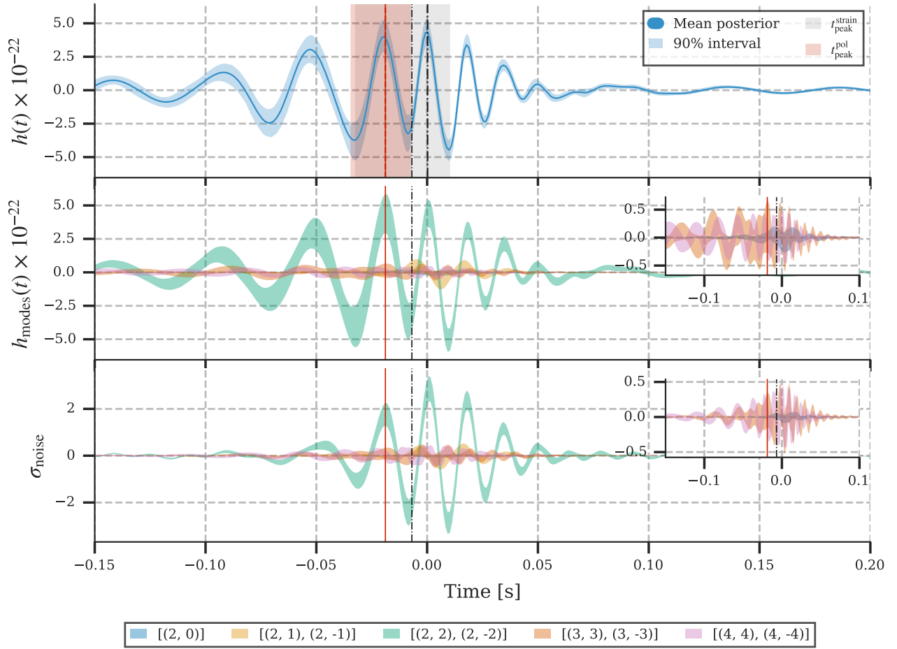
Figure 10. Top: posterior probability density functions of the NRSUR waveform time series, obtained via BILBY using the NRSUR waveform model at the LIGO Hanford detector. The red band shows the uncertainty in the measurement of t_{\text{peak}}^{\text{pol}} , and the gray band shows the uncertainty in t_{\text{peak}}^{\text{strain}} . Middle and bottom: posterior probability density functions of the mode strain, F_+h_+ + F_\times h_\times , with h_+ - ih_\times = -^2Y_{\ell,m}h_{\ell,m} + ^{-2}Y_{\ell,-m}h_{\ell,-m} , shown for the LIGO Hanford detector. The top part reports the unwhitened waveform, and the bottom part reports the whitened one, showcasing the impact of whitening in visualizing the signal morphology. The inset focuses on the (\ell, \pm m) = (2, 0), (3, 3), (4, 4) modes. The red line indicates the median of t_{\text{peak}}^{\text{pol}} , and the dashed-dotted black lines show the median of t_{\text{peak}}^{\text{modes}} .
