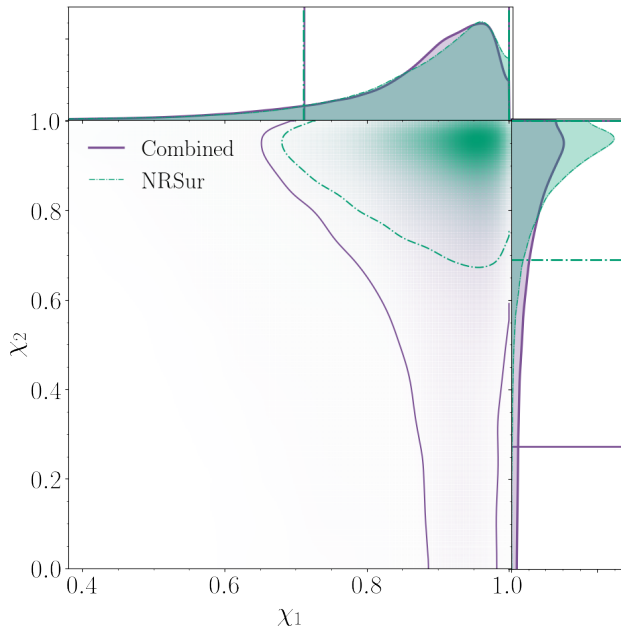
Figure 4. The posterior distribution of the primary and secondary spin magnitudes. We show the posterior distribution based on the combined samples (purple line) and from the NRSUR model (green dashed–dotted line). Each contour, as well as the colored horizontal and vertical lines, shows the 90% credible intervals.
