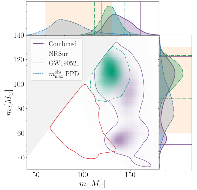
Figure 3. The posterior distribution of the primary and secondary source masses. We show the posterior distribution resulting from equally combining samples from five waveform models that include precession and higher-order multipoles (purple line). We separately show the posterior distribution obtained with NRSUR (green dashed-dotted line). We compare against estimates for the source-frame masses of GW190521 (red solid line; R. Abbott et al. 2020b, 2020c, 2023a). Each contour, as well as the colored horizontal and vertical lines, shows the 90% credible intervals. With the blue dashed line, we show the posterior predictive distribution for the largest BH mass m_{\text{max}}^{\text{obs}} in mock catalogs similar to GWTC-3 (R. Abbott et al. 2023a, 2023b)—see Section 6. The solid orange bands show the putative mass gap from (pulsational) PI from 60–130 M_\odot .
