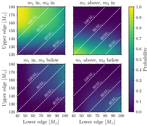
Figure 6. Probabilities using the combined parameter estimates for GW231123 that: both BHs are in the PI mass gap (top left); the primary is above the gap and the secondary is in it (top right); the primary is in it and the secondary is below (bottom left); and the primary is above and the secondary is below (bottom right). The probabilities are computed by varying the lower and upper edges of the gap, while the dashed lines mark constant gap widths.
