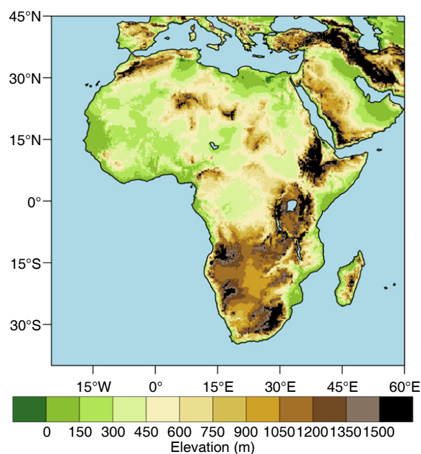
Fig. 1. Topography (elevation in meters) over Africa, derived from ETOPO1 data.
