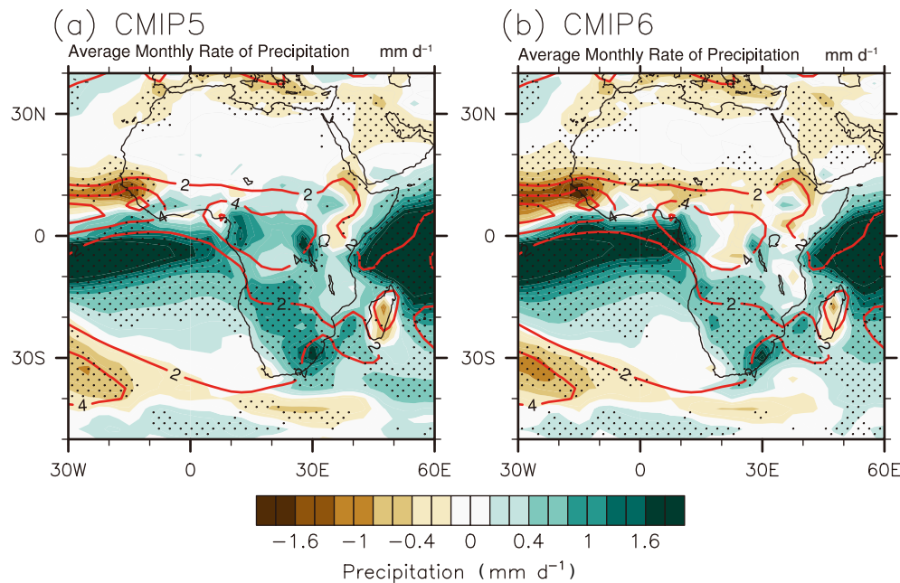
Fig. 2. Bias in annual mean precipitation ( \text{mm d}^{-1} ) for the (a) CMIP5 and (b) CMIP6 ensemble mean, relative to GPCC, over the period 1979–99. Stippling indicates that at least 70% of the models agree on the sign of the multi-model mean bias in precipitation. The red contours show the historical annual mean precipitation, averaged over the period 1960–99; 29 (41) CMIP5 (CMIP6) models were used.
