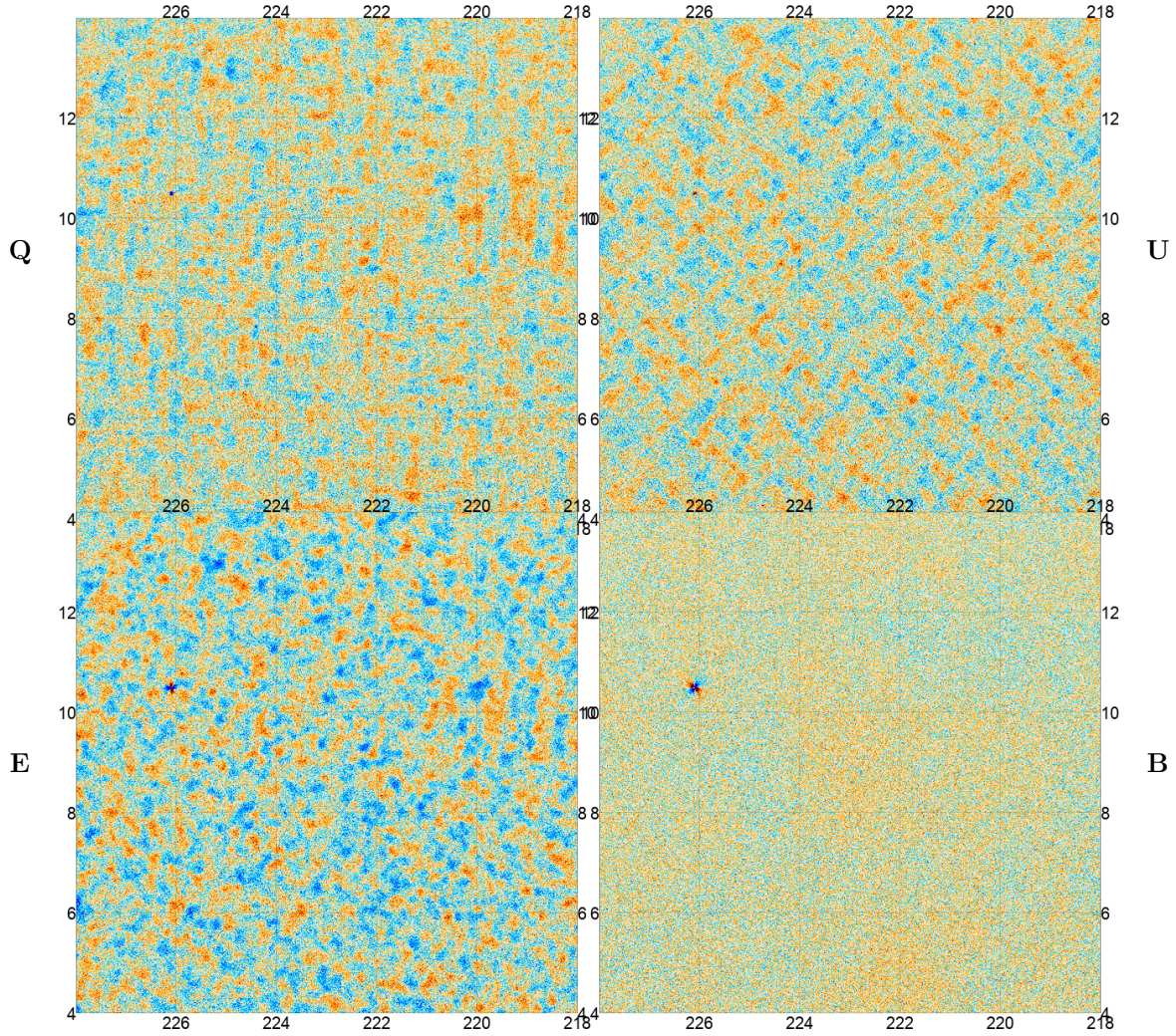
Figure 9. The same area as in figure 8, but this time showing f090+f150 polarization with a \pm 30\mu\text{K} color scale. As shown in figure 5 the white noise level is around 4\mu\text{K} arcmin in this area. Top: The Stokes Q and U parameters. We recognize the + pattern in Q and \times pattern in U characteristic of E-modes. Bottom: E and B polarization maps. The E-modes are signal-dominated while the B-modes are visually indistinguishable from our noise, except for a polarized point source. (The point source appears as a small quadrupole in E and B due to the non-local relationship between Q,U and E,B.).
