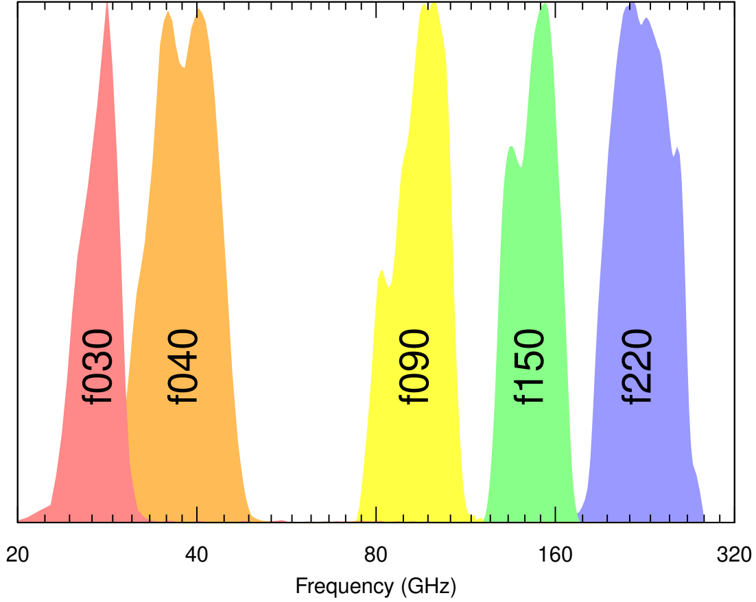
Figure 3. AdvancedACT’s five bandpasses normalized to a peak of 1. DR6 is based on f090, f150 and f220. We postpone the lowest two bands, which were installed in 2020, for future work.
