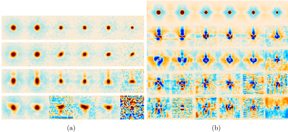
Figure 25. a: Example of four different beam-shapes seen among thousands of day-time observations. The top is the best case, equivalent to the night-time beam. The other represent increasingly pathological behavior. From left to right we have PA5 f090, PA6 f090, PA4 f150, PA5 f150, PA6 f150 and PA4 f220. b: While we have thousands of day-time beam examples, there aren't thousands of different ways for the beam to vary in practice. Most of the beam variability can be explained with just the top five eigenmodes, which are shown here for the same arrays as in a . The eigenmodes are sorted from the strongest (top) to the weakest (bottom).
