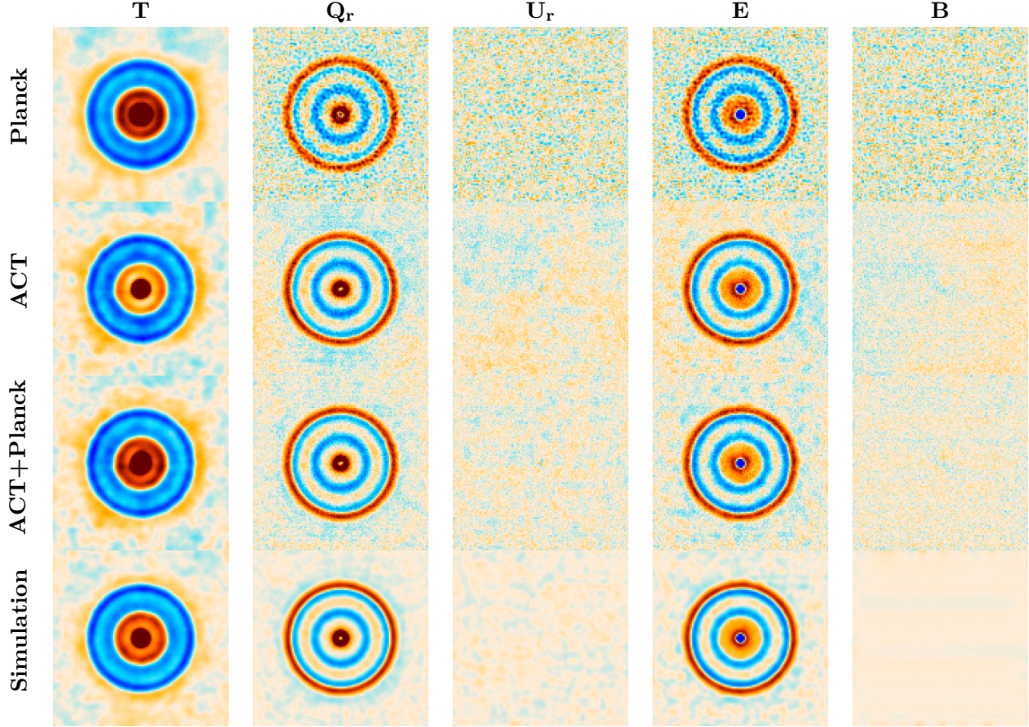
Figure 10. 4\text{ deg} \times 4\text{ deg} stacks of T , Q_r , U_r , E and B on peaks in T for Planck SMICA (row 1), an ACT night-only coadd map (row 2), an ACT+Planck day+night coadd map (row 3), and a beam-less, noise-less simulation (row 4). These stacks are closely related to the CMB autocorrelation function, and give a simple way to illustrate the causal structure of the surface of last scattering. The outermost circle at 1.2\text{ deg} represents the autocorrelation of the 0.6\text{ deg} sound horizon at the surface of last scattering. The images are normalized to give the outer ring an amplitude of 1 ( U_r and B where there is no ring use the same normalization as Q_r and E respectively). Peak detection was done separately for each map, and beam deconvolution was performed. See appendix H for details on the peak detection and stacking procedure.
