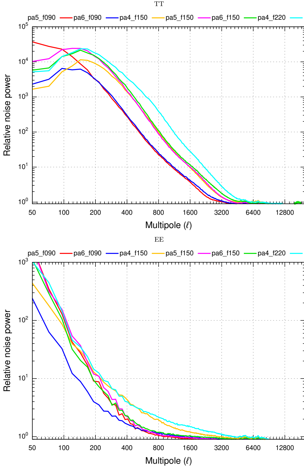
Figure 15. TT and EE noise spectra (not beam-deconvolved) measured from the act_dr6_night data set as the median over the area with -40^\circ < \text{RA} < 60^\circ for the different detector arrays. The power is measured relative to each array’s white noise floor. The turn-around in the TT spectrum for \ell \approx 150 is due to the transfer function, which was not deconvolved here. See section 5.2 for details.
