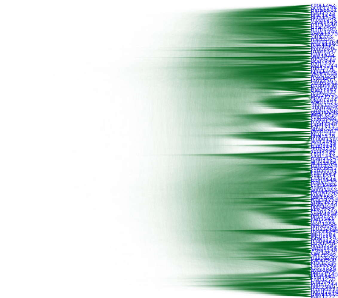
Figure 4. A densitree of the posterior distribution.
