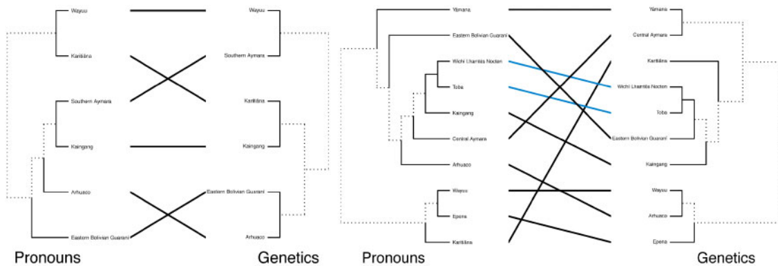
Figure 12. Comparison between the tree derived from pronouns and trees derived from genetic data. Left: Pemberton et al. (2013); right: Reich et al. (2012).
