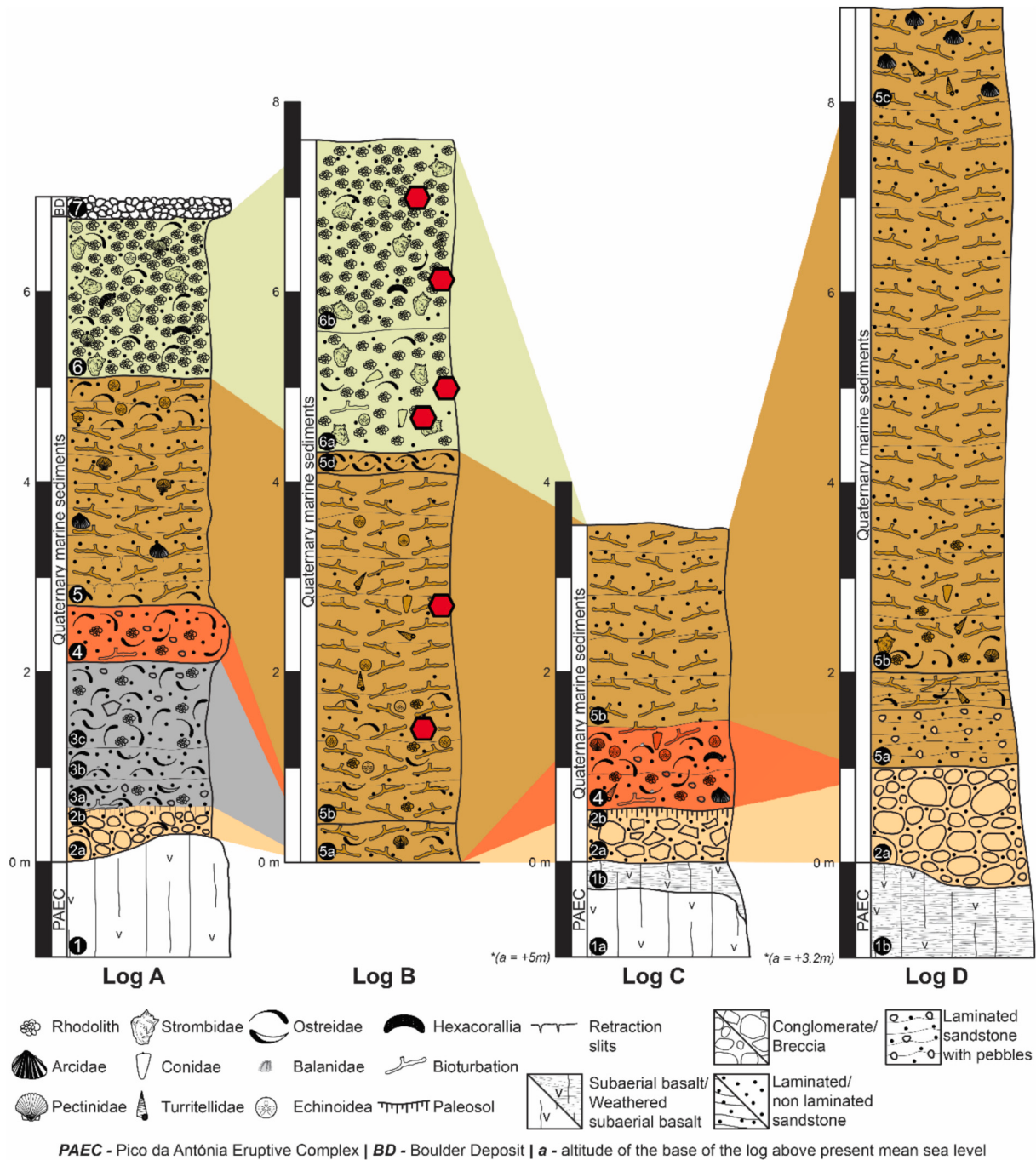
Fig. 2. Stratigraphic logs from Nossa Senhora da Luz Bay fossiliferous sections, with correlation between them. Red hexagons indicate the position where samples for nannofossil analysis were collected. PAEC – Pico da Antónia Eruptive Complex; BD – Boulder Deposit. Geological units are in accordance with the geological map of Santiago Island (Serralheiro, 1976). The sedimentological analysis was performed on five samples that were collected from layers 2a, 3a, 3b, 3c and 4, across log A. (For interpretation of the references to colour in this figure legend, the reader is referred to the web version of this article.)
