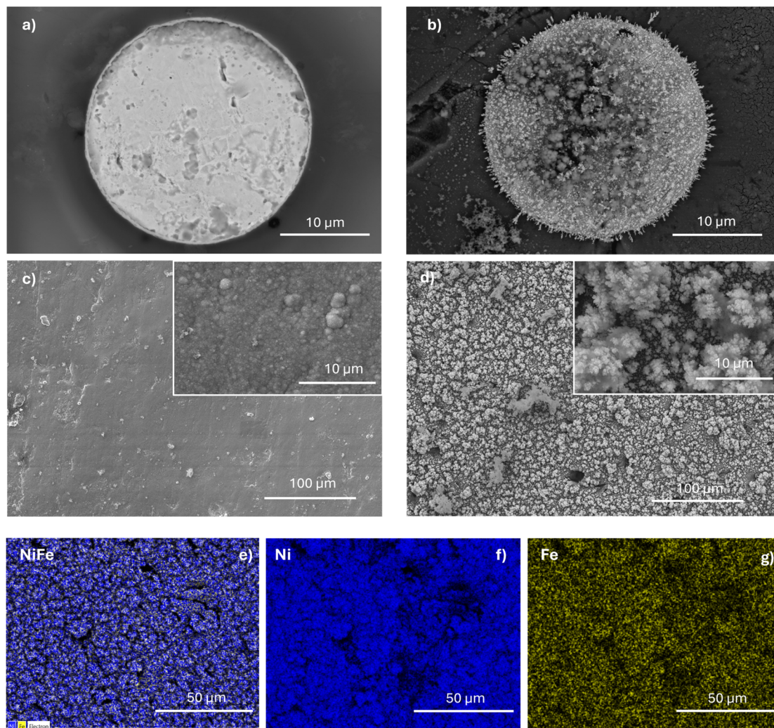
Fig. 1 (a) SEM image of polished uncoated/pristine nickel microelectrode. SEM images of varied electrodeposition capacities within 18 mM metal sulphate & 25 mM ammonium sulphate (b) SEM image of \text{NiFe}(\text{OH})_2 coated Pt microelectrode, using 250 \text{ mA cm}^{-2} for 50 seconds under low vacuum of SEM chamber to avoid charging effects (c) high vacuum SEM image of 2.5 \text{ mA cm}^{-2} for 5000 seconds on Ni foil, 1 \text{ cm}^2 surface area (d) high vacuum SEM image of 25 \text{ mA cm}^{-2} for 500 seconds on Ni foil, 1 \text{ cm}^2 surface area (e) EDS map of \text{NiFe}(\text{OH})_2 catalyst synthesised using 25 \text{ mA cm}^{-2} for 500 seconds on polished carbon plate, both Ni and iron overlaid showing distribution (f) Ni distribution (g) Fe distribution.
