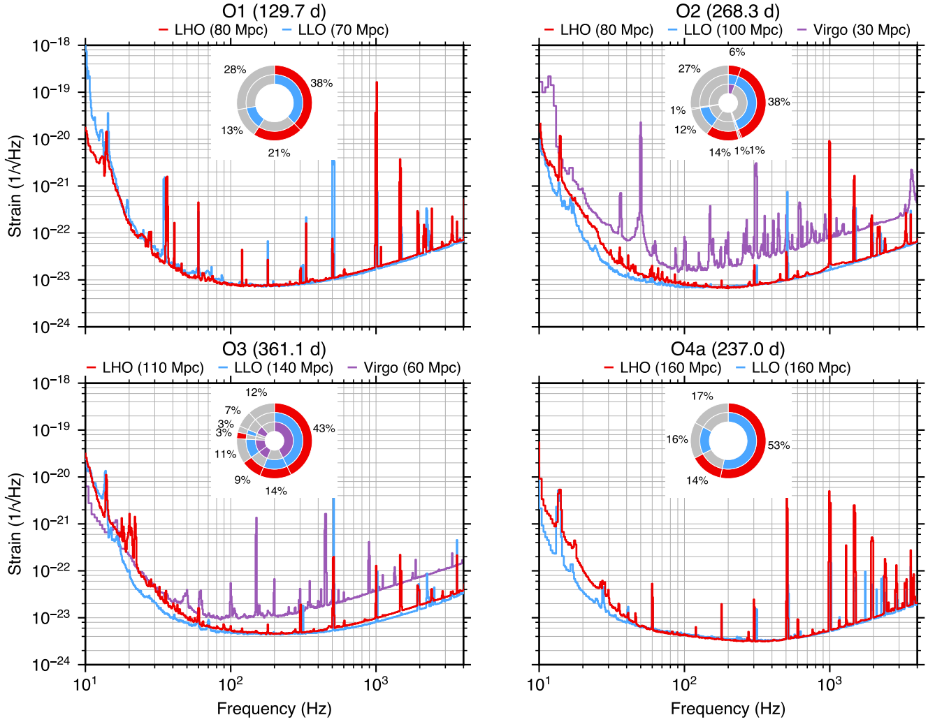
Figure 2. Representative noise amplitude spectral densities for LHO, LLO, and Virgo during O1 (LHO, LLO: 2015 October 24), O2 (LHO: 2017 June 10; LLO: 2017 August 6; Virgo: from F. Acernese et al. 2023a), O3 (LHO: 2020 January 4; LLO: 2019 April 29; Virgo: 2020 February 9), and O4a (LHO: 2024 January 11; LLO: 2023 November 19). The BNS inspiral ranges, defined by Equation (1), for these noise curves are given in the legend. Inset sunburst charts show the fraction of the run duration during which different combinations of detectors were observing. Gray regions in each ring indicate portions when a detector is not operating. The segments of the sunburst chart, clockwise from 12 o'clock, are LHO-LLO, LHO alone, LLO alone, and neither for observing runs involving only LHO and LLO; and LHO-LLO-Virgo, LHO-LLO, LHO-Virgo, LLO-Virgo, LHO alone, LLO alone, Virgo alone, and none for observing runs involving LHO, LLO, and Virgo.
