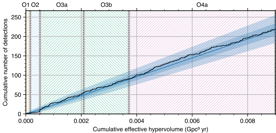
Figure 3. The number of CBC detection candidates with a probability of astrophysical origin greater than or equal to 50% vs. the detector network’s effective surveyed hypervolume for BNS coalescences (R. Abbott et al. 2021b). The BNS effective surveyed hypervolume is a valid proxy for overall sensitivity to CBCs, though its scale is set to the case of canonical BNS signals. The colored bands indicate the different observing runs. The final data sets for O1, O2, O3a, O3b, and O4a consist of 49.0 day, 122.2 day, 149.6 day (177.1 day), 124.6 day (141.9 day) and 126.5 (196.8) days, respectively, with at least two detectors (one detector) observing. The cumulative number of probable candidates is indicated by the solid black line, while the blue line, dark-blue band, and light-blue band are the median, 50% confidence interval, and 90% confidence interval for a Poisson distribution fit to the number of candidates at the end of O4a, respectively.
