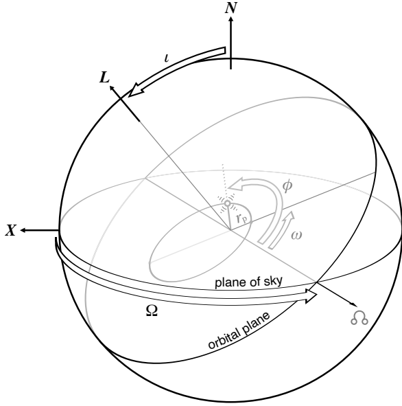
Figure 5. Relationship between the orbital elements and the GW coordinate frame. The direction from the source to Earth is N , and the vector X defines a reference direction on the transverse plane (the plane of the sky). The inclination \iota is the angle between N and the orbital angular momentum vector L . The longitude of the ascending node of the orbit \Omega is the angle on the plane of the sky between X and the ascending node \mathcal{Q} , N \times L . The angle \Omega is degenerate with the polarization angle \psi . The orbit of the primary about the center of mass of the system is shown. The orbital phase \phi is the angle on the orbital plane between the ascending node and position vector of the primary relative to the center of mass. For an eccentric orbit, the distance of the primary from the center of mass at periastris is r_p , and the argument of the periastris \omega for the primary is the angle on the orbital plane between the ascending node and the position vector of the primary at periastris.
