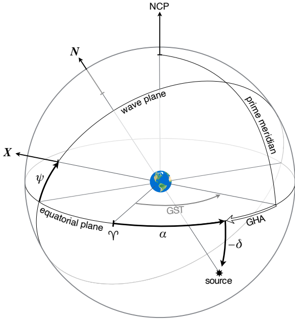
Figure 4. Relationship between the sky location in equatorial coordinates, the polarization angle, and the GW coordinate frame. The direction from the source to Earth is N , and the vector X defines a reference direction on the transverse plane called the wave plane. The location of the source on the sky in the equatorial coordinate system is given by its R.A. \alpha and decl. \delta . The polarization angle \psi is the angle counterclockwise about N between the equatorial plane and X . Also shown is the Greenwich sidereal time (GST), the angle between the first point of Aries \Upsilon and the prime meridian, and the Greenwich hour angle (GHA) of the source, GHA = GST - \alpha . NCP is the north celestial pole.
