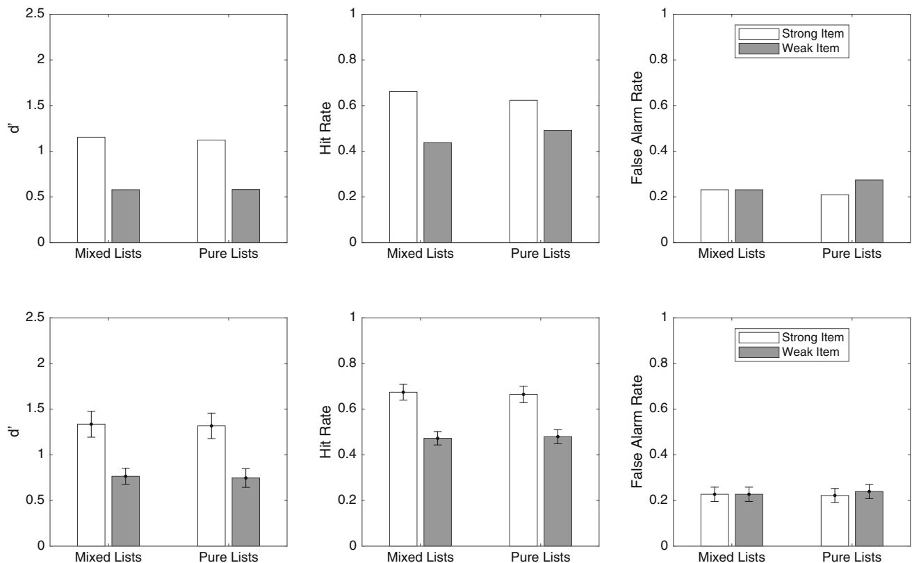
Fig. 11 Model (top) output based on the best-fitting parameters from the parameter explorations (Model variant “ g=0.1 ” in Table 5 to the spaced-repetition data from Experiment 1 (bottom). Parameter values are g = 0.1 , p_e = 0.8 , t_{\text{weak}} = 1 , t_{\text{strong}} = 5 , u^* = 0.04 , c = 0.7 , n = 20 and L = 32
