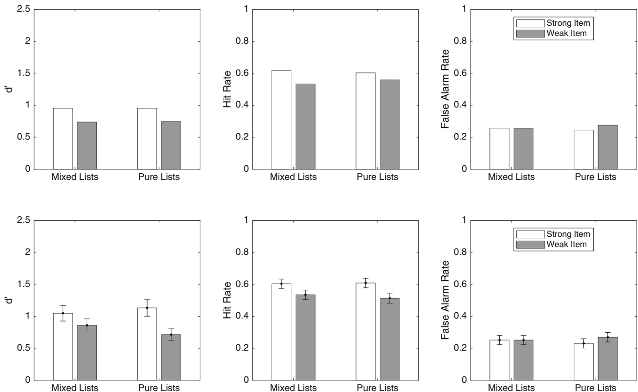
Fig. 10 Model (top) output based on the best-fitting parameters from the parameter explorations (Model variant “ n = 10 ” in Table 4 to the massed-repetition data from Experiment 1 (bottom). Parameter values are g = 0.4 , p_e = 1.0 , t_{\text{weak}} = 7 , t_{\text{strong}} = 10 , u^* = 0.04 , c = 0.7 , n = 10 and L = 32
