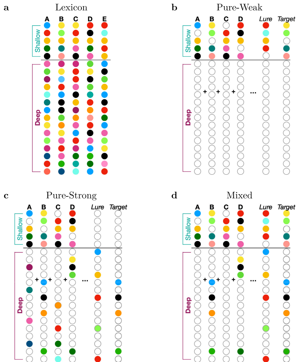
Fig. 1 Attentional subsetting theory schematic. a Example items (A, B, etc.), n -dimensional column vectors. Each circle stands for a vector dimension, and the color (arbitrarily chosen) denotes its value. b In a pure-weak list, only shallow features are stored and processed at test. Grey unfilled circles denote features that are not attended. c In a pure-strong list, shallow and deep features are stored. At test, because deeper features are more diagnostic of items due to their sparseness, we assume participants disregard shallow features in their decision process because the shallow features offer far less evidence of whether or not a word was studied. d In a mixed list, weak and strong items are encoded
