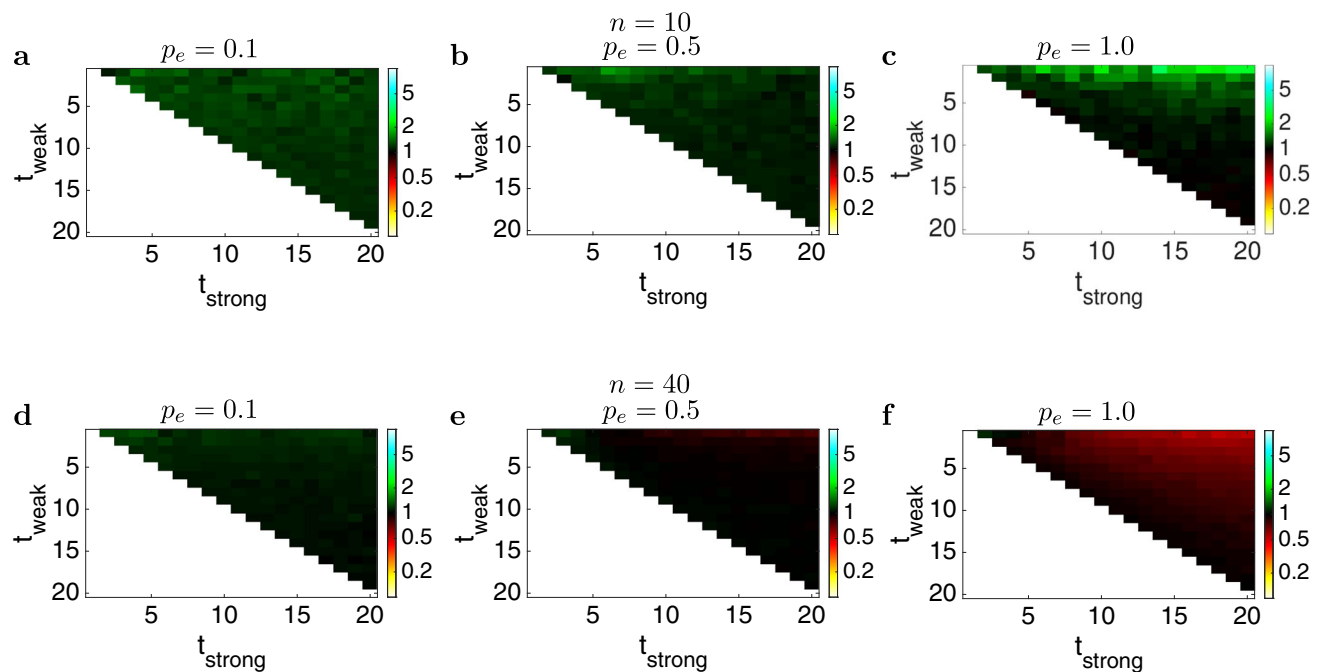
Fig. 8 Varying n , item vector length. REM simulations with half ( n = 10 , a–c) or double ( n = 40 , d–f) the number of features per item. List-length, L = 32 , g = 0.4 , u^* = 0.04 and c = 0.7 . t_{\text{weak}} and t_{\text{strong}} are jointly varied. Panels a–c plot three levels of p_e (0.1, 0.5, and 1.0, respectively), the probability that a repeated item results in an
