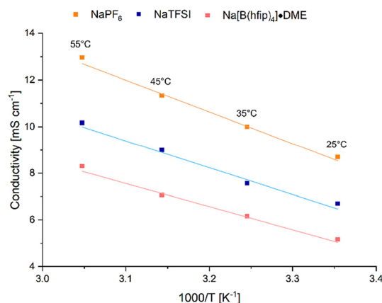
Fig. 5 Arrhenius plot of 1 M \text{NaPF}_6 , 1 M \text{NaTFSI} and 1 M \text{Na[B(hfip)}_4\text{]}\cdot\text{DME} in \text{EC}:\text{DEC} (1:1 v/v) solvent. Bulk conductivity measurements recorded at 25 °C, 35 °C, 45 °C and 55 °C. Electrolytes are 1 M \text{NaPF}_6 (orange), 1 M \text{NaTFSI} (blue) and 1 M \text{Na[B(hfip)}_4\text{]}\cdot\text{DME} (pink) in \text{EC}:\text{DEC} (1:1 v/v).
