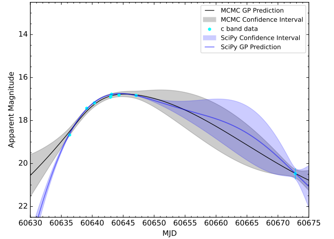
Figure 2. The SciPy and EMCEE optimised fit for the c -band data
