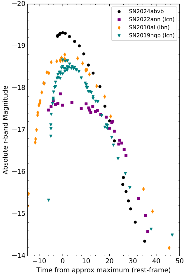
Figure 4. Comparison photometry in the r -band (absolute magnitude) for SN 2024abvb, the Type Ibn (SN 2010al; Pastorello et al. 2015) and two other Type Icn (SNe 2022ann and 2019hgp; Davis et al. 2023).
