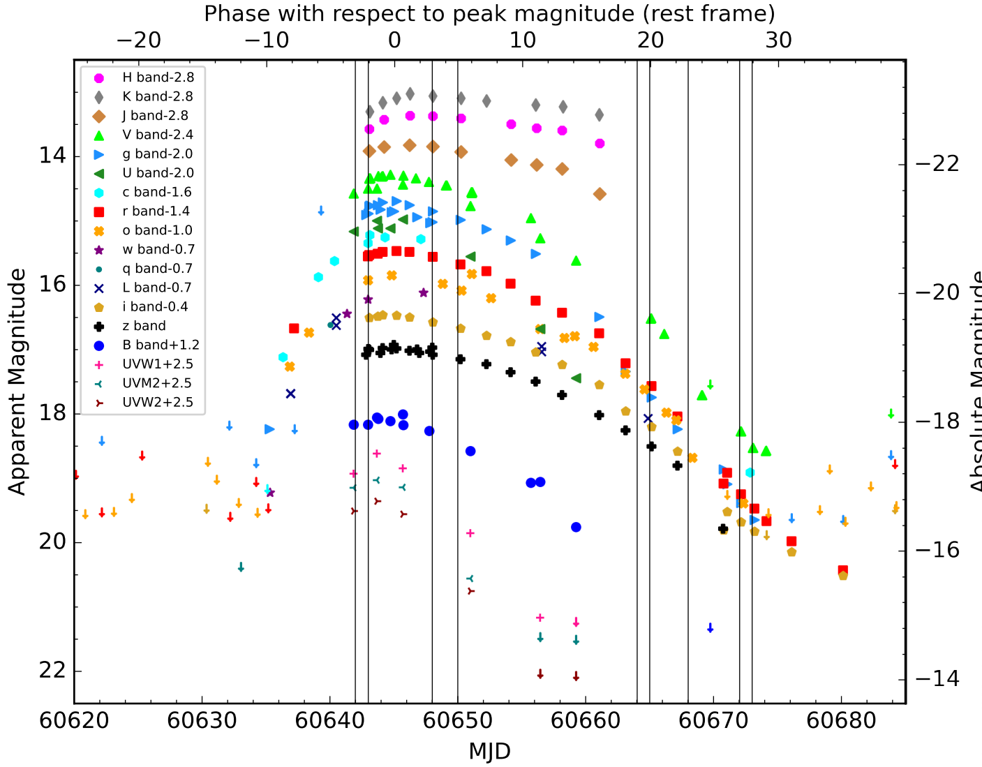
Figure 3. Light curves of SN 2024abvb from AFOSC, ATLAS, Pan-STARRS, LCO, NTT, Swift, NOT, ZTF, REM, TTT, Moravian, BlackGem and GOTO for all available bands from the UV-NIR. The phase is given relative to the V-band maximum. The legend indicates which shape and colour is associated with specific bands. Non-detections are shown with downward arrows. The rise times and decline rates for each band can be seen in Table 2. The vertical black lines indicate the epochs when spectra were taken. The L - and q -bands refer to GOTO and BlackGem bands, respectively. The figure is not extinction corrected. griz are AB magnitudes, as are those of the surveys ATLAS, PS1 and GOTO. UBVJHK are Vega magnitudes.
