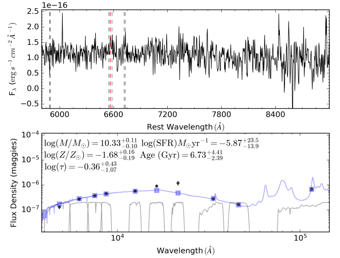
Figure 10. Top panel: Host spectrum with galaxy lines (H \alpha indicated in red, Na I, N II and S II are indicated in black) at the assumed redshift of z = 0.039 . Bottom panel: Best fit SED obtained from PROSPECTOR. The black points are the LIS griz , W1, W2 and W3 and VHS JHKs data points with error bars. The blue boxes and line are the fitted SED and data points. This fit has a reduced \chi^2 = 0.025 .
