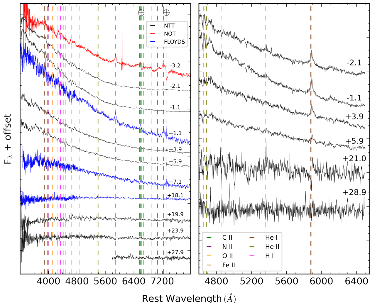
Figure 6. Left panel: All low-resolution spectra (see Table A1), corrected for redshift and reddening, for SN 2024abvb taken between -3.23 days and 27.90 days relative to V -band maximum brightness. The C II, H I, He I, He II, O II, N II and Fe II lines are marked. We see some telluric contamination; however, it leaves the spectral lines mostly unaffected. The cross in this figure shows the telluric lines. Right panel: All medium resolution spectra (see Table A1), corrected for redshift and reddening, for SN 2024abvb taken between -2.05 days and 28.90 days relative to V -band maximum brightness. In all instances, multi-component decomposition was fully resolved, as were the subsequent P-Cygni profiles.
