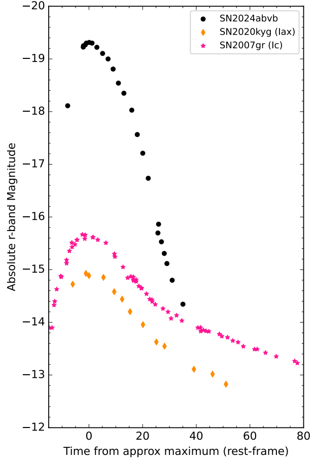
Figure 12. Comparison photometry in the r -band for SN 2024abvb, a Type Iax SN (2020kyg, Srivastav et al. 2022) and a Type Ic SN (2007gr, Hunter et al. 2009).
