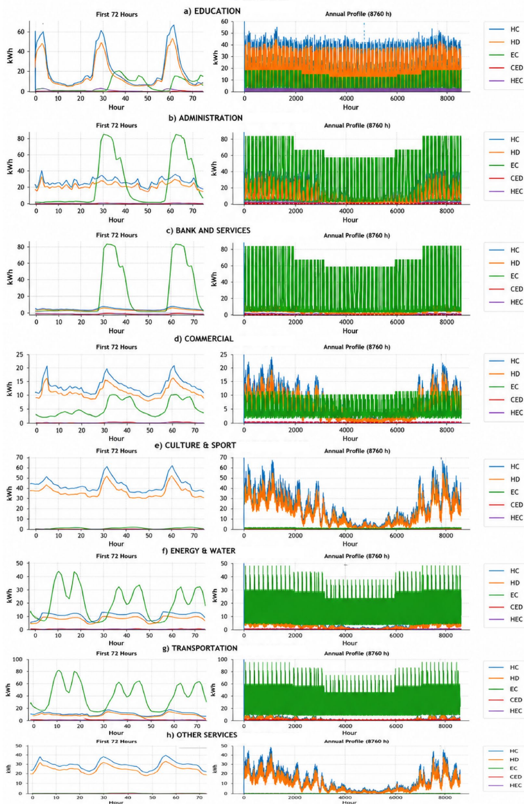
Fig. 4 Average hourly profiles (on left) and Seasonal evolution of hourly tertiary energy demand during the year (on right) of HC(t), HD(t), EC(t), CED(t), and HEC(t) for tertiary building categories ((a) Education, (b) Administration, (c) Banks and Services, (d) Commercial, (e) Culture and Sport, (f) Energy and Water, (g) Transportation and (h) Other Services). Total characteristics are given in Table S4 (Appendix).
