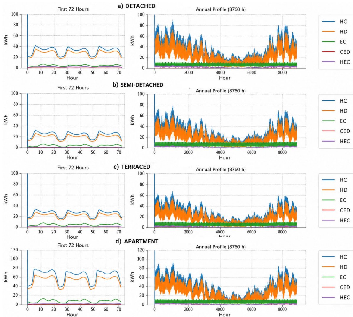
Fig. 3 Average hourly and seasonal energy profiles for residential building typologies in Wallonia. (a–d) Correspond to detached, semi-detached, terraced and apartment buildings, respectively. Profiles are shown for HC, HD, EC, CED and HEC over the 8,760-hour simulation period.
