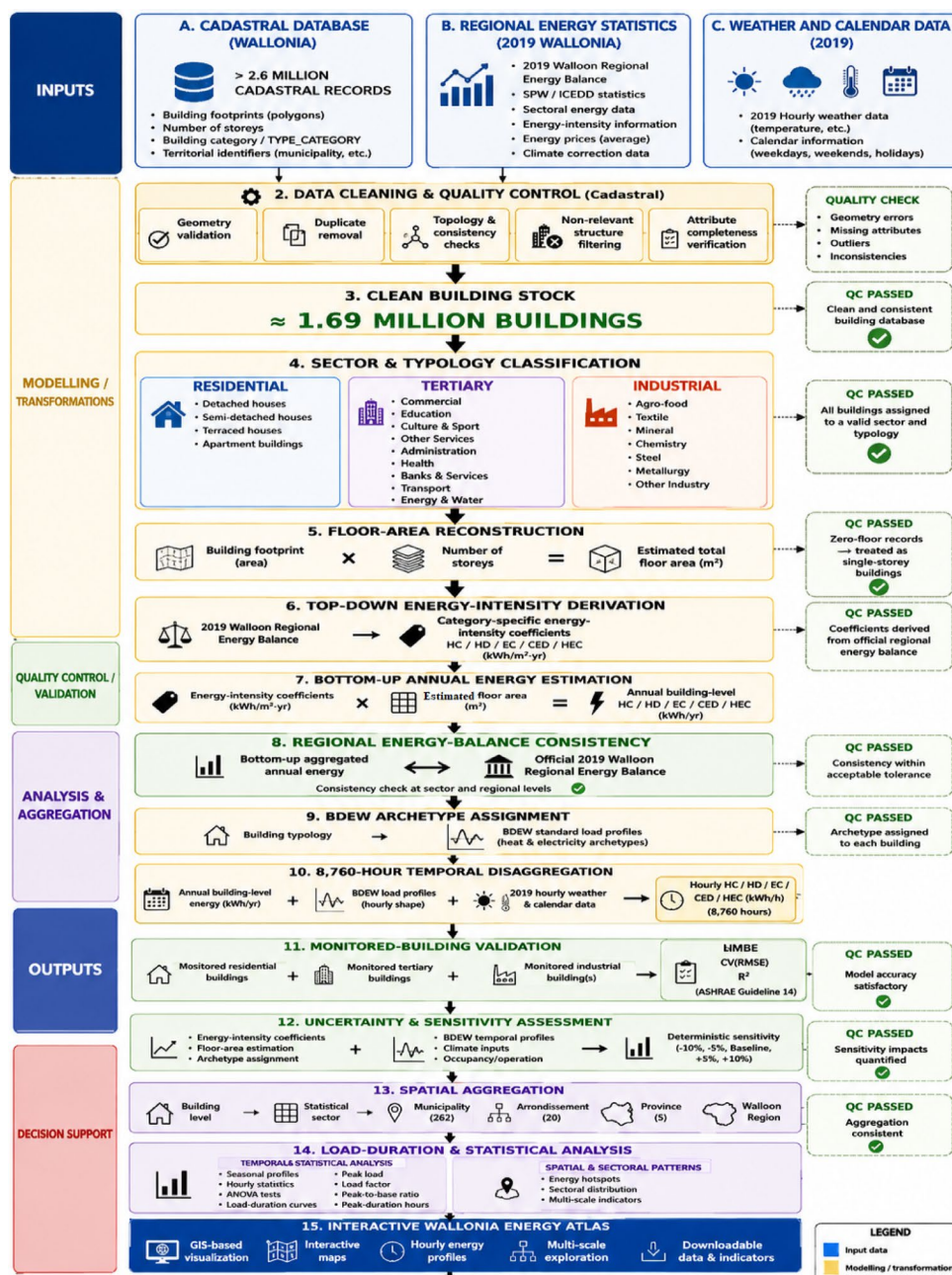
Fig. 1 Step-by-step methodological workflow for the generation, validation, analysis and deployment of hourly building-energy profiles across the Walloon building stock. The workflow distinguishes input datasets, modelling transformations, quality-control and validation procedures, and final analytical and decision-support outputs.
