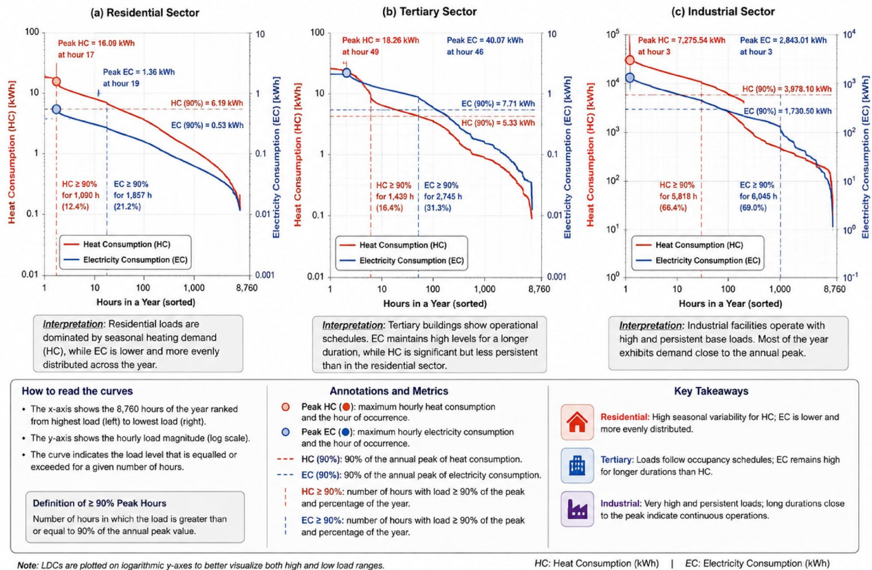
Fig. 6 Load-duration curves of hourly heat and electricity consumption across residential, tertiary, and industrial sectors in Wallonia.
