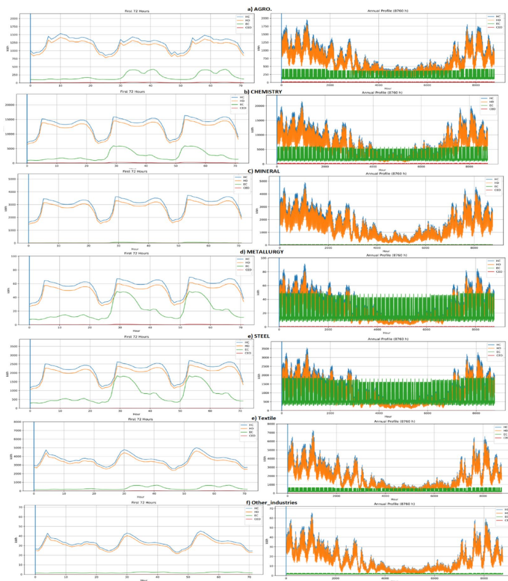
Fig. 5 Average hourly profiles (left) and seasonal evolution of hourly industrial energy demand (right) for HC(t), HD(t), EC(t), and CED(t) for industrial building categories: (a) Agro-food, (b) Chemistry, (c) Mineral, (d) Metallurgy, (e) Steel, (f) Textile, and (g) Other Industries. HEC was not modelled for industrial categories. Overview characteristics are given in Supplementary Table S5.
