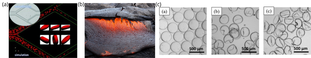
Figure 5. Rheology in nature. (a) Modelling flow of red blood cells (RBCs) in narrow channels using microfluidics and simulation, adapted from [176] published under Creative Commons license (CC BY 3.0). (b) Photograph of a viscous lava flow (adapted from Rufiyaa, CC BY-SA 4.0, via wikimedia commons). (c) A biomimetic model for RBCs, adapted from [177] published under Creative Commons license (CC BY 4.0)
