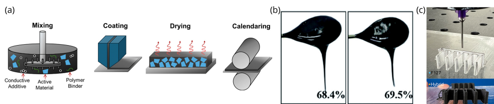
Figure 6. Rheology and manufacturing. (a) Rheological aspects of the battery electrode manufacturing process, adapted from [226] published under Creative Commons license (CC BY 4.0). (b) High solid content cathode slurries, adapted from [227] published under Creative Commons license (CC BY NC NC 3.0). (c) Snapshots of printed hydrogels and advanced materials formulations adapted from [228] published under Creative Commons license (CC BY 4.0)
