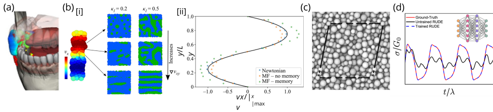
Figure 3. Modelling rheological phenomena. (a) Modelling the breakdown of agar gel during chewing, adapted from [81] reproduced with permission (c) 2014 Wiley. (b) Simulated multi-phase flow using a heterogeneous multi-scale method, adapted from https://arxiv.org/pdf/2211.05080 CC-BY, [82]. Shown are [i] snapshots of the simulated system for different model parameters, and [ii] simulated velocity profiles. (c) Example of a discrete element method (DEM) simulation typically used for studying granular rheology. (d) Rheological prediction made by ML-based model.
