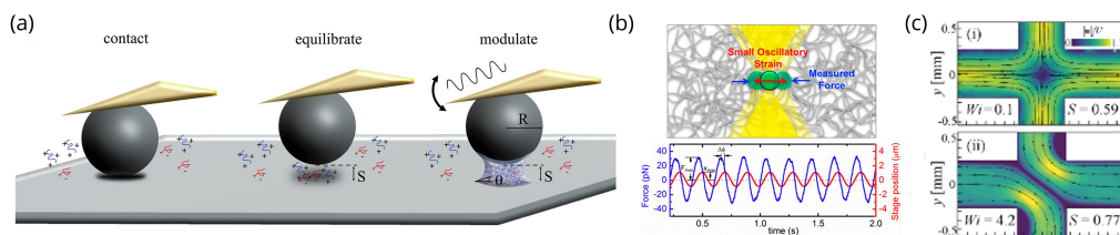
Figure 2. Microrheology and microfluidics. (a) Protein condensate rheology studied using a spherical probe on an atomic force microscopy (AFM) cantilever, adapted from [57] published under Creative Commons license (CC BY 4.0). (b) Sketch illustrating oscillatory microrheology, adapted from [58] published under Creative Commons license (CC BY). (c) Planar extensional flow in a cross-slot geometry, adapted from [59] published under Creative Commons license (CC BY 4.0)
