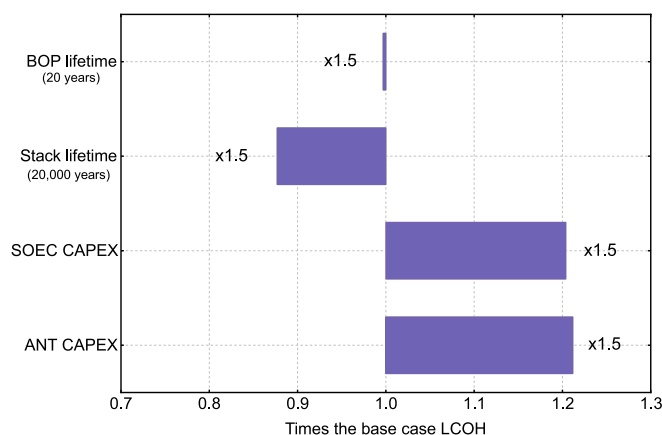
Fig. 11. Normalised sensitivity of LCOH to key ANT and SOEC techno-economic parameters in Scenario 2.
