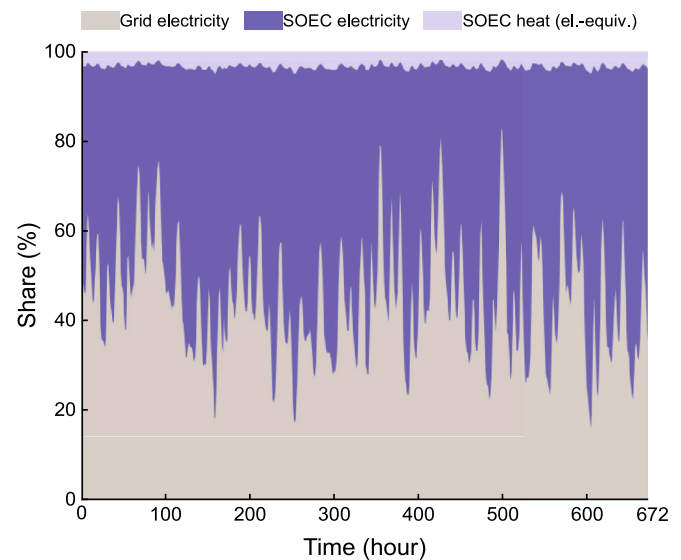
Fig. 8. Plant-level time-varying allocation of ANT-derived energy in the SOEC case, with SOEC heat expressed in electricity-equivalent terms.
