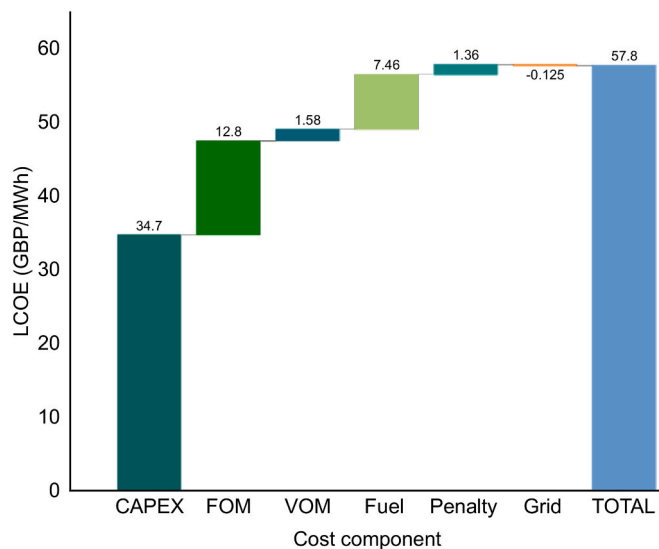
Fig. 6. Plant-level LCOE breakdown for Scenario 1.
