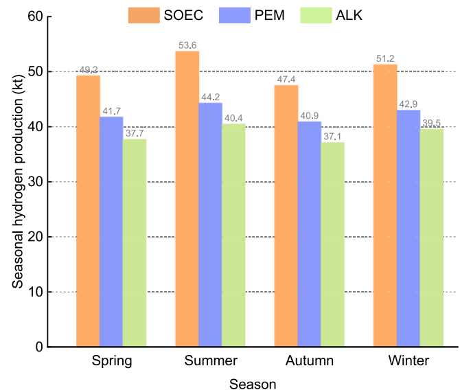
Fig. 9. Seasonal hydrogen production by electrolyser technology.
