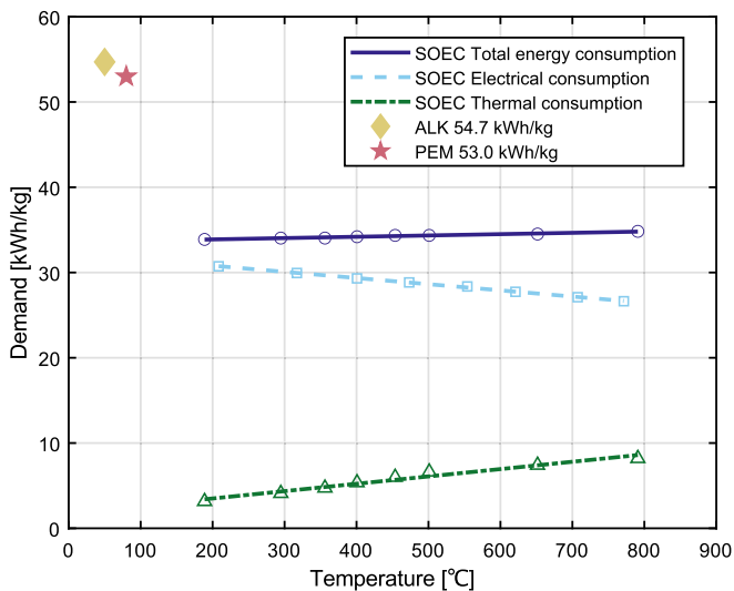
Fig. 2. Temperature-dependent electricity and heat requirements for SOEC hydrogen production [18].
