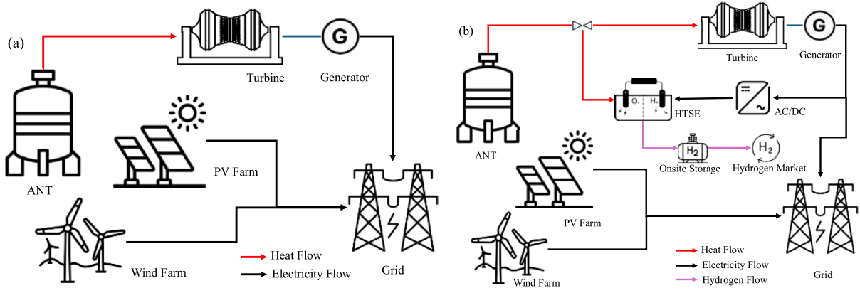
Fig. 1. Alternative configurations of the repurposed nuclear-renewable system at a retired CCGT site: (a) without hydrogen co-generation; (b) with hydrogen co-generation.
