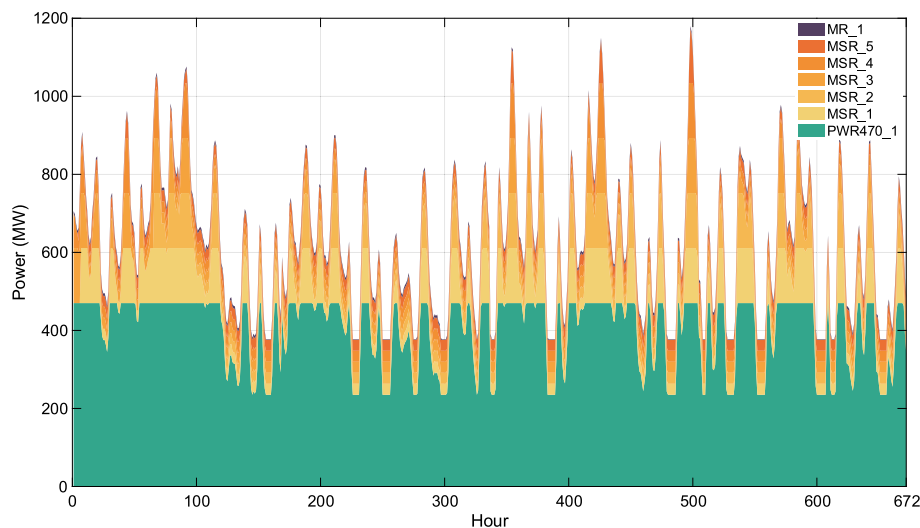
Fig. 5. Plant-level time-varying unit contributions to total electricity output in the ANT-only configuration.
