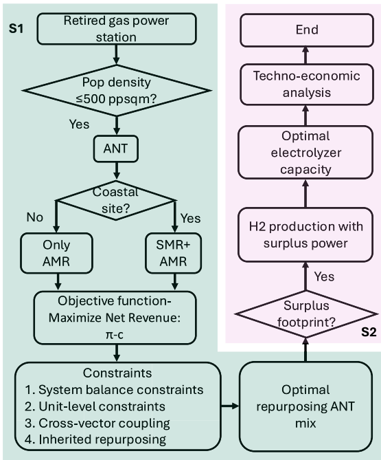
Fig. 3. Workflow for siting screening, repurposing optimisation, and techno-economic evaluation of retired gas power station sites.
