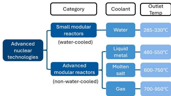
Fig. 4. Classification of Advanced nuclear technologies (ANTs).
