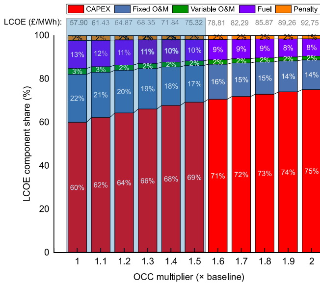
Fig. 7. Decomposition of LCOE into cost components under different OCC multipliers.
