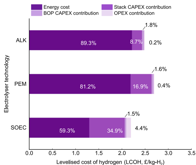
Fig. 10. Plant-level LCOH breakdown under Scenario 2 for three electrolyser technologies.
