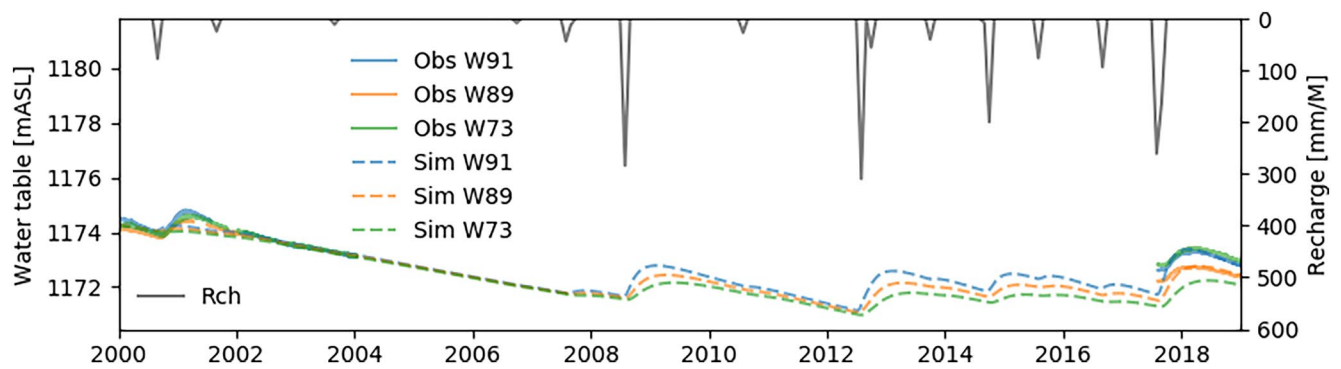
FIGURE 6 | Temporal variation of groundwater recharge at the river cell of the flume F01 (see Figure 1) from the best basin scale model (Section 3.2) (top x-axis), and comparison of simulated and observed values of water table elevation; locations of monitoring wells are shown in Figure 1. Simulated water table elevations were obtained from the 1D groundwater model (see Section 2.5).
