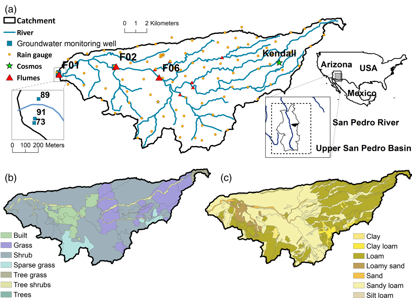
FIGURE 1 | (a) Geographic location of Walnut Gulch Experimental Watershed and location of monitoring stations, (b) land cover, and (c) soil spatial distribution over the basin.
