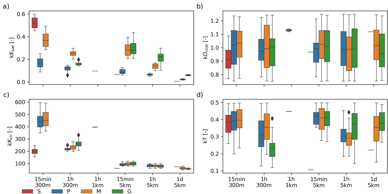
FIGURE 8 | Distribution of parameter factors (a) kK_{sat} , (b) kD_{root} , (c) kK_{ch} , and (d) kT for behavioural simulations based on evaluation at flumes F01, F02 and F06, and soil moisture and AET at Kendall. Results at the 5-km grid size were evaluated only at flume F01. Models using different infiltration methods are represented as P = Philip's, S = Schaaque, G = upscaled Green and Ampt, and M = modified Green and Ampt. Models at 5-km grid size are not considered in the evaluation the evapotranspiration.
