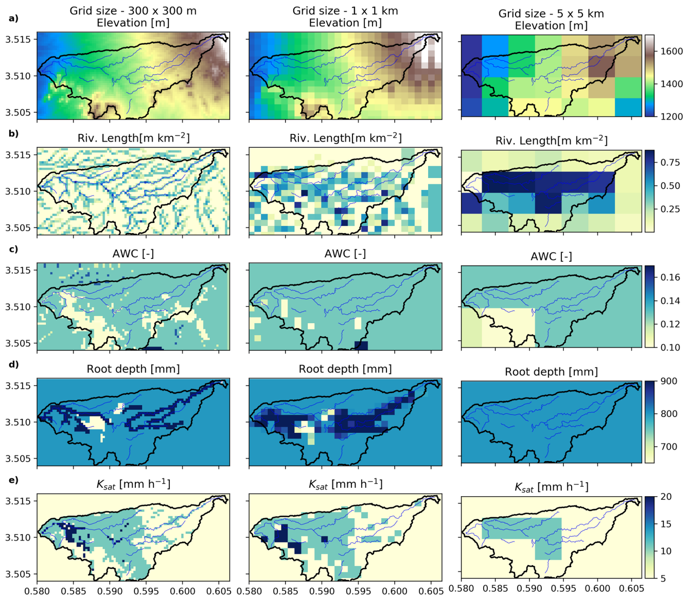
FIGURE 3 | (a) Topography, (b) river length, and soil hydraulic characteristics: (c) available water content (AWC), (d) rooting depth, and (e) K_{sat} saturated hydraulic conductivity for the three different grid scales (300 m, 1, 5 km). Values in square brackets are units and values in parenthesis are grid size, solid black line represent the WGEW, and solid blue lines represent streams. Length units of x and y axis are in 1000 km.
