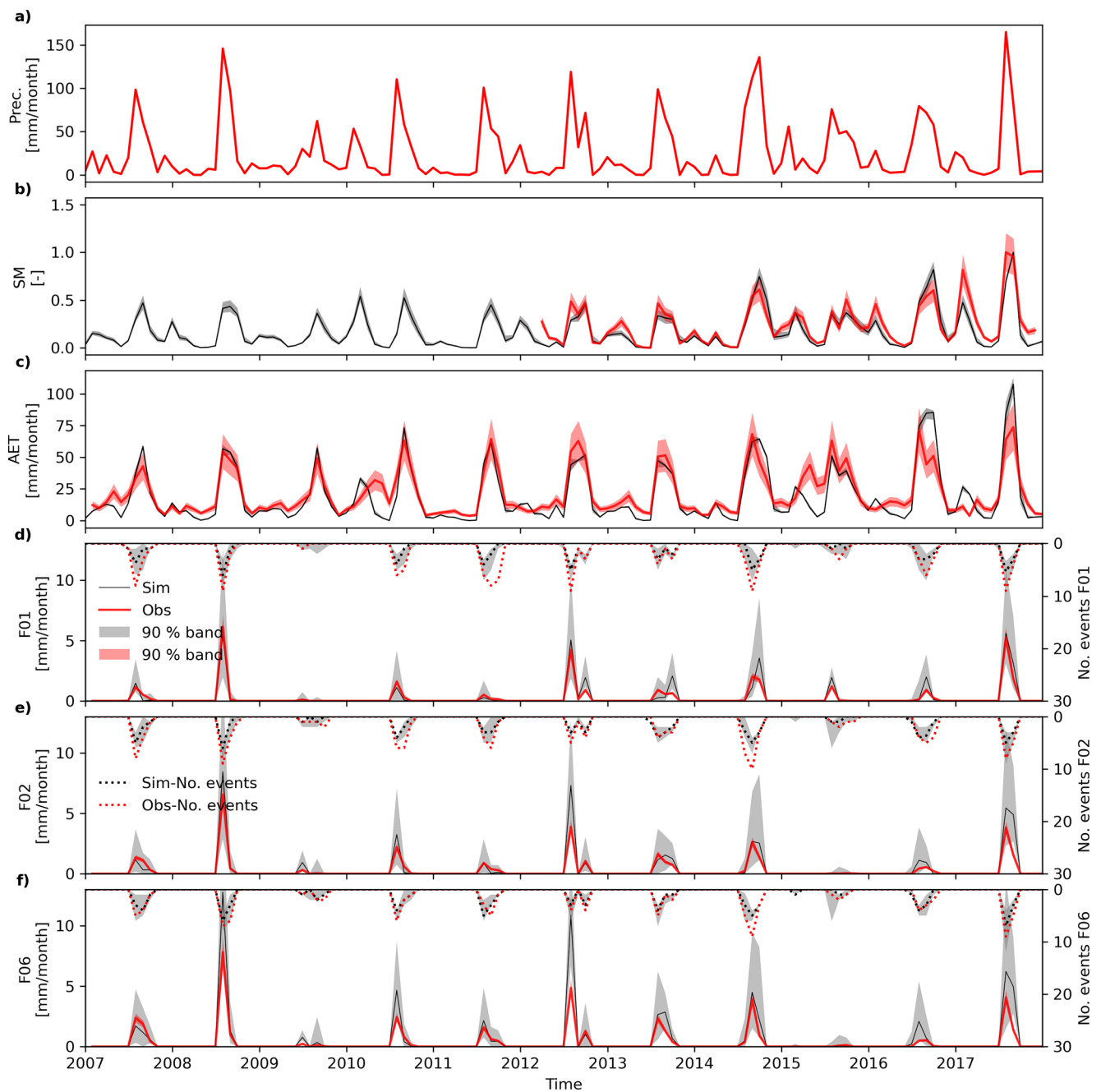
FIGURE 5 | Comparison between observed (red) and simulated (P300m60min) (black) values of monthly temporal variations of (a) precipitation, (b) soil moisture at cosmos Kendall location, (c) actual evapotranspiration at Kendall, (d) streamflow at flume F01, (e) streamflow at flume F02, and (f) streamflow at flume F06. See Figure 1 for station locations.
