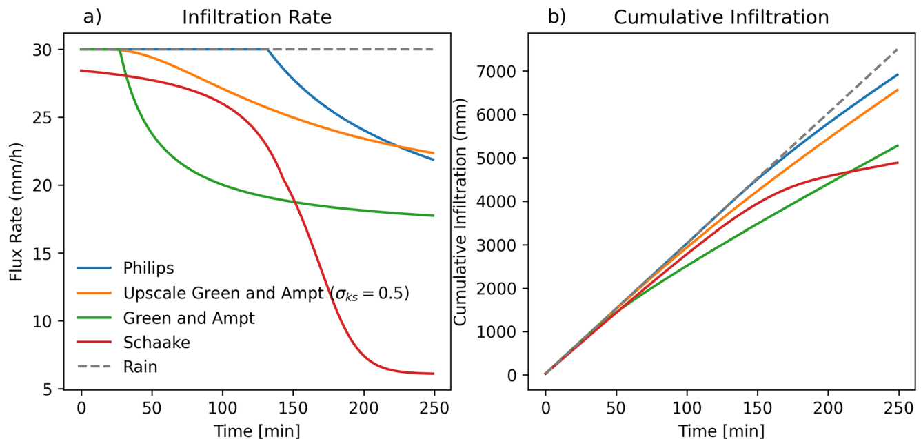
FIGURE A1 | (a) Temporal evolution of infiltration rates simulated by the infiltration approaches used in the main text: Philip (blue), Upscaled Green–Ampt (orange), Green–Ampt (green), and Schaake (red). (b) Cumulative infiltration over the simulation period. Rainfall intensity was held constant throughout the simulation at i = 30 \text{ mm h}^{-1} . The parameters used in the experiment were: Saturated hydraulic conductivity, K_{sat} = 1.6 \text{ cm h}^{-1} ; saturated water content, \theta_{sat} = 0.453 \text{ m}^3 \text{ m}^{-3} ; air-entry pressure at saturation, \psi = 211.01 \text{ mm} ; pore-size distribution index, \lambda = 4.9 [–]; and standard deviation of saturated hydraulic conductivity, \sigma_{K_{sat}} = 0.5 .
