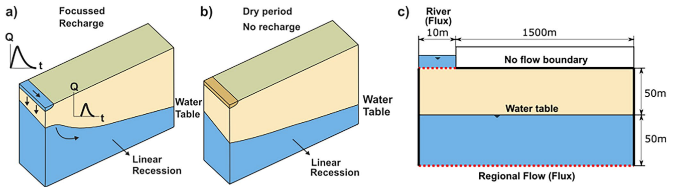
FIGURE 4 | Conceptual model for evaluation of estimated focused recharge, and a diagram for model setup. (a) water table mound during recharge event, (b) water table linear recession after the recharge has occurred, and (c) groundwater model setup and boundary conditions.
