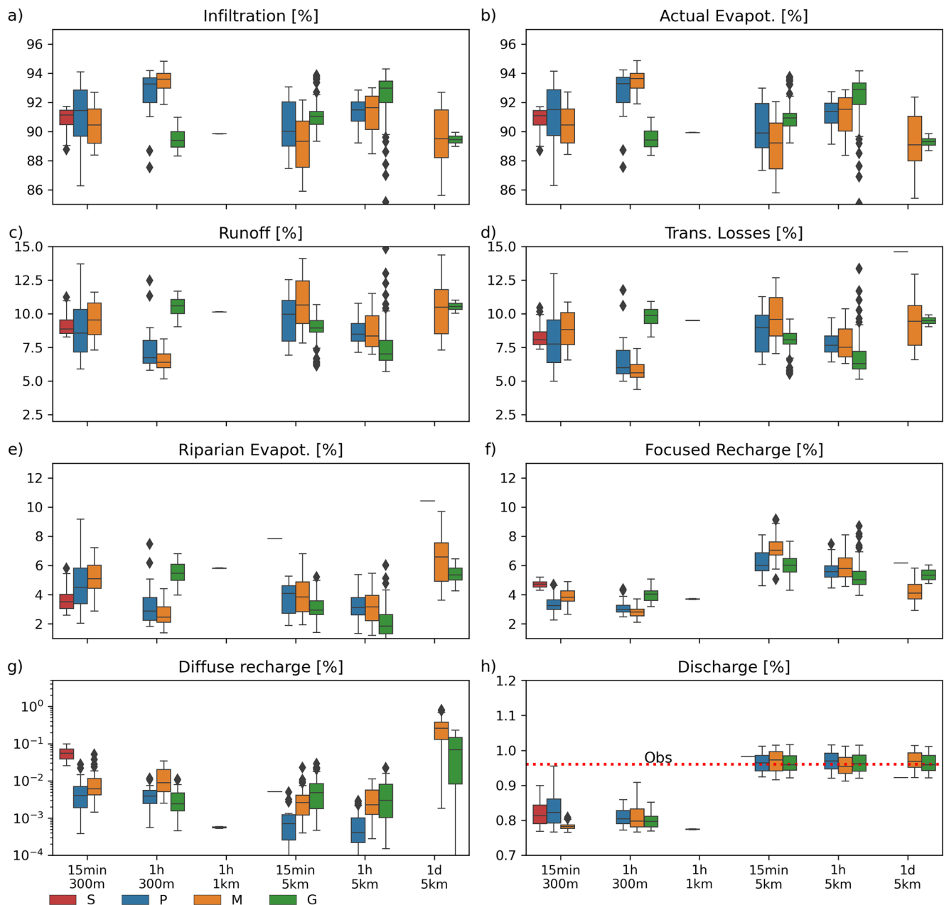
FIGURE 9 | Flux distribution as a percentage of precipitation for behavioural models based on the evaluation at flumes F01, F02 and F06, and soil moisture and AET at Kendall. Results at 5 km grid size were evaluated only at flume F01.
