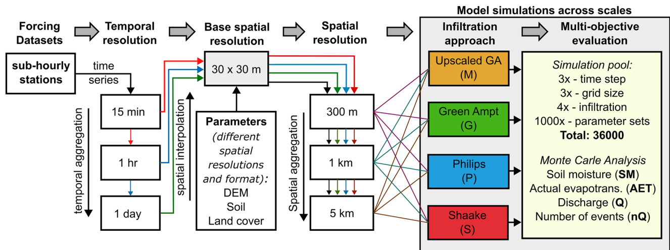
FIGURE 2 | Framework for multi-scale assessment of the effects of temporal and spatial scales on water partitioning (see Appendix A for differences among infiltration approaches).
