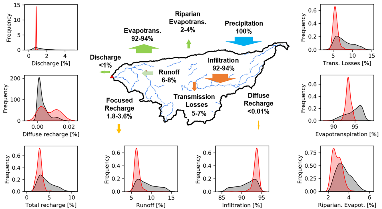
FIGURE 10 | Schematic representation of the water balance components of the WGEW based on the best model: Philips-300m-60min. Arrow scale and direction depend on the magnitude of the components and direction indicates inflow/outflow. Grey shaded areas represent the entire population of model simulations, whereas red shaded areas represent the distribution of behavioural models only.
