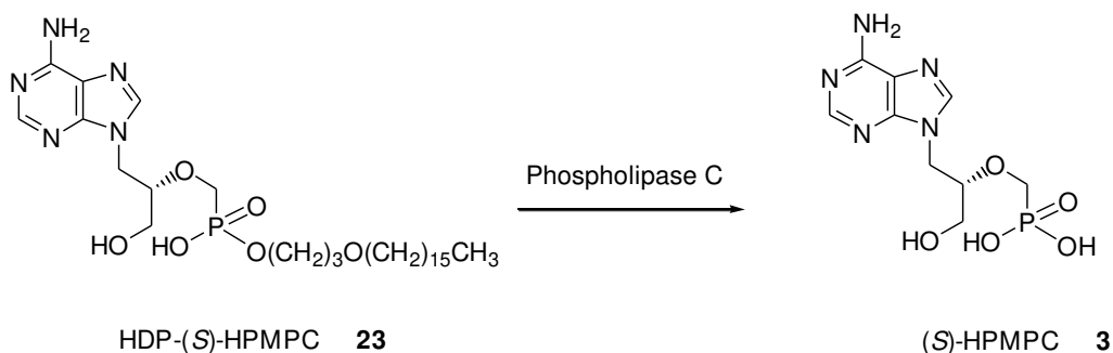
Figure 12. Metabolic pathway for HDP-( S )-HPMPC ( 23 ).
