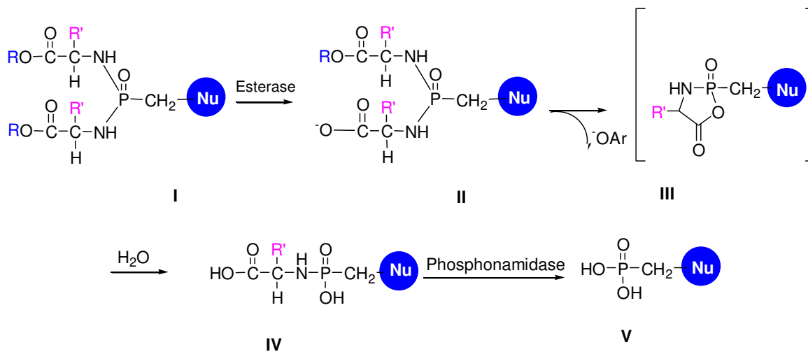
Figure 19. Metabolic pathway for phosphonodiamidate prodrugs.
