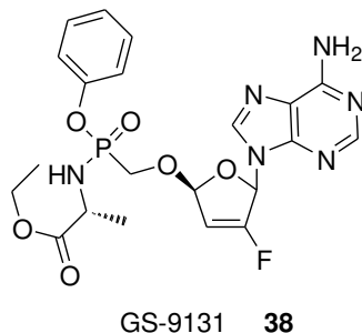
Figure 18. Structure of phosphonoamidate derivative GS-9131 ( 38 ).
