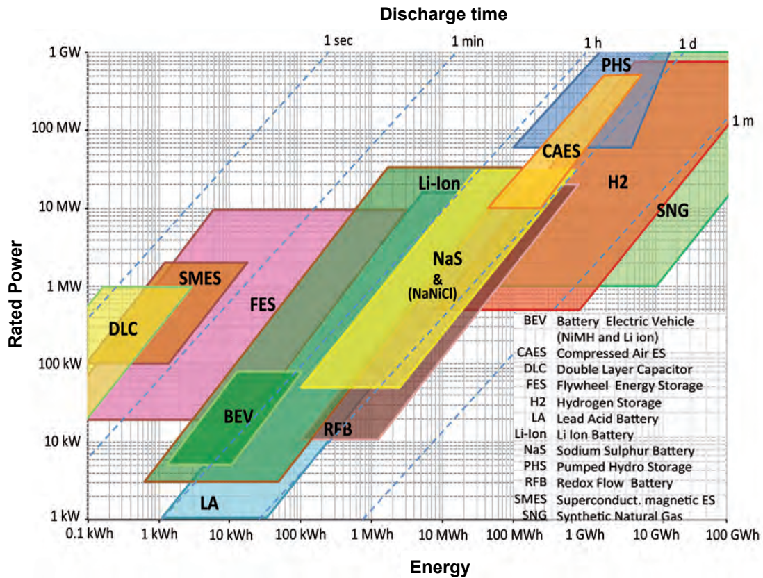
Figure 2: Comparison of rated power, energy content and discharge time of different EES technologies [26] (after Schwunk 2011)
