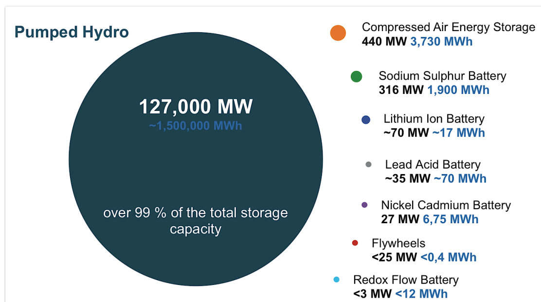
Figure 5: Worldwide installed storage capacity for electrical energy [12]
