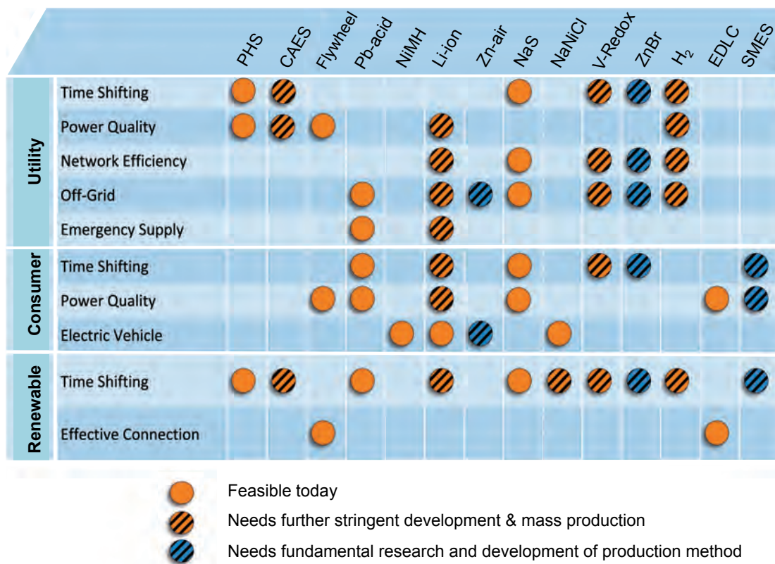
Figure 7: EES present feasibility, future potential, need for further research and development [26, 52] (after Schwunk 2011)
