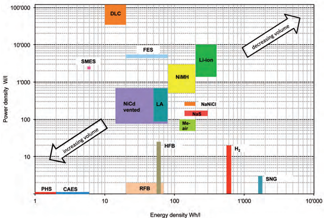
Figure 4: Comparison of power density (Watts/litre of storage facility) and energy density (Watt-hours/litre of storage facility) of EES technologies [26, 52] (after Schwunk 2011)
