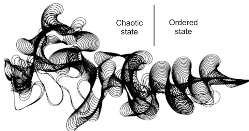
Figure 1.2: Evolution of the river simulated by Stolum (1996). The simulation started with a nearly straight line and evolves to both chaotic (on the left) and ordered state (on the right). The transition between the two states was initiated by a cutoff cluster. “The ordered state in the right part of the figure has reached a mature stage in which the train of bends is still highly symmetrical around the original axis, while at the same time each bend is growing into an asymmetrical shape” (Stolum, 1996, p1711).
