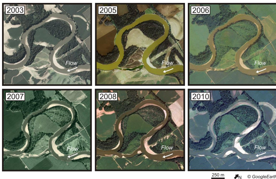
Figure 1.4: Aerial photographs showing the initiation of a chute cutoff on the White River (Indiana, USA).
