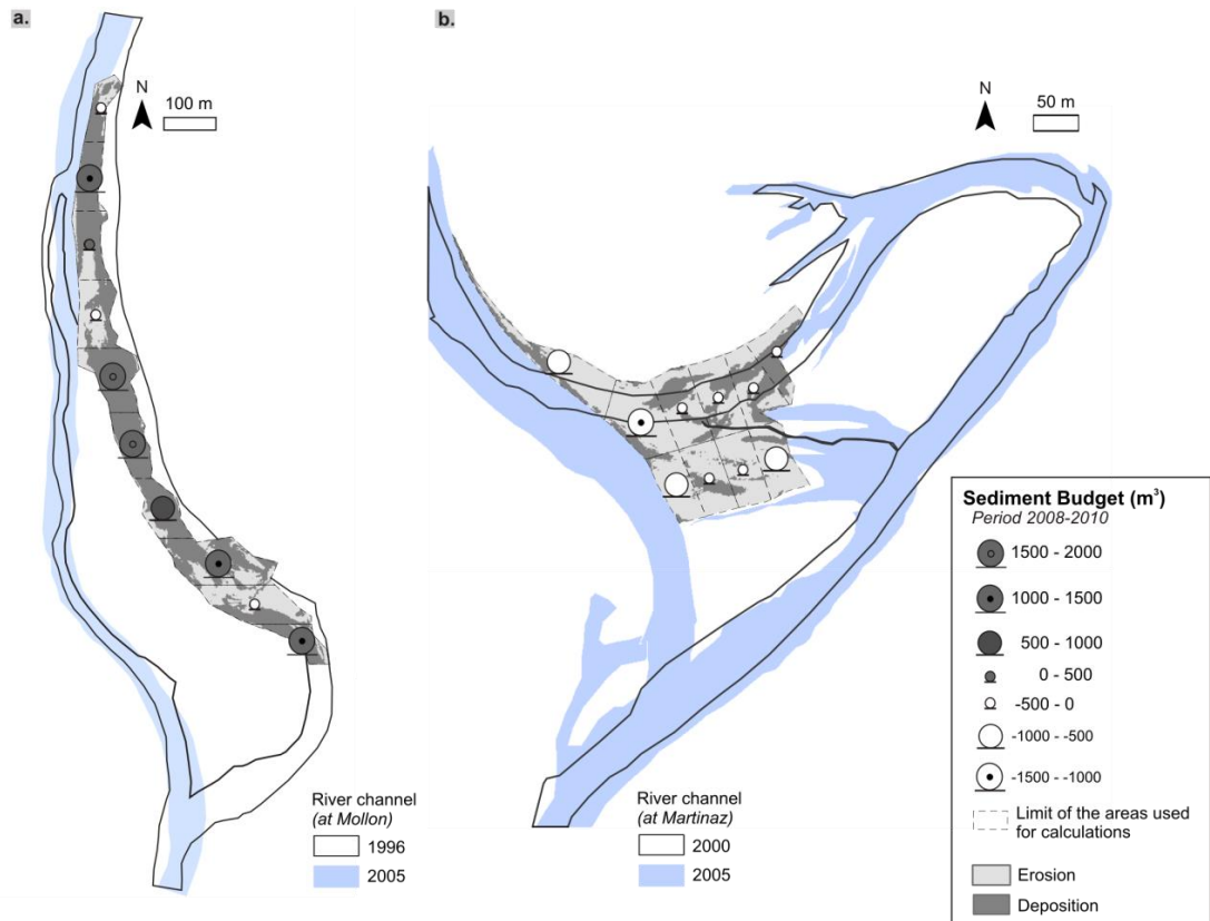
Figure 3.10: Representation of sediment mobilisation for the period 2008-2010. (a) The MOL cutoff site primarily shows areas of net aggradation (dark grey) with up to 2000 m 3 of deposition of sediment in sub-reaches (dark circles). (b) The MAR1&2 cutoff site is primarily erosional with up to 1500 m 3 of sediment loss in sub reaches (white circles). The pre- (dark lines) and post-cutoff (grey shaded area) channel forms show the magnitude of channel change caused by the cutoffs.
