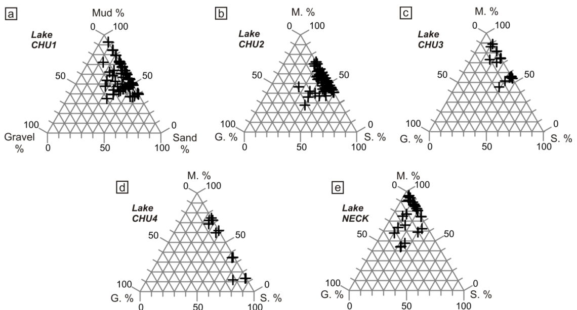
Figure 4.3: Averaged grain size distribution per auger flight. The size fractions considered are clay and silt ( \leq 63 \mu\text{m} ), sand (from >63 \mu\text{m} to \leq 2 \text{ mm} ) and gravel ( >2 \text{ mm} ).
