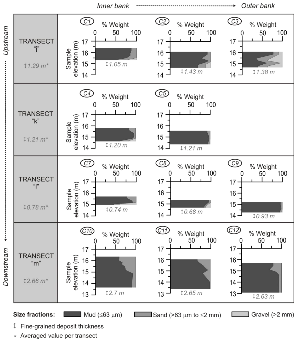
Figure 4.8: Grain size distribution and fine-grained deposit thickness at Lake NECK. It was measured for 11 auger flights from 4 transects located in the abandoned channel. The location references "Upstream-Downstream" and "Inner to Outer Bank" are showing the relative location of auger flights between one another.
