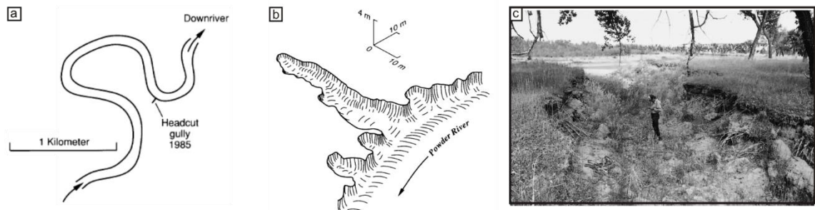
Figure 1.6: Illustration of a headcut that led to chute cutoff on the Powder River (Montana, USA) in 1985.
