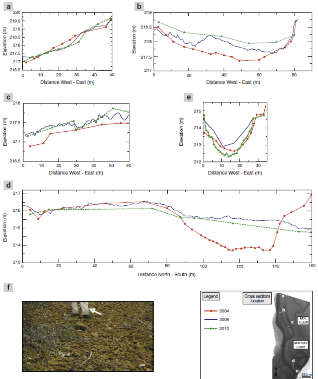
Fig. 6. Cross sections collected along our study reach for the years 2004, 2008, and 2010. Cross section locations are shown on a LIDAR image from 2008, with cross section “a” representing the most upstream location. Differencing of cross sections allowed us to calculate a sediment budget for 2004–2008 and 2008–2010. (f) Photograph of the coarse-grained infill of the MOL cutoff taken in 2011 near cross section “c”; the deposits represent the typical infill of all the cutoff channels in our study reach.
