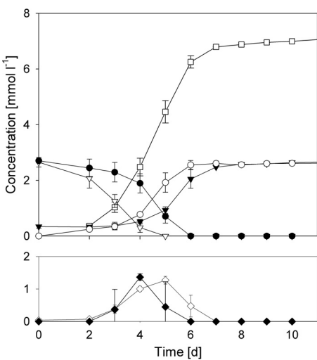
FIG 2 Successive metabolism of trimethylamine, its intermediates, and glycine betaine by Methanococcoides sp. NM1. Both substrates were present in the medium from day 0. Note the different scale in the bottom graph showing the concentrations of intermediates of trimethylamine consumption. Only the first 10 days of the experiment are shown. The cultures were monitored for another 3 weeks but did not show any significant concentration changes. All values are the averages of three replicates, with the error bars indicating 1 standard deviation. □, methane; ●, glycine betaine; ○, N,N -dimethylglycine; ▽, trimethylamine; ▼, ammonium; ◆, dimethylamine; ◇, methylamine.
