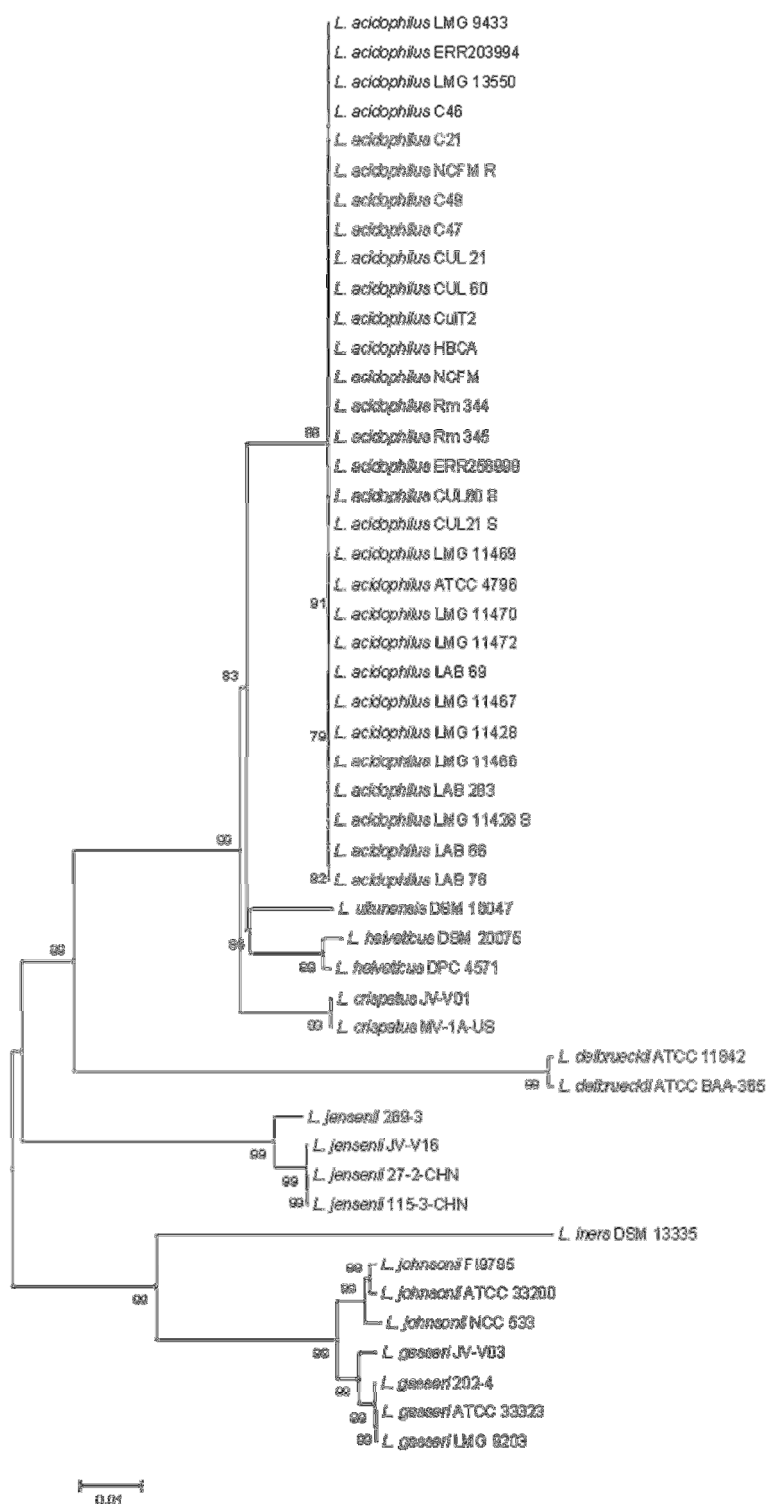
Figure 4.4: Neighbour Joining phylogeny of concatenated ribosomal protein genes from L. acidophilus group isolates
