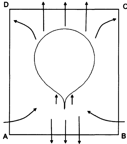
Figure 6.20: Indication of direction of velocities in rising bubble with negative wake, resulting in an additional upward thrust.
