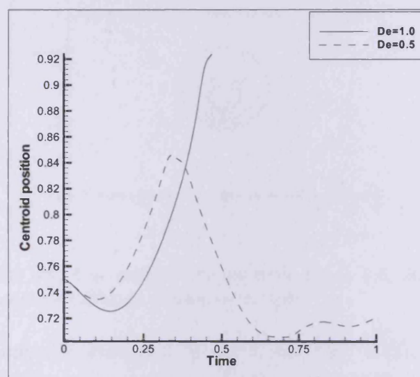
Figure 5.30: Bubble centroid position for h = 0.75 with different De .
