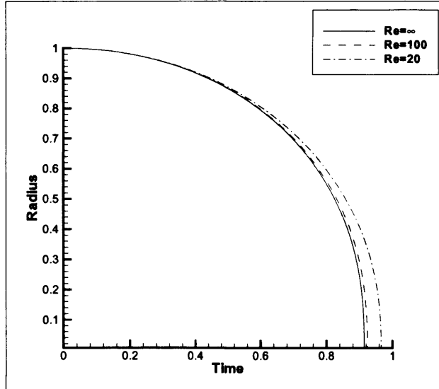
Figure 2.16: Variation of radius with time for a Jeffreys fluid, with \lambda_1 = 10 and \mu_p = 0 ( \beta = 1 ).
