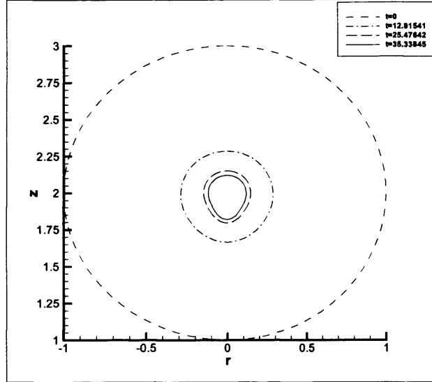
Figure 3.26: Bubble surface profiles at different stages of collapse at a distance h = 2.0 , Re = 0.2 , De = 5 .
