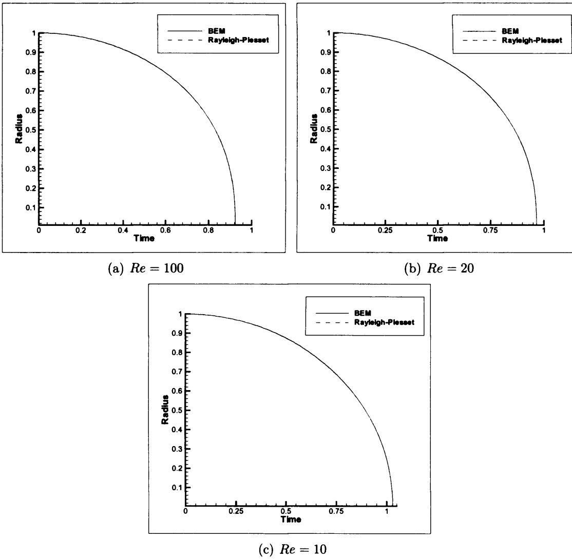
Figure 2.4: Comparison of the BEM to the numerical solution of the Rayleigh-Plesset equation for a selection of Reynolds numbers.
