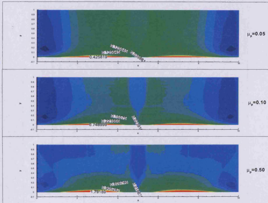
Figure 7.37: The stress contours of component T_{xx} for different polymeric viscosities. The remaining parameters are We = \mu_s = 0.1 , h = 1.1 .
