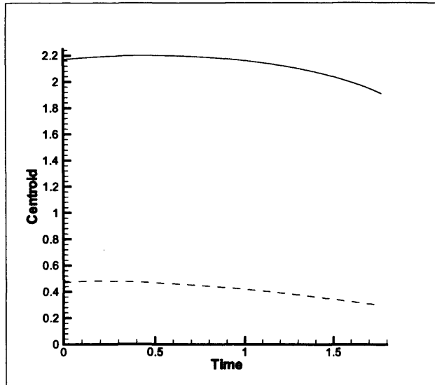
Figure 4.6: Evolution of bubble centroids. h_2 = 0.47 , h_1 = 2.17 , R_2 = 0.57 .
