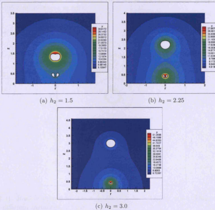
Figure 4.29: Pressure contour plots for varying h_2 with De = 1 , Re = 2 , h_1 = 0.5
