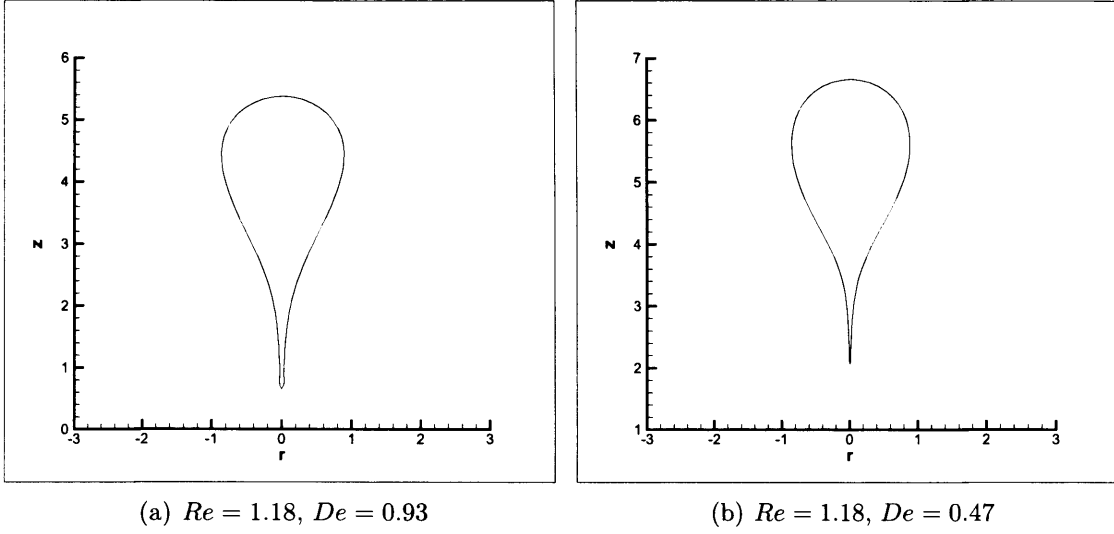
Figure 6.23: Steady state bubble shapes for the Upper Convected Maxwell (UCM) constitutive equation.
