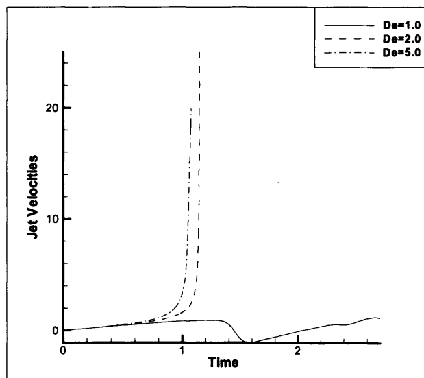
Figure 3.19: Jet velocities during collapse with varying De . Re = 1 and h = 1.5 .
