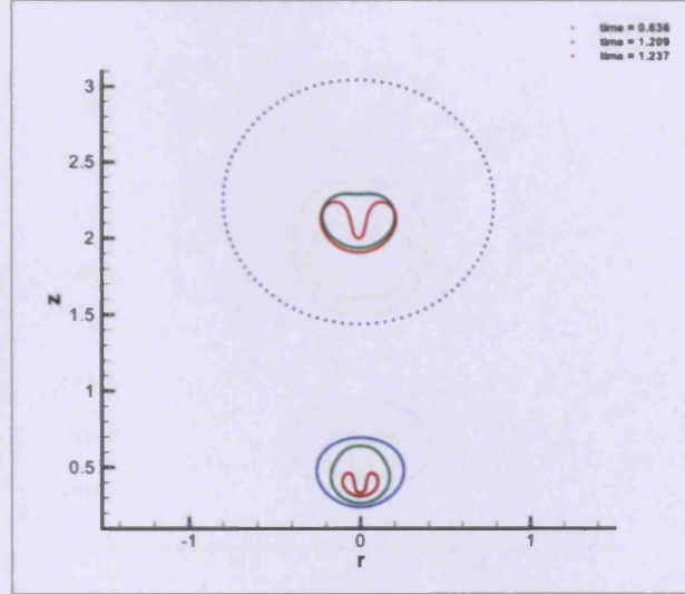
Figure 4.24: Bubble shapes for De = 2.5 , Re = 2 , h_1 = 0.5 , h_2 = 2.25 . Different colours indicate different instances in time.
