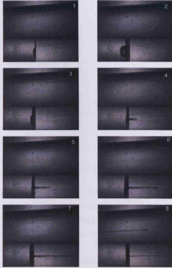
Figure 5.41: Jet formation in Newtonian silicon oil, with a shear viscosity of 0.18\text{Pa}\cdot\text{s} . 3
