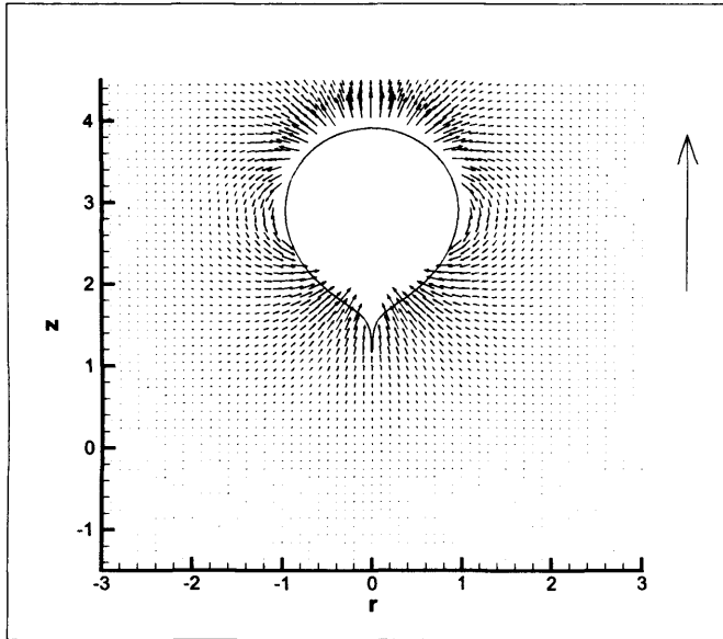
Figure 6.19: Velocity field in the fluid around the rise bubble. The velocity in the wake of the bubble is everywhere directed upwards, i.e. there is no negative wake.
