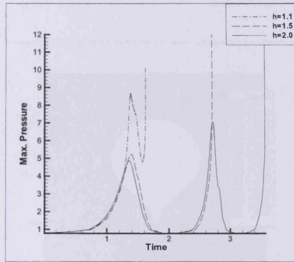
Figure 3.40: Maximum pressure with time at different heights Re = 1 , De = 1 .
