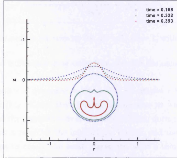
Figure 5.14: Bubble and free surface shapes with De = 1 , Re = 1 at h = 0.5 . Different colours indicate different instances in time.
