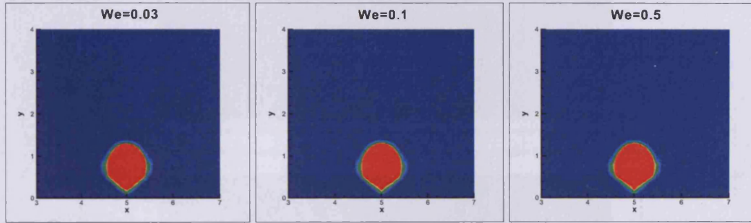
Figure 7.33: A plot of the colour function at t = 0.5 for different Weissenberg numbers. The remaining parameters are \mu_p = \mu_s = 0.1 , h = 1.1 .
