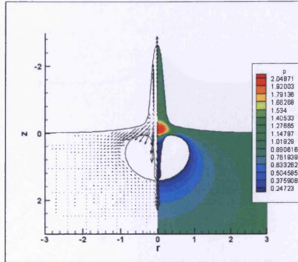
Figure 5.10: Pressure contours and velocity vectors at t = 0.973 for an inviscid fluid ( h = 0.5 ).
