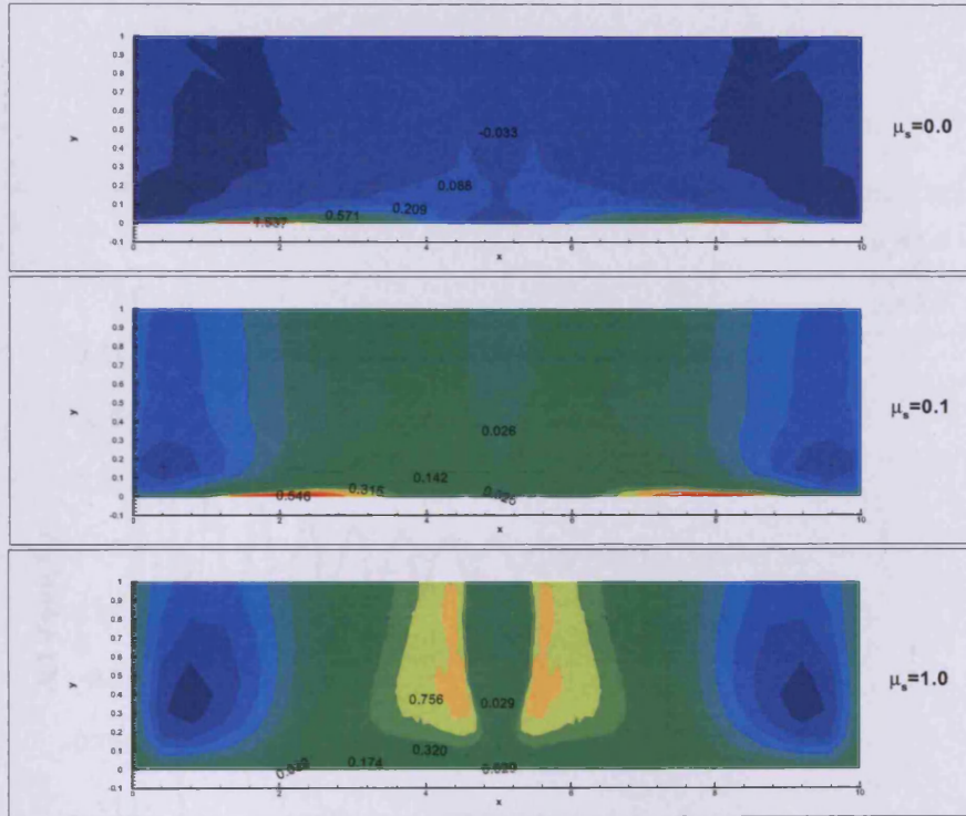
Figure 7.31: The stress contours of component T_{xx} for different solvent viscosities \mu_s . The remaining parameters are \mu_p = 0.1 , We = 0.03 , h = 1.1 .
