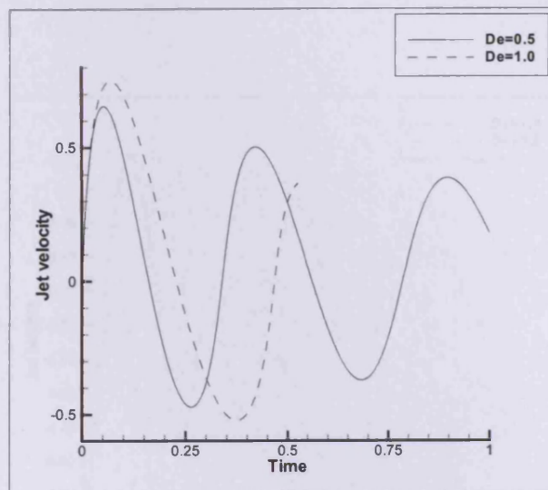
Figure 5.33: Free surface jet velocity for h = 1.0 with different De .
