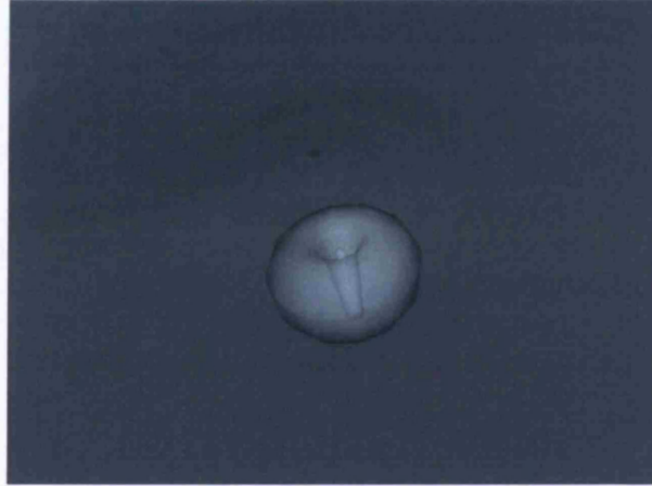
Figure 5.18: 3D visualisation of Fig. 5.17.
