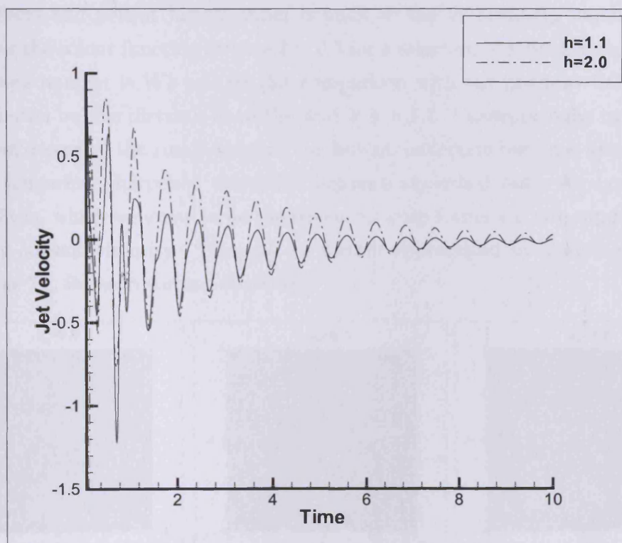
Figure 7.29: Variation of the jet velocity with time, at different distances h from the wall, in a UCM fluid with \mu_p = 0.1 , We = 0.03 .
