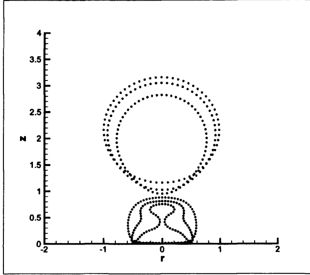
Figure 4.5: Bubble shapes of two different-sized bubbles near a rigid boundary. h_2 = 0.47 , h_1 = 2.17 , R_2 = 0.57 . Different colours indicate different instances in time.
