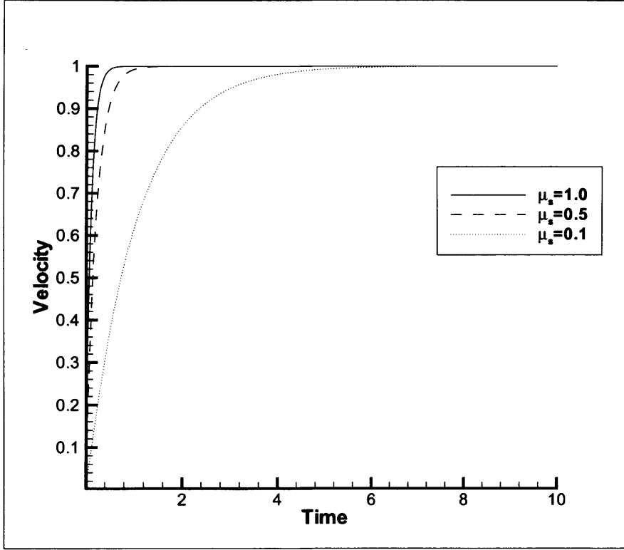
Figure 7.7: Numerical approximation of horizontal velocity component u(0.5, 0.5, t) with time for Poiseuille flow. Here c^2 = 1 \times 10^3 and the channel length is L = 1 .
