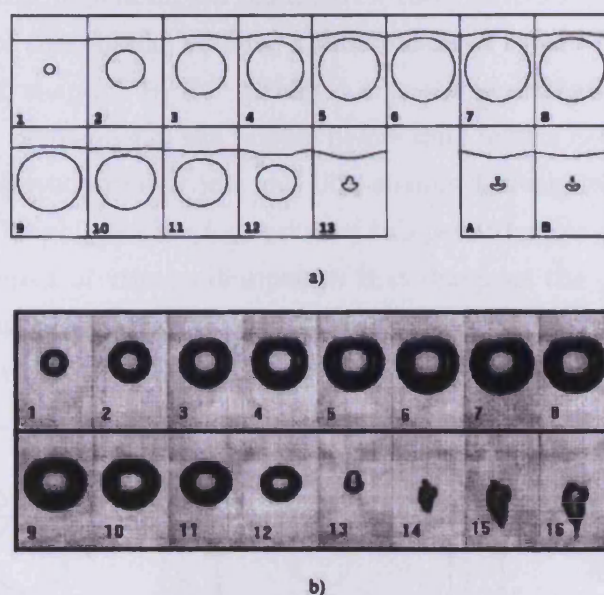
Figure 5.39: Bubble collapse near an elastic medium 2 .
