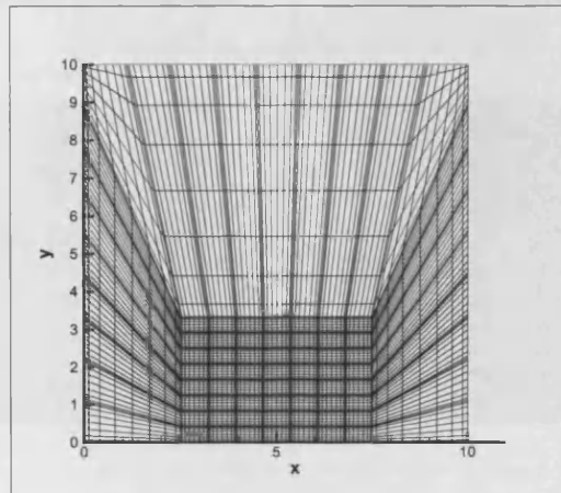
Figure 7.14: An example of the spectral element mesh used in the bubble collapse problems.
