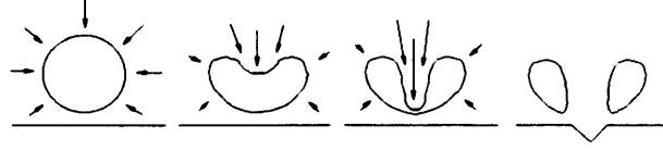
Figure 1.2: Sketch of jet formation and impact during collapse near a rigid wall - and the possible damage that results.
