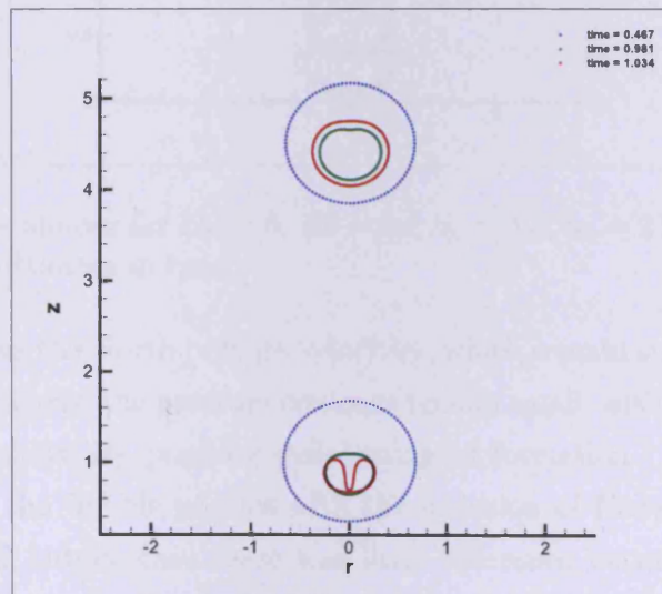
Figure 4.17: Bubble shapes for De = 1 , Re = 2 , h_1 = 1.0 , h_2 = 4.5 . Different colours indicate different instances in time.
