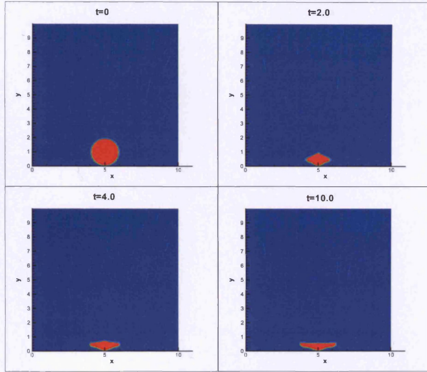
Figure 7.17: Bubble collapse near a wall in a Newtonian fluid with \mu_s = 0.1 .
