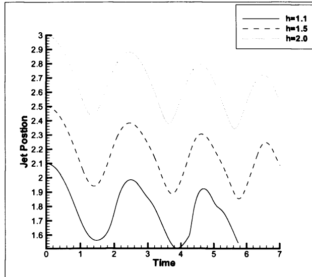
Figure 3.27: Position of jet point on z axis with time, Re = 0.2 , De = 5 , for varying height.
