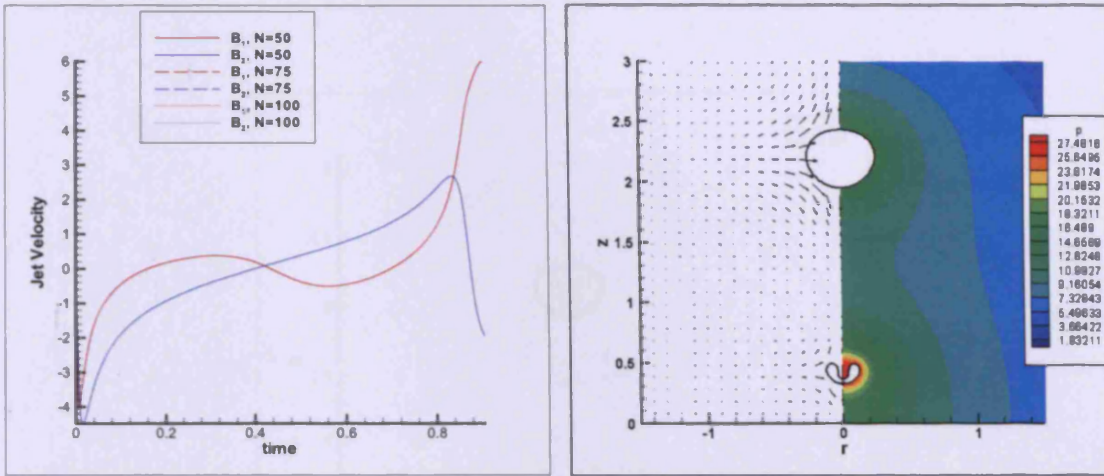
(a) North pole jet velocities for different mesh refinement. (b) Velocity vector and pressure contour plots at t \approx 0.9 .
