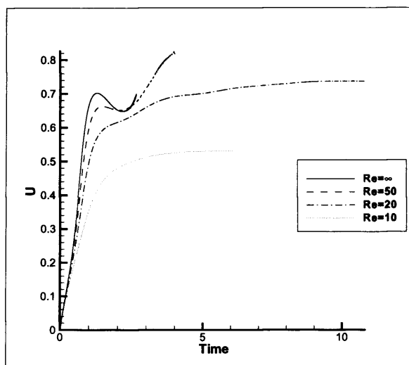
Figure 6.7: Evolution of the rise velocity for a selection of Reynolds numbers with E\ddot{o} = 6.6 .
