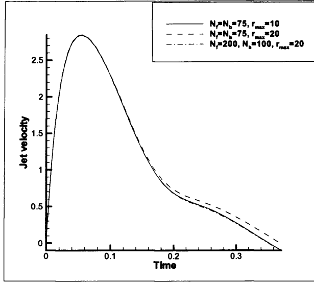
Figure 5.16: Free surface jet velocity for De = 1 , Re = 1 , with varying mesh refinement and r_{max} values.
