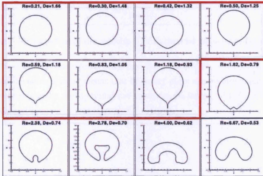
Figure 6.13: Final profiles of rising bubbles of different volumes in a viscoelastic fluid. Steady state bubble shapes reside within the red box.
