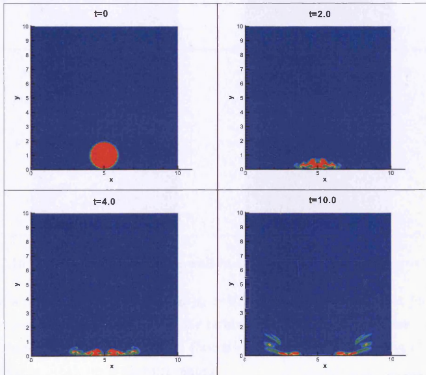
Figure 7.15: Bubble collapse near a wall in a Newtonian fluid with \mu_s = 1 \times 10^{-3} .
