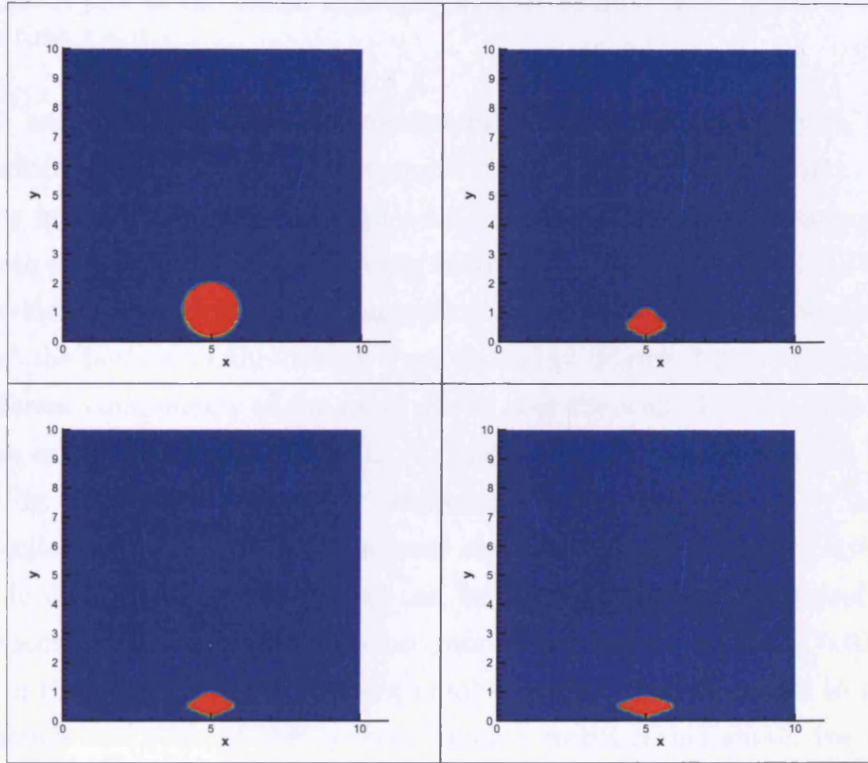
Figure 7.23: A plot of the colour function at different times, representing bubble collapse near a wall in a UCM fluid with \mu_p = 0.1 , We = 0.03 , h = 1.1 .
