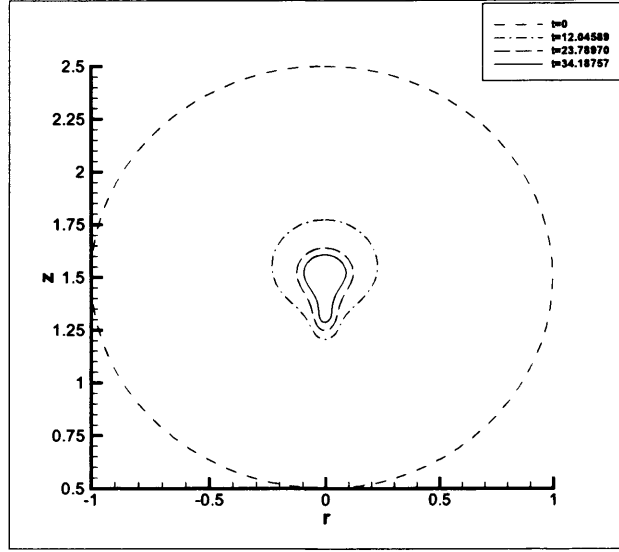
Figure 3.25: Bubble surface profiles at different stages of collapse at a distance h = 1.5 , Re = 0.2 , De = 5 .
