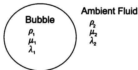
Figure 7.1: Schematic of bubble and ambient fluid, each with different densities and material properties.
