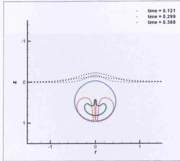
Figure 5.17: Bubble and free surface shapes with De = 0.5 , Re = 1.0 at h = 0.5 . Different colours indicate different instances in time.
