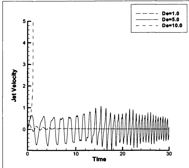
Figure 3.32: Jet velocities during collapse with varying De . Re = 0.2 and h = 1.5 .
