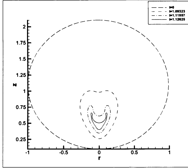
Figure 3.7: Bubble surface profiles at different stages of collapse at a distance h = 1.1 , Re = 20
