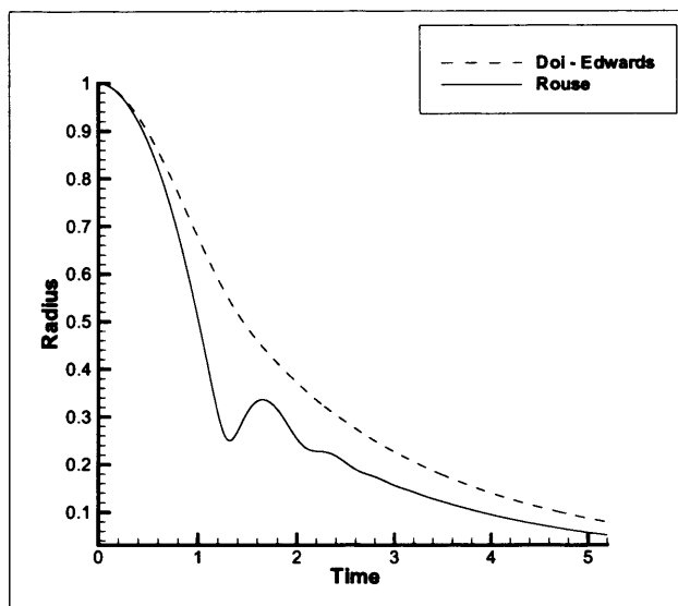
Figure 2.17: Variation of bubble radius with time for Rouse and Doi-Edwards like fluids, with \lambda_0 = 0.5 , \mu_0 = 0.5 .
