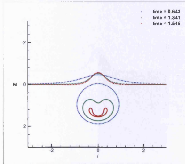
Figure 5.9: Bubble and free surface shapes with Re = 50 at h = 1.0 . Different colours indicate different instances in time.
