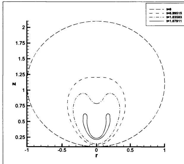
Figure 3.4: Bubble surface profiles at different stages of collapse at a distance h = 1.1 , Re = \infty
