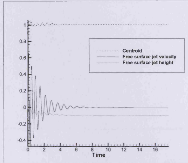
Figure 5.36: Bubble centroid position, free surface jet position and free surface velocity for h = 1.0 , De = 0.5 , Re = 1.0 .
