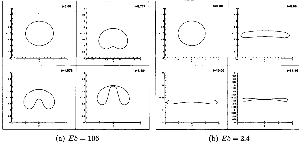
Figure 6.4: Bubble profiles at select times during ascent for Re = 50 .
