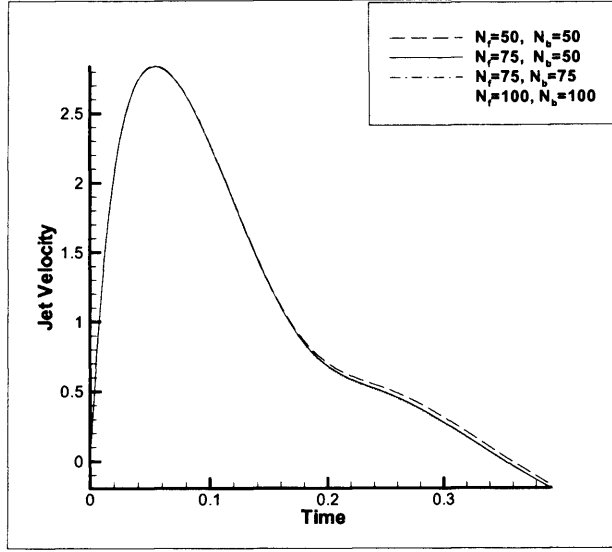
Figure 5.15: Free surface jet velocity for De = 1 , Re = 1 , with mesh refinement
