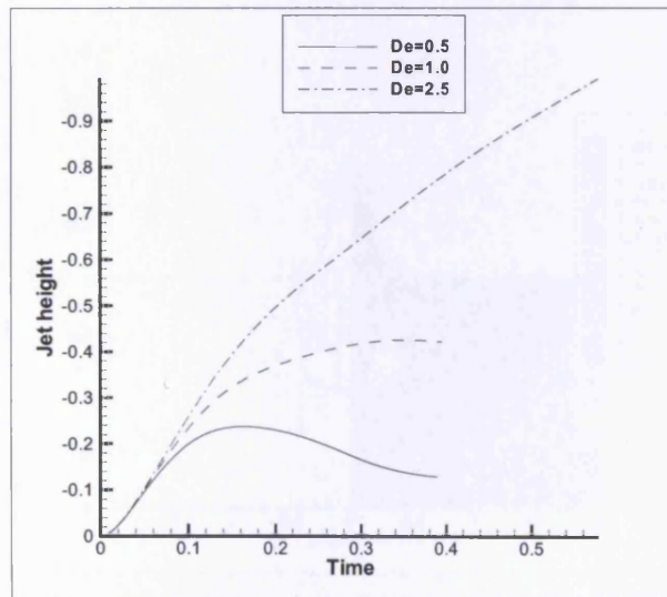
Figure 5.21: Free surface jet height for h = 0.5 with different De .
