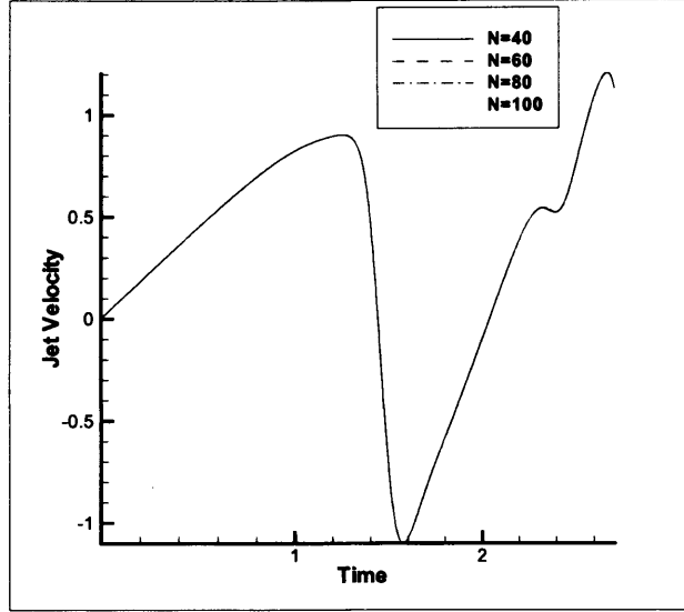
Figure 3.21: Jet velocity with different mesh refinements for De = 1 , Re = 1 , h = 1.5
