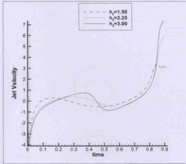
Figure 4.28: Jet velocities in B_1 at h_1 = 0.5 , for varying h_2 ( De = 1 , Re = 2 ).
