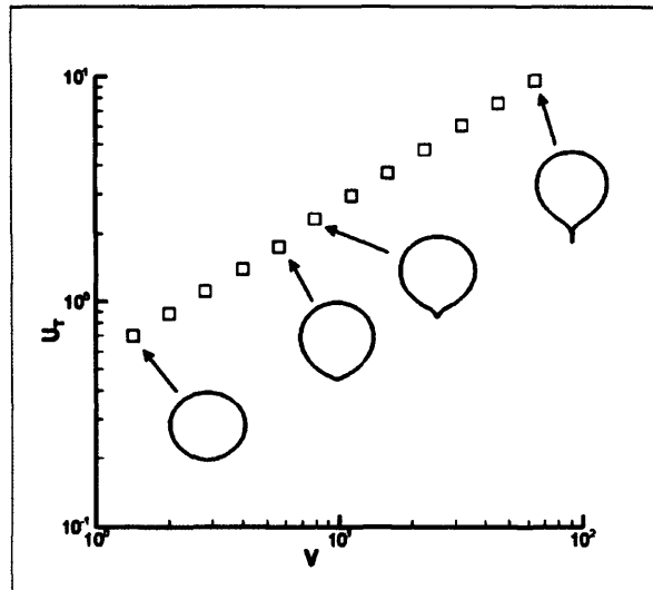
Figure 6.18: Terminal rise velocity for different bubble volumes. Noteworthy bubble shapes are indicated at particular bubble volumes.
