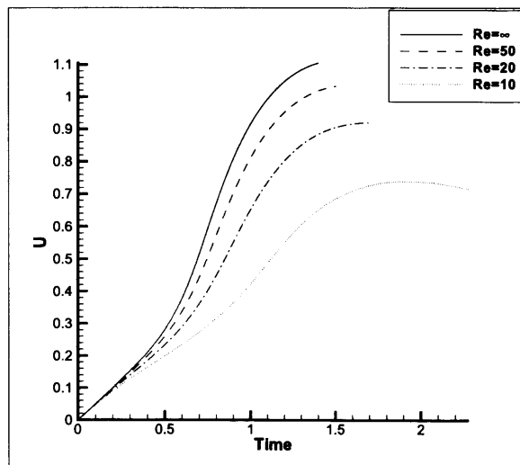
Figure 6.6: Evolution of the rise velocity for a selection of Reynolds numbers with Eö = 106 .
