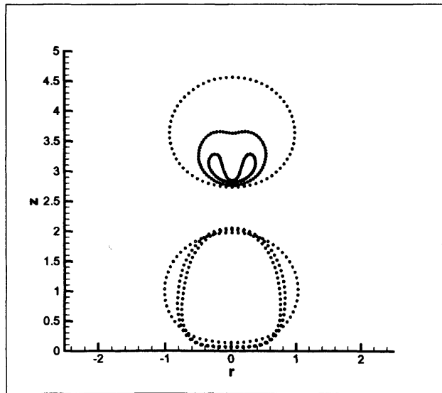
Figure 4.3: Bubble shapes of two approximately equal-sized bubbles near a rigid boundary. h_2 = 0.99 , h_1 = 3.60 , R_1 = 0.94 . Different colours indicate different instances in time.
