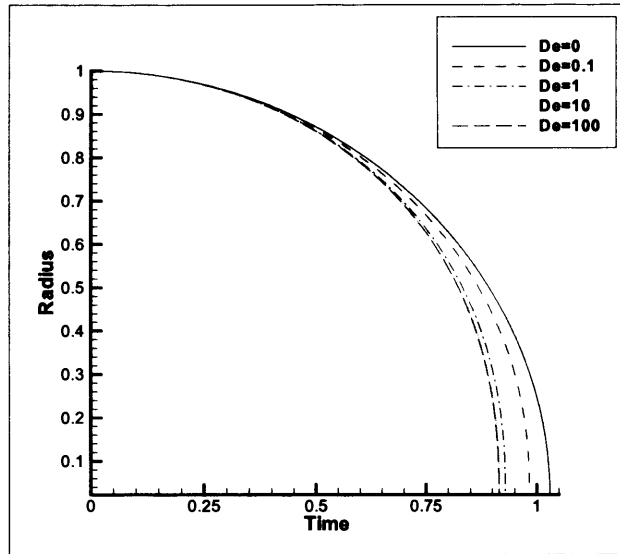
Figure 2.6: Variation of radius of spherical bubble with time for different De . Re = 10
