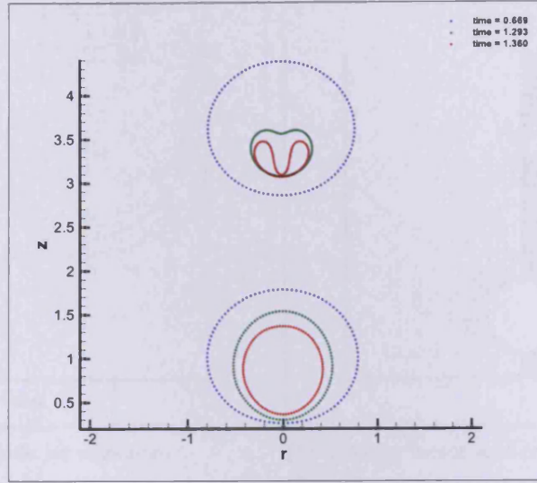
Figure 4.12: Bubble shapes for De = 2.5 , Re = 2 , h_1 = 1.0 , h_2 = 3.6 . Different colours indicate different instances in time.
