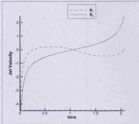
(a) North pole jet velocities.
