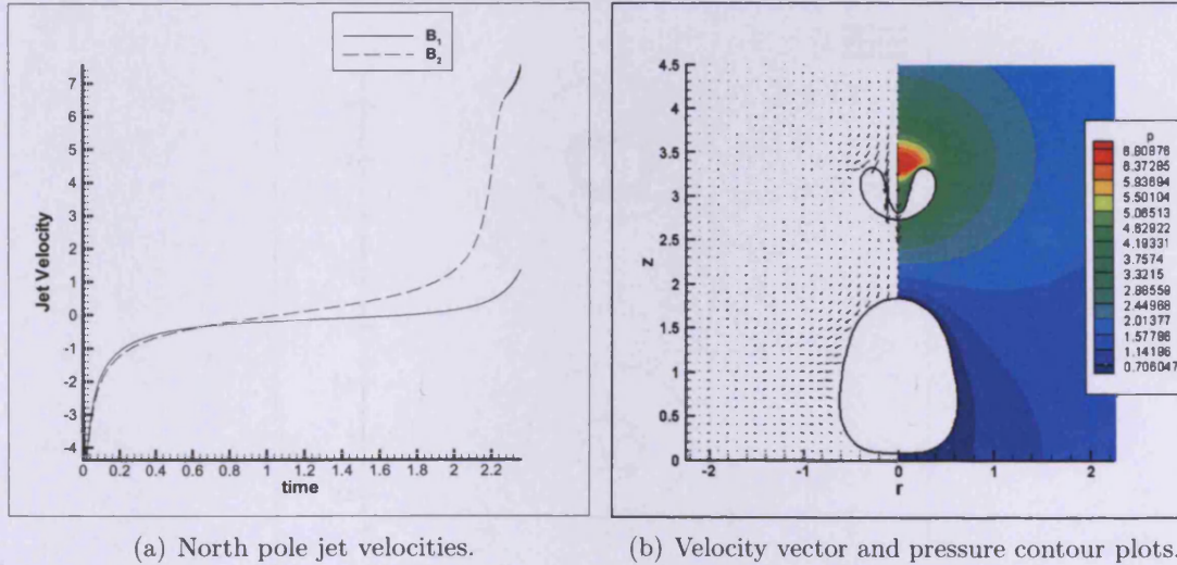
Figure 4.9: (a) North pole jet velocities, (b) velocity vector and pressure contour plots at t \approx 2.3 for De = 0 , Re = 100 , h_1 = 1.0 , h_2 = 3.6
