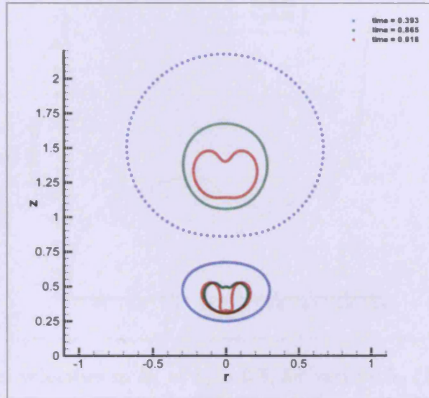
Figure 4.26: Bubble shapes for De = 1 , Re = 2 , h_1 = 0.5 , h_2 = 1.5 . Different colours indicate different instances in time.
