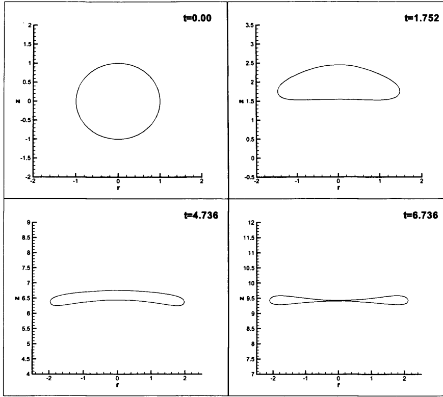
Figure 6.3: Bubble profiles at select times during ascent for Re = \infty and E\ddot{o} = 2.4 .
