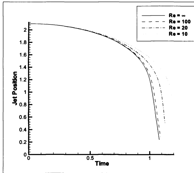
Figure 3.13: Position of jet point on z axis with time, at a distance of h = 1.1 , with varying Re .
