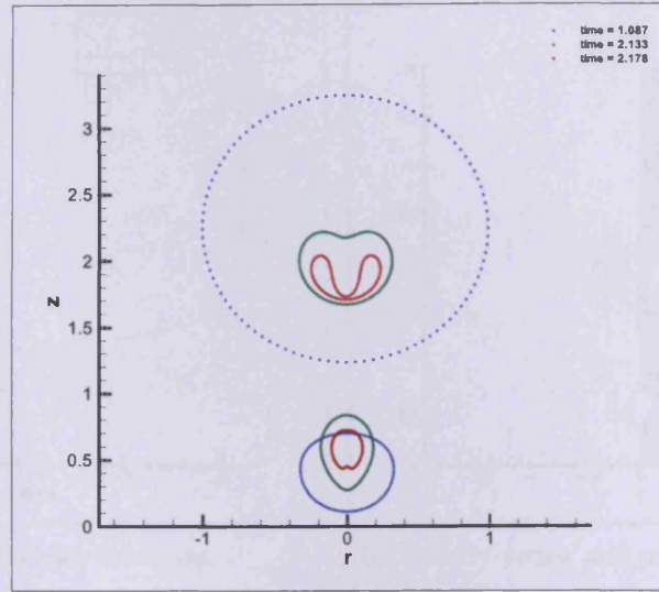
Figure 4.20: Bubble shapes for De = 0 , Re = 100 , h_1 = 0.5 , h_2 = 2.25 . Different colours indicate different instances in time.
