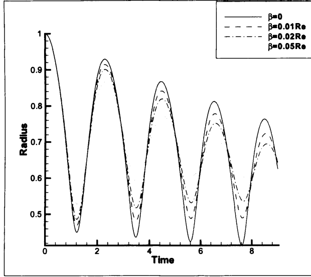
Figure 2.15: Variation of radius with time for a Jeffreys fluid, with De = 10
