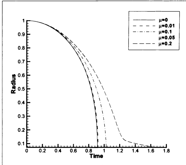
Figure 2.1: Numerical solution of the Rayleigh-Plesset equation for different viscosities.
