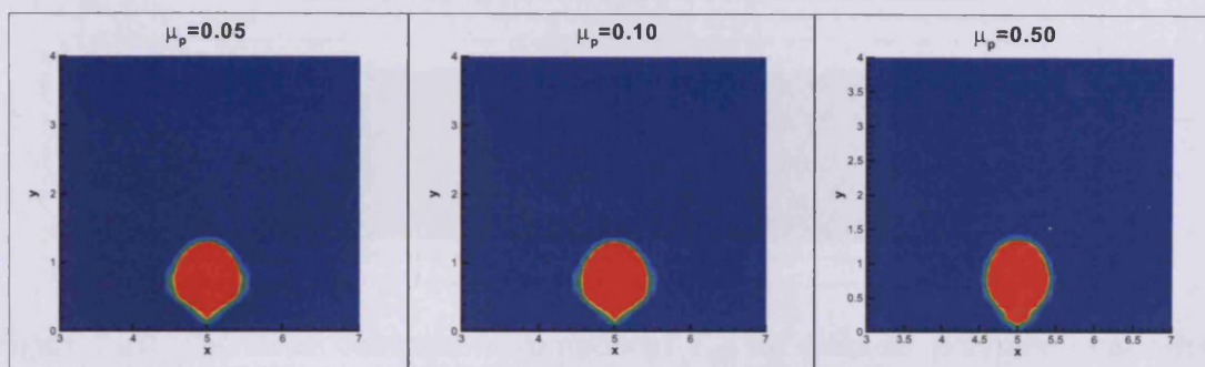
Figure 7.36: A plot of the colour function at t = 0.5 for different polymeric viscosities. The remaining parameters are We = \mu_s = 0.1 , h = 1.1 .
