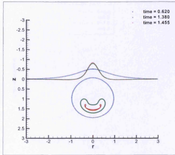
Figure 5.3: Bubble and free surface shapes for h = 1.0 . Different colours indicate different instances in time.
