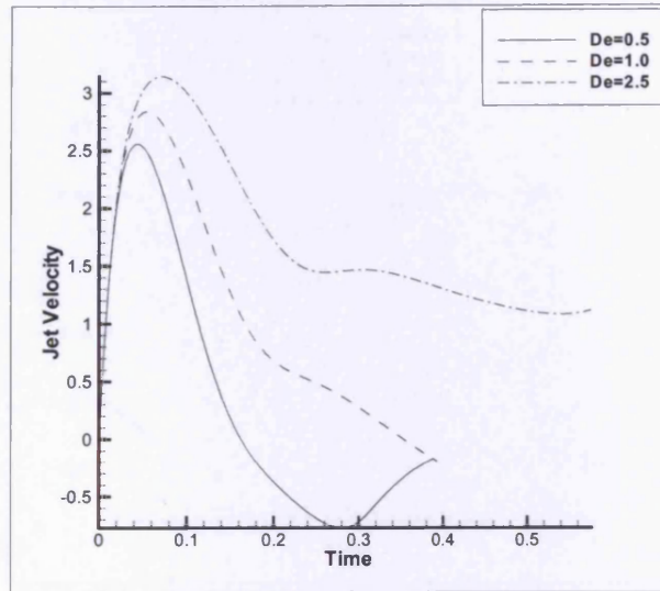
Figure 5.20: Free surface jet velocity for h = 0.5 with different De .
