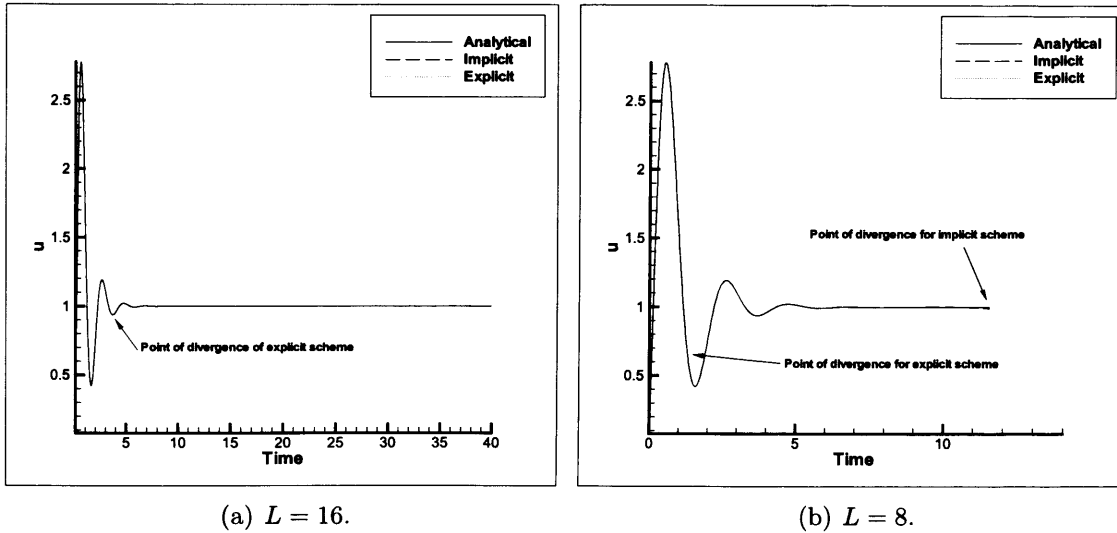
Figure 7.11: Analytical and numerical solutions of an Oldroyd B fluid in Poiseuille flow for different numerical schemes at different channel lengths L , with increased streamwise mesh refinement. The grid parameters are: N = 6 , \alpha = 3 , \beta = 1 .
