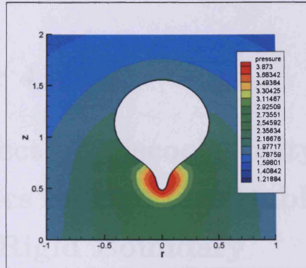
Figure 3.41: Pressure contours in the final stages of collapse ( t \approx 5.720 ), with h = 1.1 , Re = 0.2 , De = 5 .
