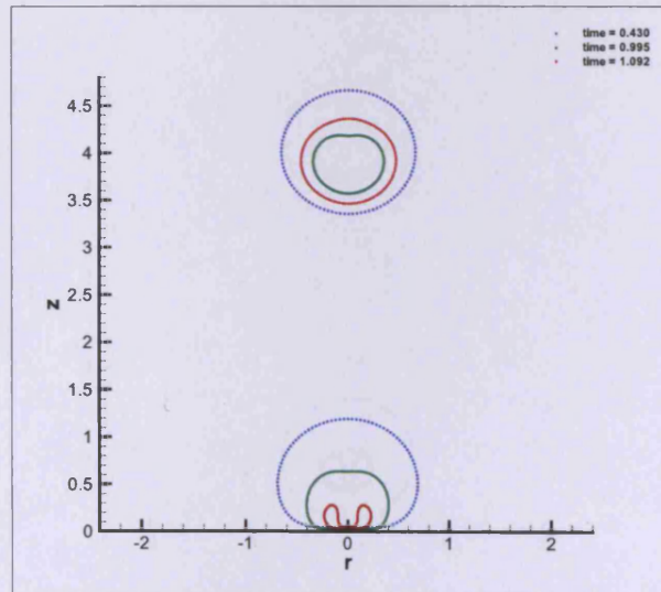
Figure 4.15: Bubble shapes for De = 1 , Re = 2 , h_1 = 0.5 , h_2 = 4.0 . Different colours indicate different instances in time.
