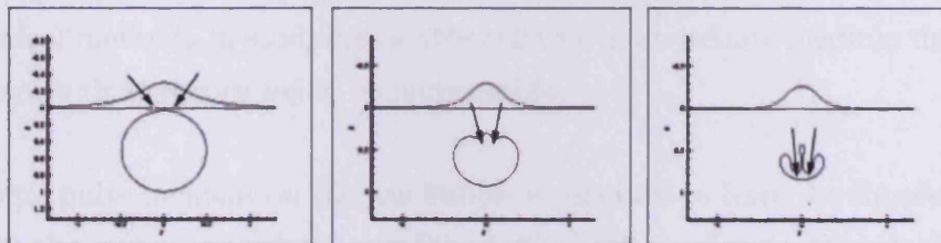
Figure 5.40: The instigation of a perturbation in the bubble surface by the free surface, resulting in annular jet formation.
