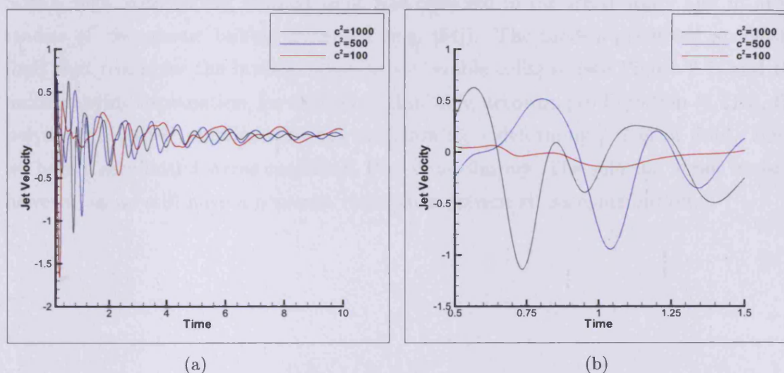
Figure 7.40: (a) Variation of jet velocity with time (after initial collapse) for different speeds of sound, with We = \mu_s = \mu_p = 0.1 , h = 1.1 . (b) Close up of the jet velocities, indicating the increase in the frequency of oscillations with increasing sound speed.
