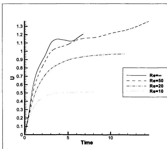
Figure 6.8: Evolution of the rise velocity for a selection of Reynolds numbers with E\ddot{o} = 2.4 .
