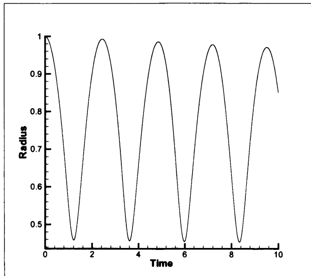
Figure 2.14: Near elastic oscillation of radius with time for De = 100 , Re = 0.01 )
