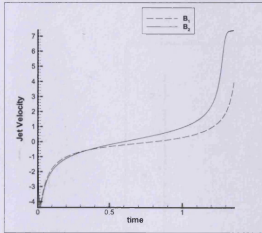
(a) North pole jet velocities.
