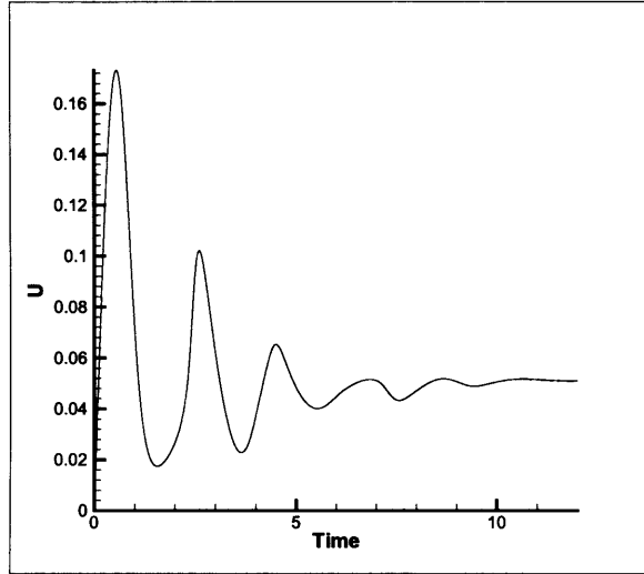
Figure 6.16: Variation of rise velocity U with time for Re = 1.18 and De = 0.93 .
