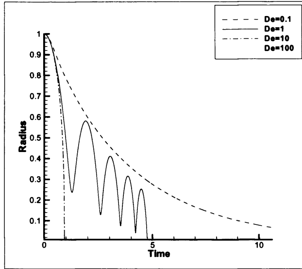
Figure 2.7: Variation of radius of spherical bubble with time for different De . Re = 1
