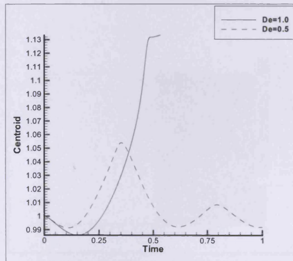
Figure 5.35: Bubble centroid position for h = 1.0 with different De .
