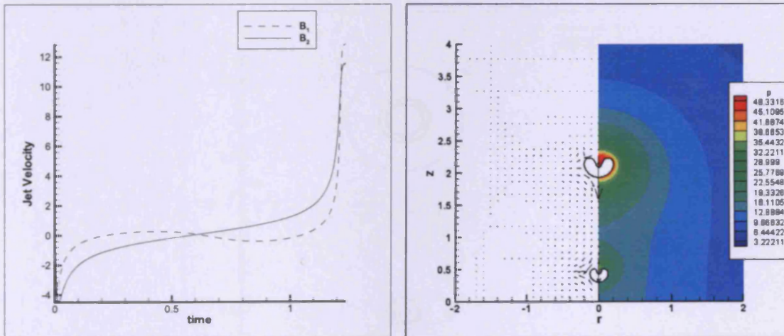
(a) North pole jet velocities.
