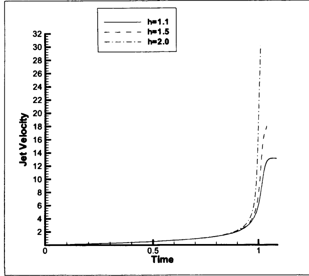
Figure 3.6: Jet velocities during collapse with Re = 100 for different initial distances from wall.
