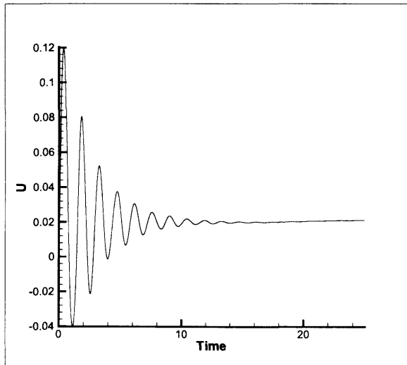
Figure 6.15: Variation of rise velocity U with time for Re = 0.5 , De = 1.25 .
