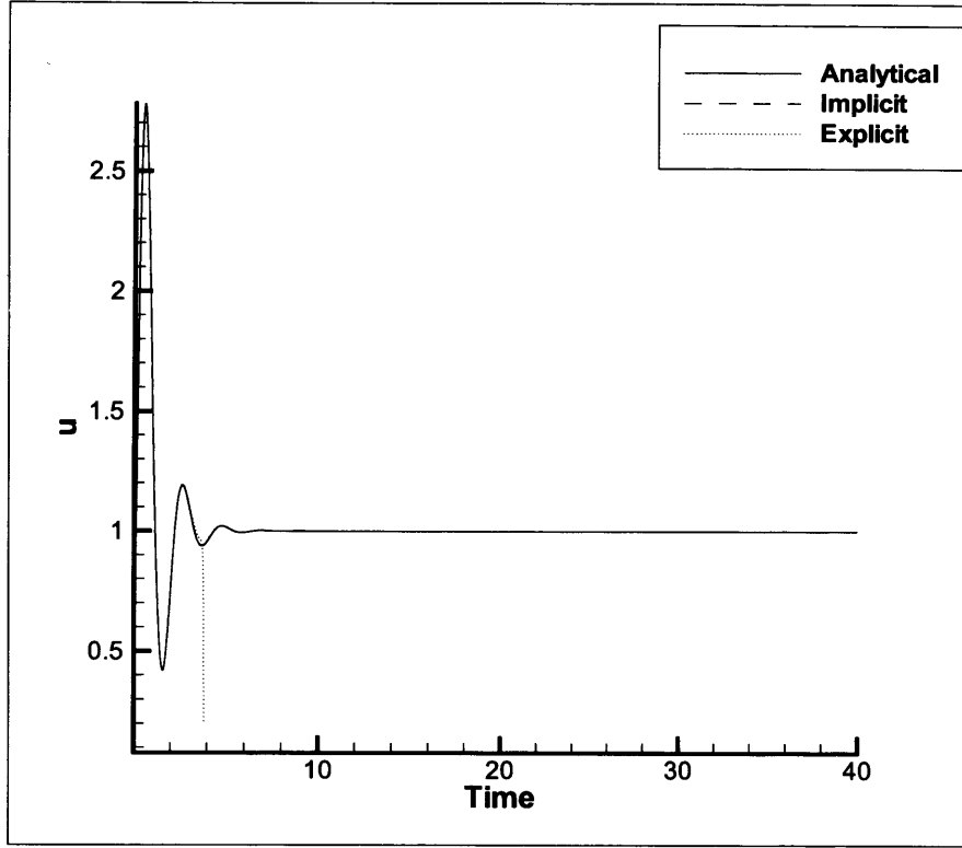
Figure 7.10: Analytical and numerical component of velocity u with time for an Oldroyd B fluid in Poiseuille flow. L = 8 , We = 1 , Re = 1 , \beta = 1/9 . The grid parameters are: N = 6 , \alpha = 1 , \beta = 1
