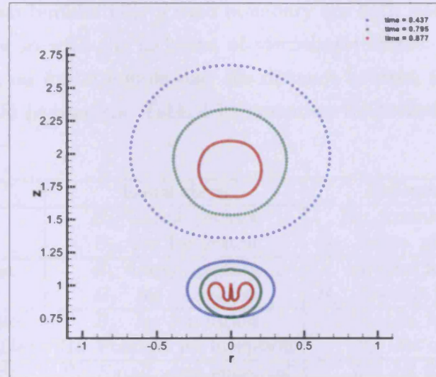
Figure 4.30: Bubble shapes for De = 1 , Re = 2 , h_1 = 1.0 , h_2 = 2.0 . Different colours indicate different instances in time.
