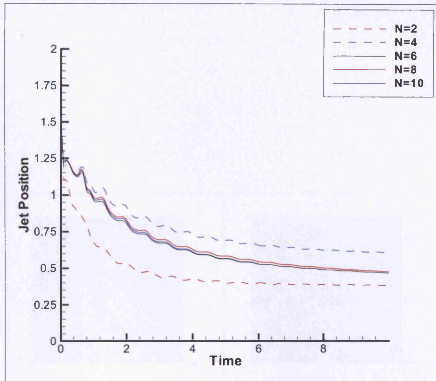
Figure 7.20: Dependence of the position of the jet on mesh refinement for \mu_s = 0.1 .
