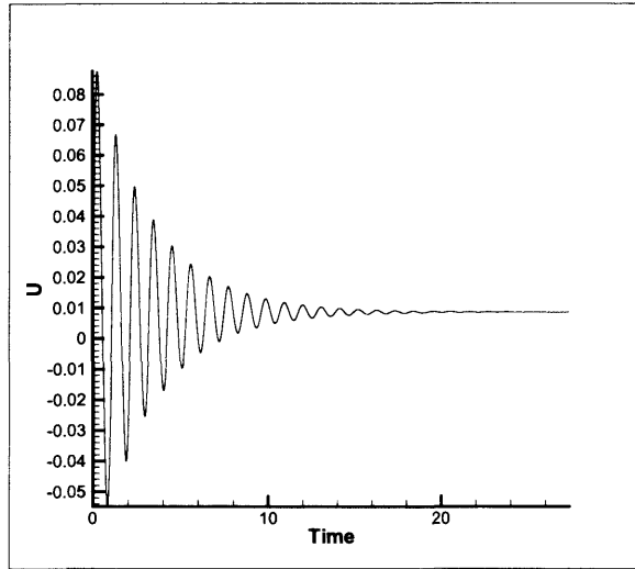
Figure 6.14: Variation of rise velocity U with time for Re = 0.21 , De = 1.66 .
