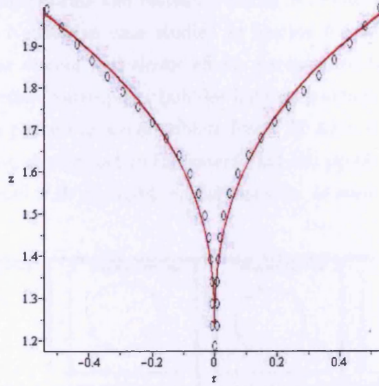
Figure 6.12: The numerical cusp (circles) from Fig. 6.10 and the associated least squares fit (red line).
