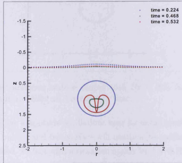
Figure 5.31: Bubble and free surface shapes with De = 1.0 , Re = 1.0 at h = 1.0 . Different colours indicate different instances in time.
