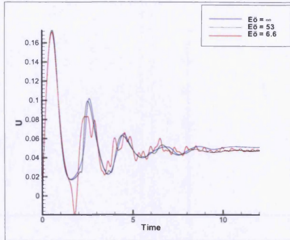
Figure 6.22: Rise velocity with time for a selection of Eötvös numbers with Re = 1.18 and De = 0.93
