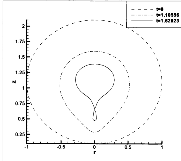
Figure 3.15: Bubble surface profiles at different stages of collapse at a distance h = 1.1 , Re = 1 , De = 1 .
