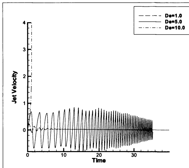
Figure 3.33: Jet velocities during collapse with varying De . Re = 0.2 and h = 2.0 .
