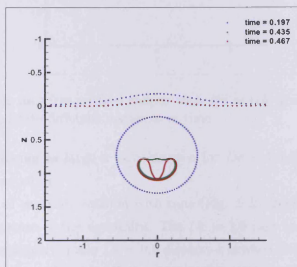
Figure 5.26: Bubble and free surface shapes with De = 1.0 , Re = 1.0 at h = 0.75 . Different colours indicate different instances in time.
