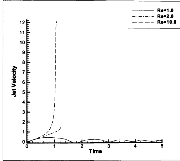
Figure 3.23: Jet velocities during collapse with varying Re . De = 0.5 and h = 1.1 .
