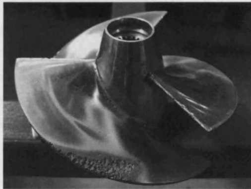
Figure 1.1: Cavitation damage on a propeller blade 1 .
