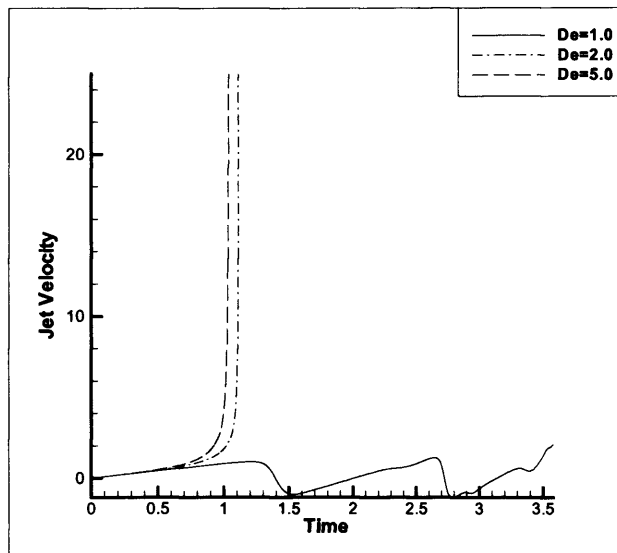
Figure 3.20: Jet velocities during collapse with varying De . Re = 1 and h = 2.0 .
