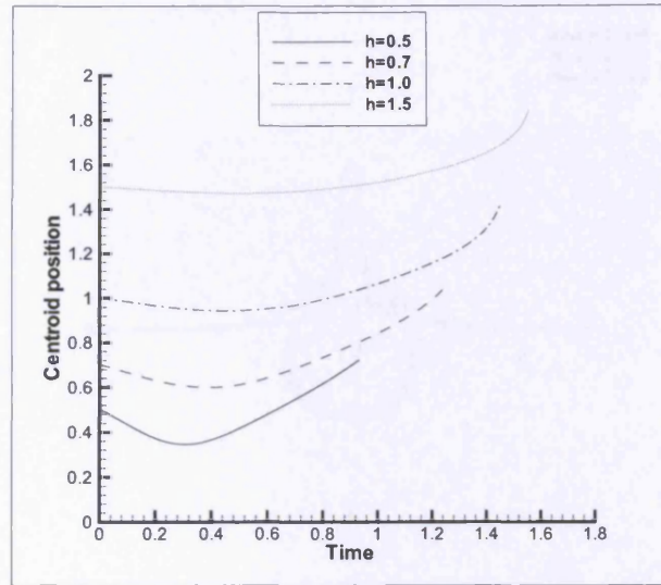
Figure 5.4: Bubble centroid positions for a range of values of h
