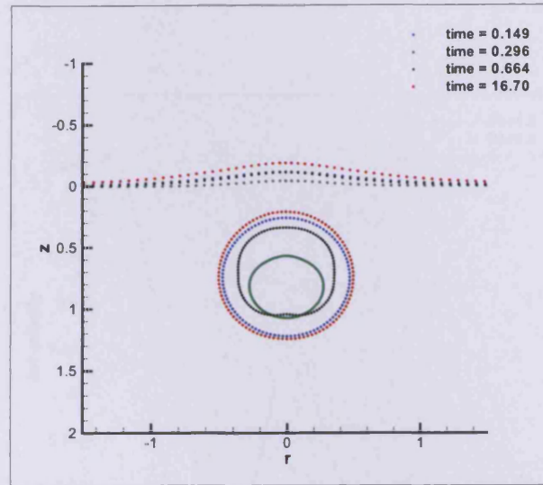
Figure 5.27: Bubble and free surface shapes with De = 0.5 , Re = 1.0 at h = 0.75 . Different colours indicate different instances in time.
