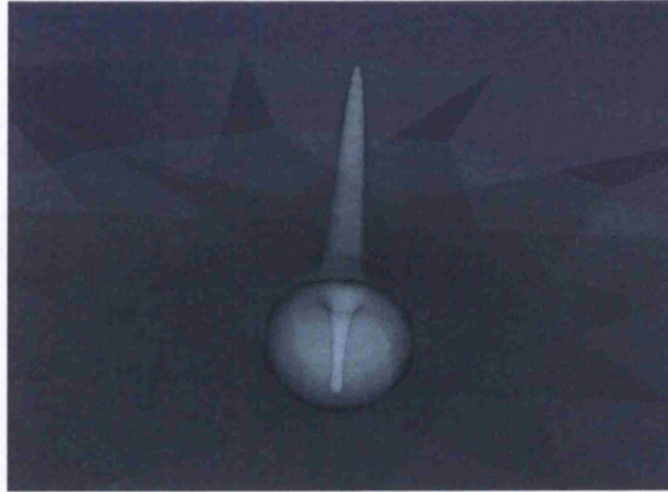
Figure 5.6: 3D visualisation of Fig. 5.5
