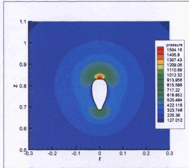
Figure 3.37: Pressure contours in the final stages of collapse, with h = 1.1 , Re = 10 , De = 0 .
