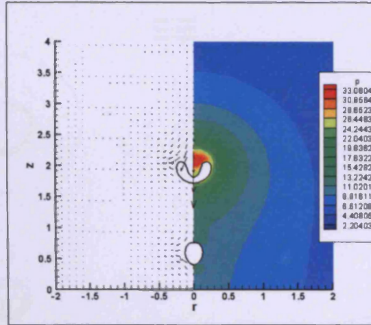
(b) Velocity vector and pressure contour plots at t \approx 2.17 .
