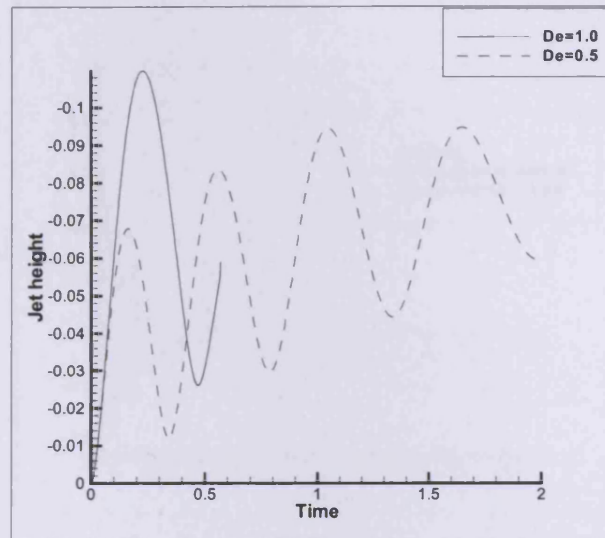
Figure 5.34: Free surface jet height for h = 1.0 with different De .
