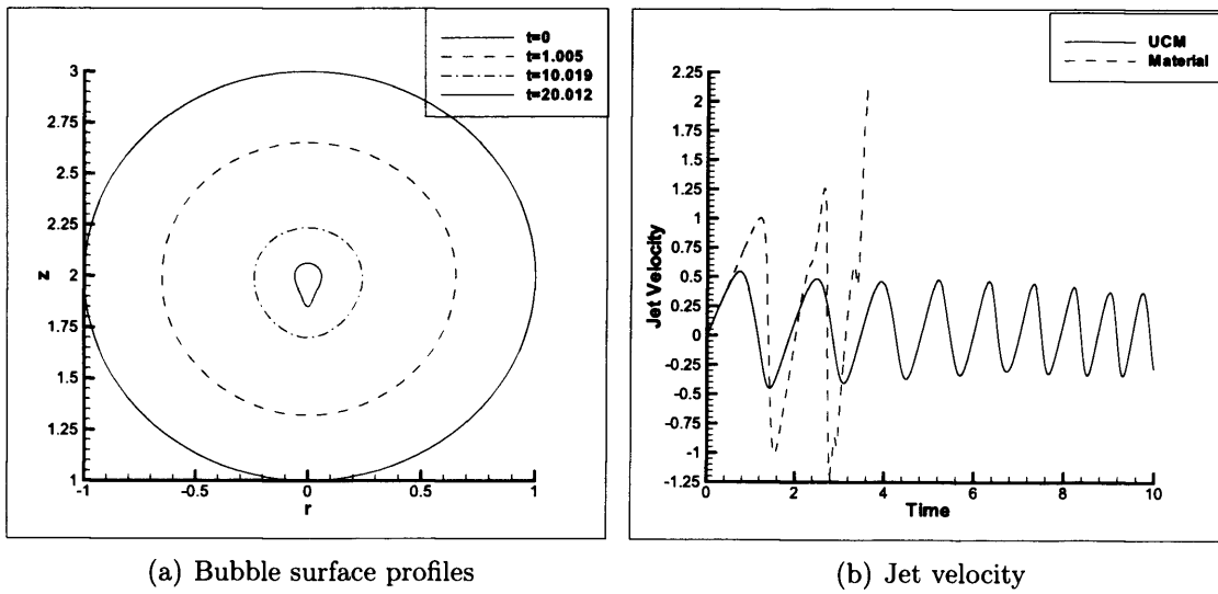
Figure 3.35: Bubble collapse near a wall using the UCM model. De = Re = 1 , h = 2
