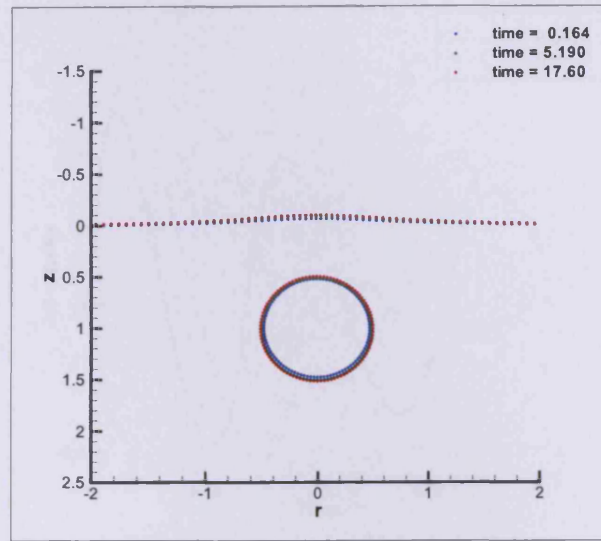
Figure 5.32: Bubble and free surface shapes with De = 0.5 , Re = 1.0 at h = 1.0 . Different colours indicate different instances in time.
