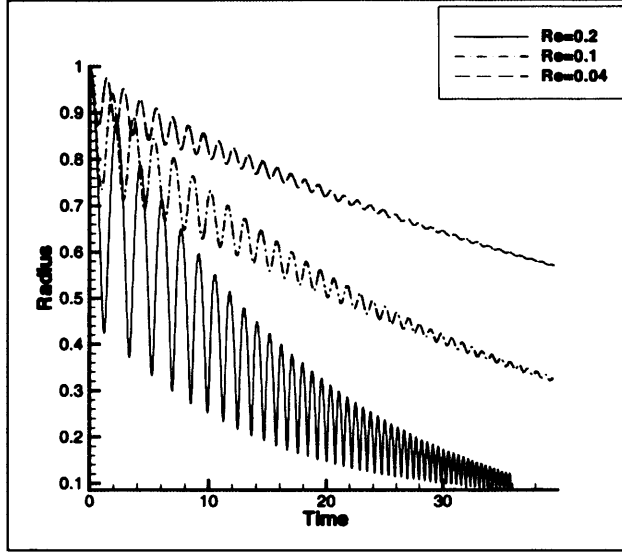
Figure 2.10: Variation of radius of spherical bubble with time for different Re . De = 5
