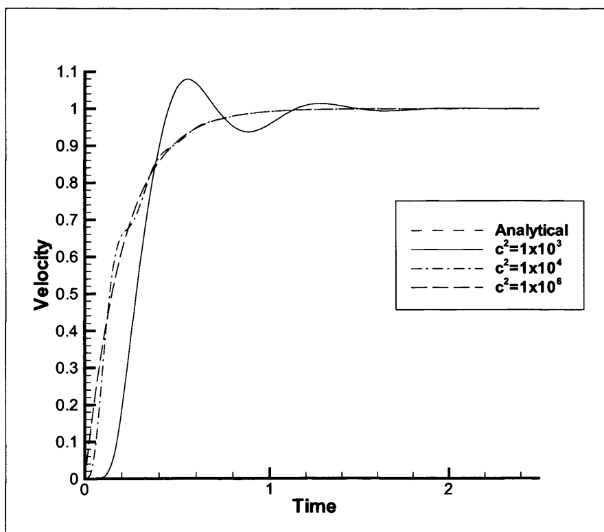
Figure 7.8: Incompressible analytical and compressible numerical solutions for velocity u for transient Poiseuille flow. By increasing the speed of sound the compressible solutions tend towards the incompressible solution. The channel length in this case is L = 10 .
