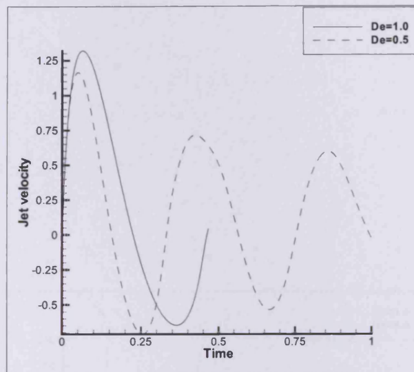
Figure 5.28: Free surface jet velocity for h = 0.75 with different De .
