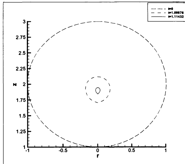
Figure 3.12: Bubble surface profiles at different stages of collapse at a distance h = 2.0 , Re = 10
