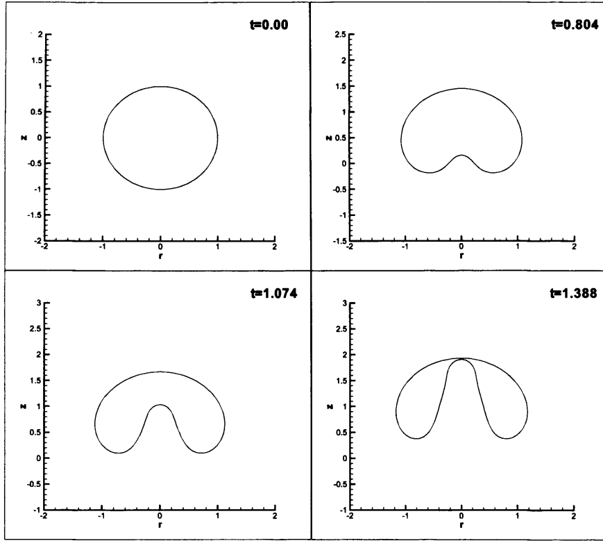
Figure 6.1: Bubble profiles at select times during ascent for Re = \infty and Eö = 106 .
