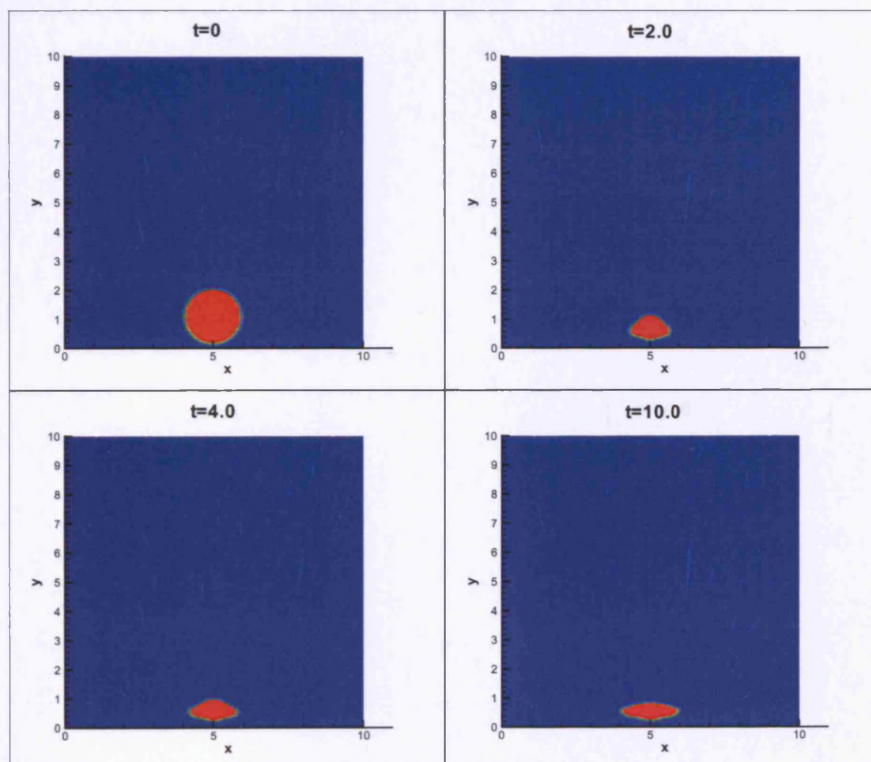
Figure 7.21: A plot of the colour function at different times, representing bubble collapse near a wall in a Newtonian fluid with \mu_s = 0.1 , h = 1.1 .
