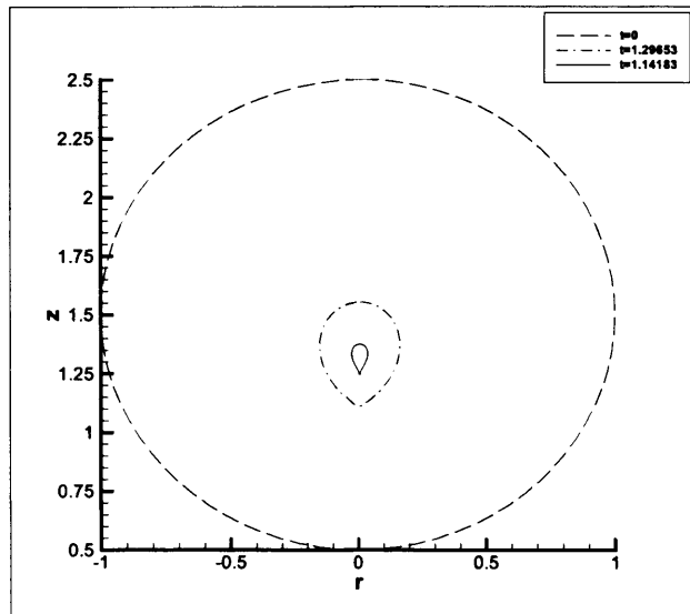
Figure 3.11: Bubble surface profiles at different stages of collapse at a distance h = 1.5 , Re = 10
