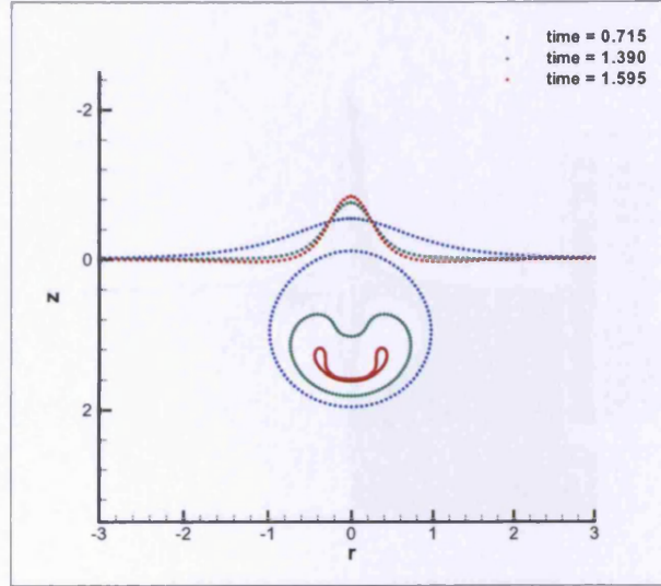
Figure 5.8: Bubble and free surface shapes for an inviscid fluid at h = 1.0 . Different colours indicate different instances in time.
