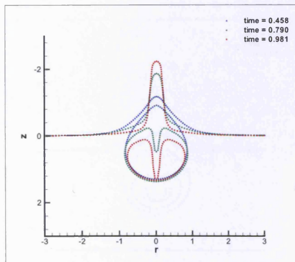
Figure 5.7: Bubble and free surface shapes with Re = 50 at h = 0.5 . Different colours indicate different instances in time.
