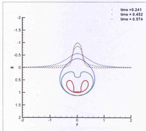
Figure 5.19: Bubble and free surface shapes with De = 2.5 , Re = 1.0 at h = 0.5 . Different colours indicate different instances in time.
