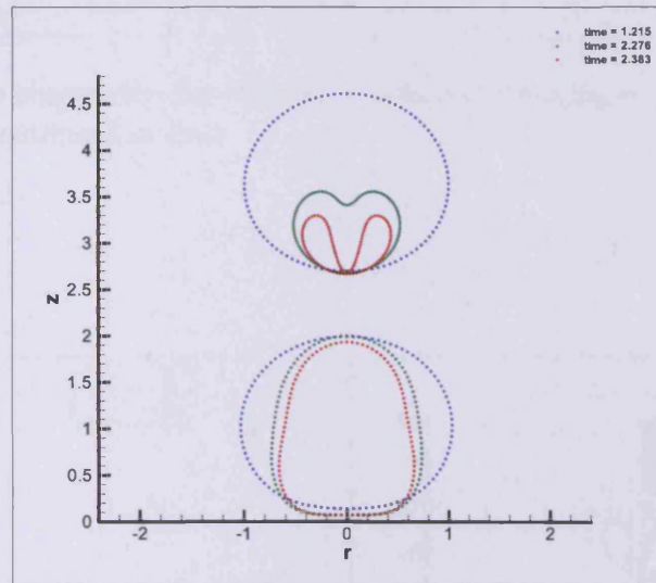
Figure 4.7: Bubble shapes for De = 0 , Re = \infty , h_1 = 1.0 , h_2 = 3.6 . Different colours indicate different instances in time.
