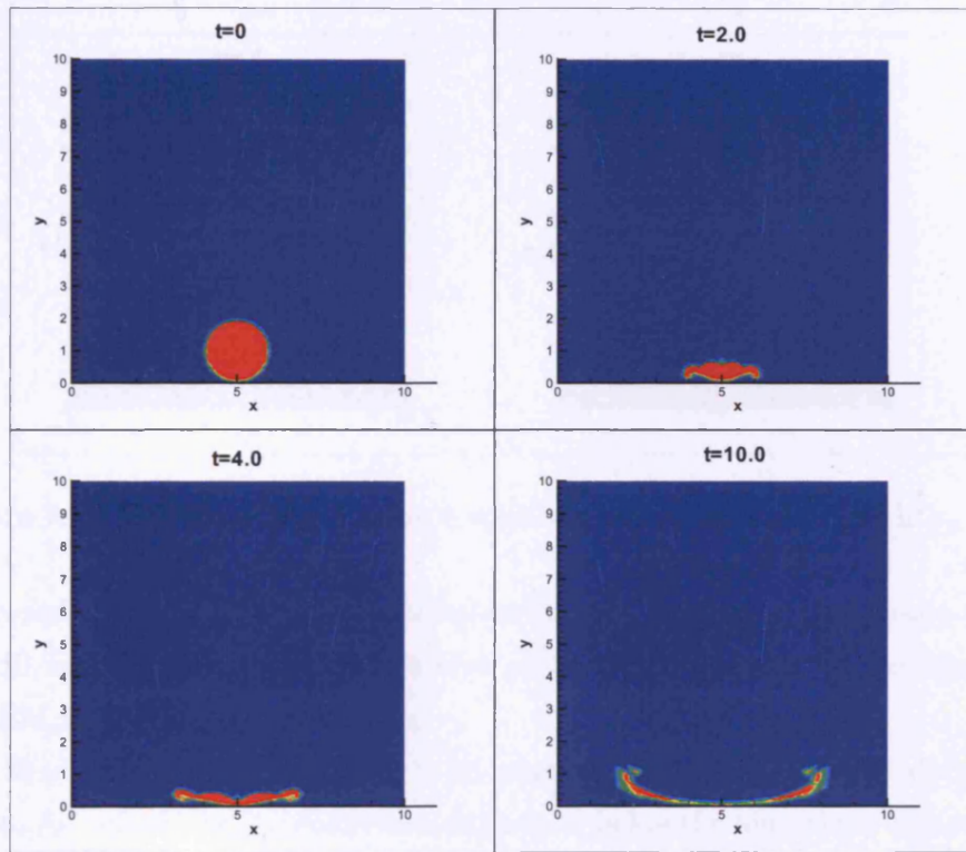
Figure 7.16: Bubble collapse near a wall in a Newtonian fluid with \mu_s = 1 \times 10^{-2} .
