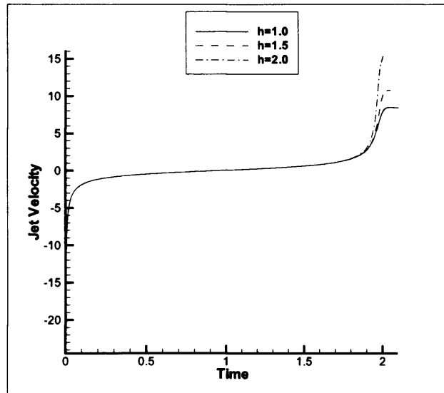
Figure 3.3: Jet velocities during growth and collapse of an inviscid bubble at varying initial distances from the rigid wall.
