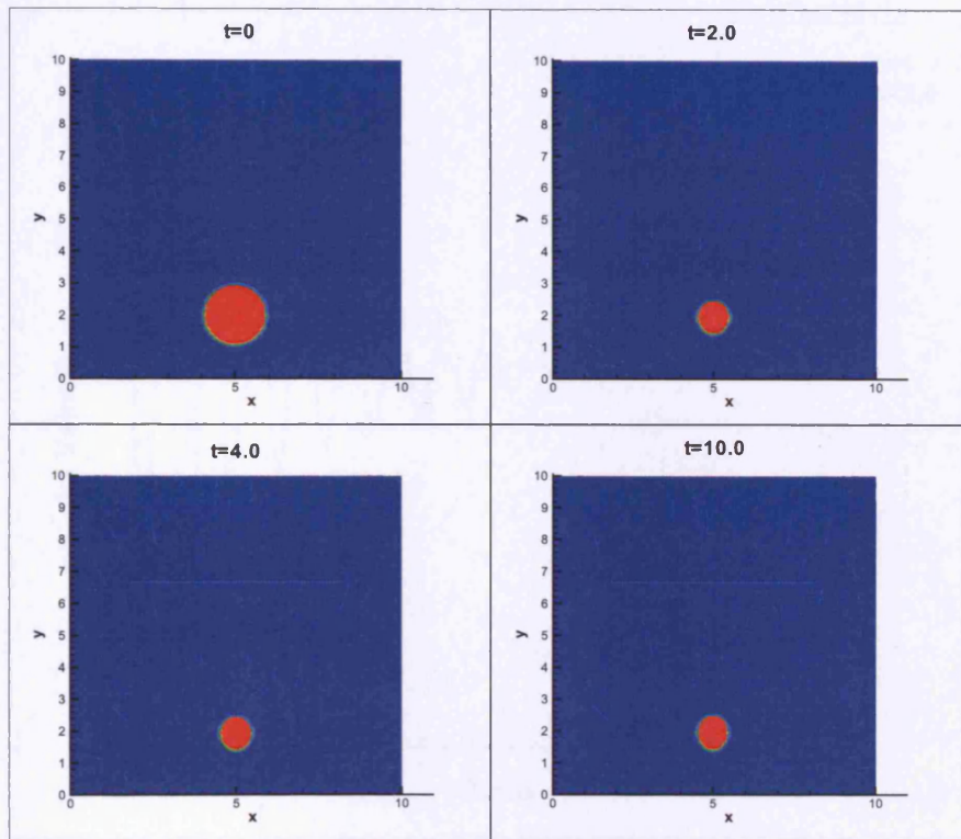
Figure 7.28: A plot of the colour function at different times, representing bubble collapse near a wall in a UCM fluid with \mu_p = 0.1 , We = 0.03 , h = 2.0 .
