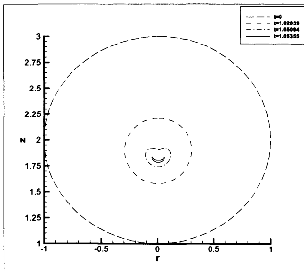
Figure 3.9: Bubble surface profiles at different stages of collapse at a distance h = 2.0 , Re = 20
