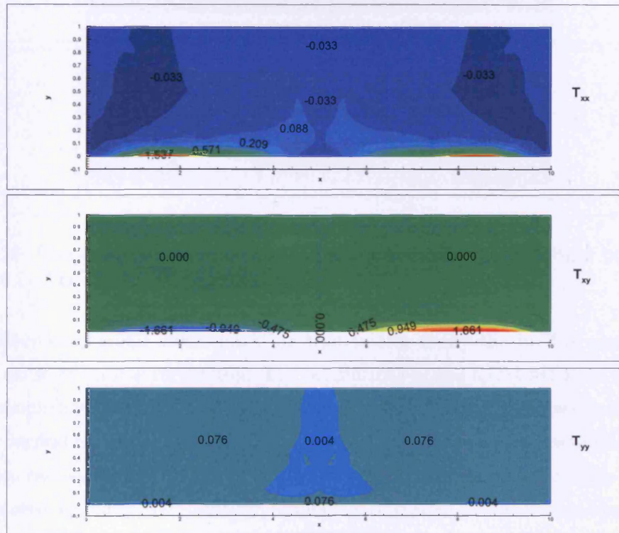
Figure 7.25: Contour plots of the extra stress components near the rigid boundary at time t = 0.5 . It is a UCM fluid with \mu_p = 0.1 , We = 0.03 , h = 1.1 .
