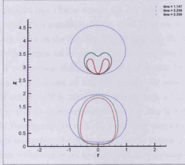
Figure 4.8: Bubble shapes for De = 0 , Re = 100 , h_1 = 1.0 , h_2 = 3.6 . Different colours indicate different instances in time.
