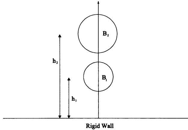
Figure 4.1: Schematic diagram detailing initial configuration.
