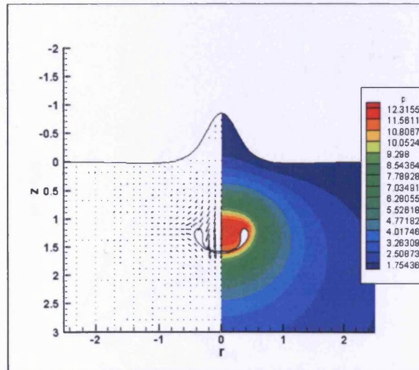
Figure 5.11: Pressure contours and velocity vectors at t = 1.595 for an inviscid fluid ( h = 1.0 ).
