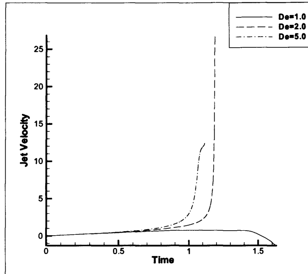
Figure 3.18: Jet velocities during collapse with varying De . Re = 1 and h = 1.1 .
