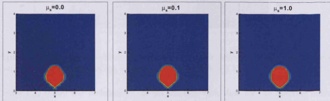
Figure 7.30: A plot of the colour function at t = 0.5 in an Oldroyd B fluid for different solvent viscosities \mu_s . The remaining parameters are \mu_p = 0.1 , We = 0.03 , h = 1.1 .
