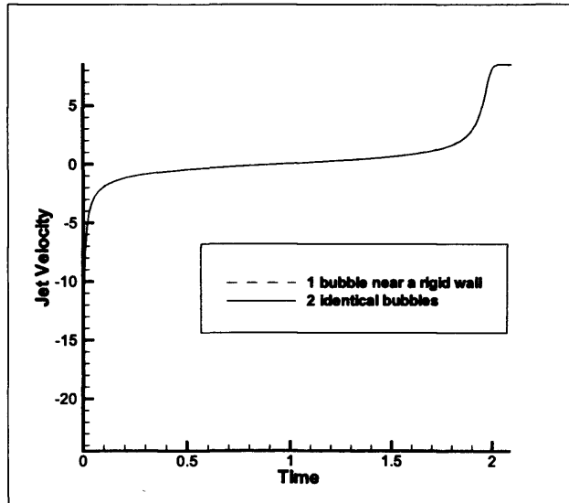
Figure 4.2: Jet velocities for a bubble near a rigid wall and one bubble near an identical bubble
