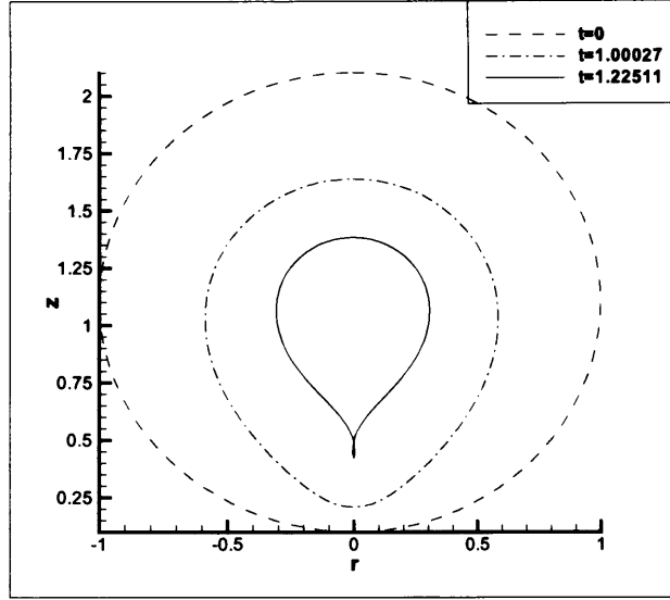
Figure 3.22: Bubble surface profiles at different stages of collapse at a distance h = 1.1 , Re = 2 , De = 0.5 .
