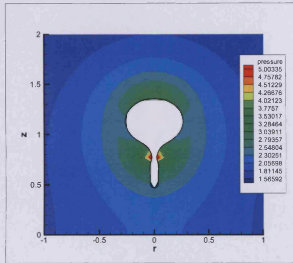
Figure 3.38: Pressure contours in the final stages of collapse ( t \approx 1.600 ), with h = 1.1 , Re = 1 , De = 1 .
