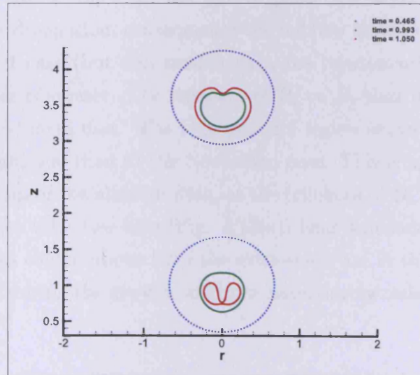
Figure 4.10: Bubble shapes for De = 1 , Re = 2 , h_1 = 1.0 , h_2 = 3.6 . Different colours indicate different instances in time.
