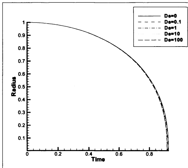
Figure 2.5: Variation of the radius of spherical bubble with time for different De . Re = 100 .
