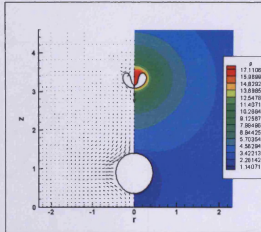
(b) Velocity vector and pressure contour plots at t \approx 1.35
