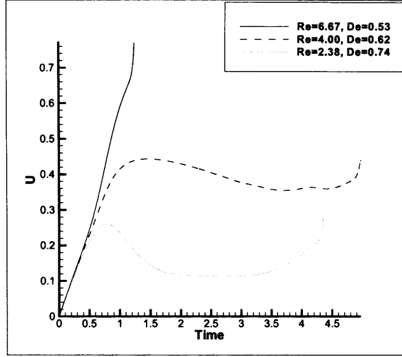
Figure 6.17: Variation of rise velocity U with time for a selection of Reynolds and Deborah numbers.
