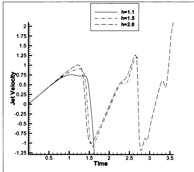
Figure 3.17: Jet velocities during collapse with varying height. Re = 1 and De = 1 .
