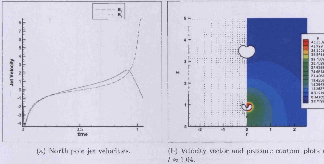
Figure 4.11: North pole jet velocities and velocity vector and pressure contour plots for De = 1 , Re = 2 , h_1 = 1.0 , h_2 = 3.6
