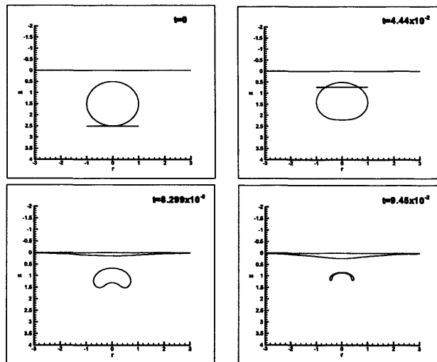
Figure 5.44: Bubble collapse under a shockwave, near a free surface, in a Newtonian inviscid fluid
