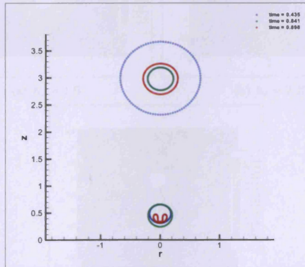
Figure 4.27: Bubble shapes for De = 1 , Re = 2 , h_1 = 0.5 , h_2 = 3.0 . Different colours indicate different instances in time.
