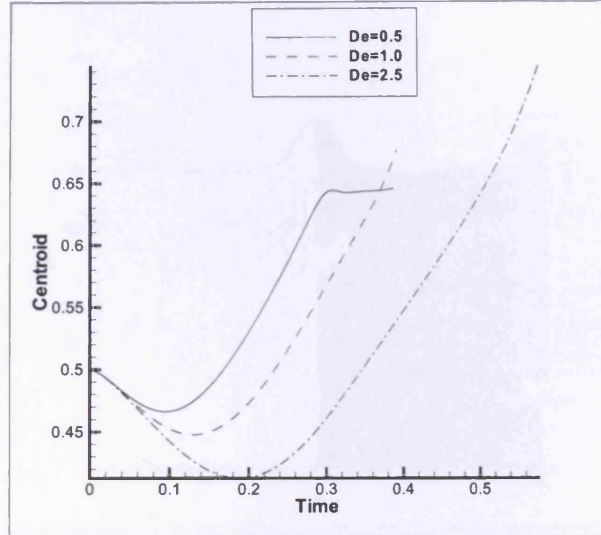
Figure 5.22: Bubble centroid position for h = 0.5 with different De .
