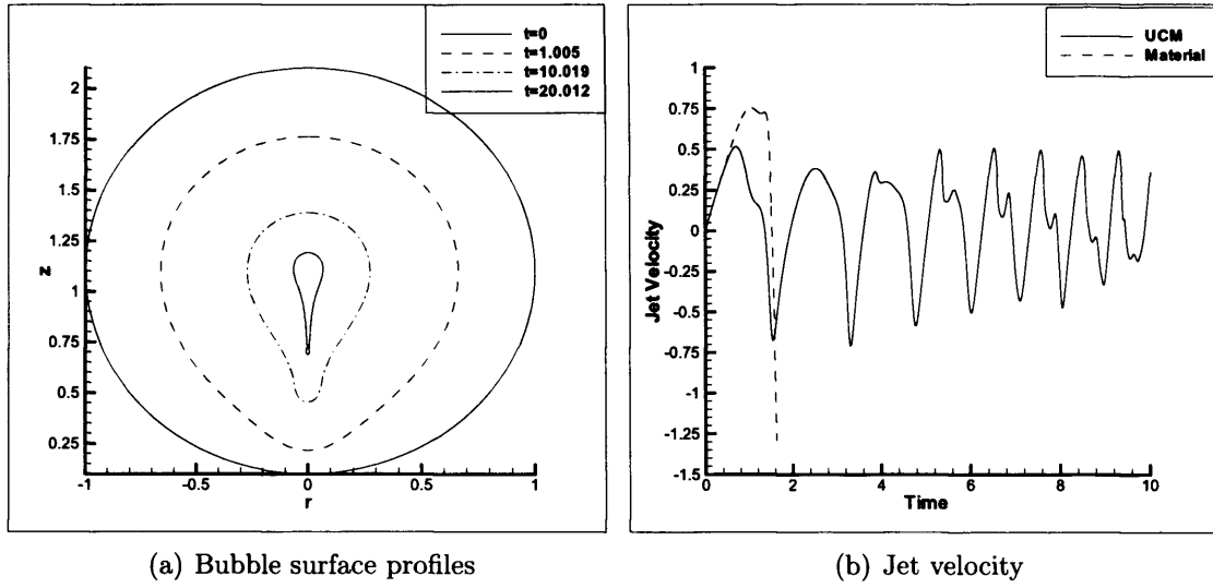
Figure 3.34: Bubble collapse near a wall using the UCM model. De = Re = 1 , h = 1.1
