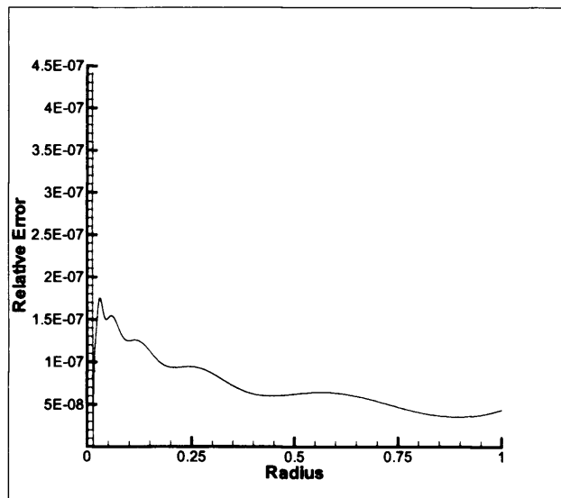
Figure 2.3: Relative error in the radial velocity of a spherical cavity in an inviscid fluid, varying with radius
