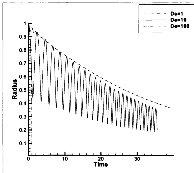
Figure 2.8: Variation of radius of spherical bubble with time for different De . Re = 0.1
