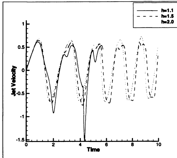
Figure 3.28: Jet velocities during collapse with varying height. Re = 0.2 and De = 5 .
