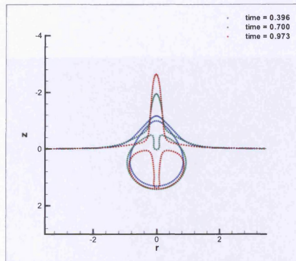
Figure 5.5: Bubble and free surface shapes for an inviscid fluid at h = 0.5 . Different colours indicate different instances in time.
