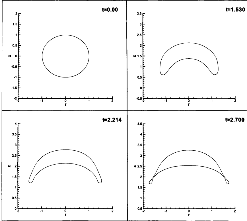
Figure 6.2: Bubble profiles at select times during ascent for Re = \infty and Eö = 6.6 .
