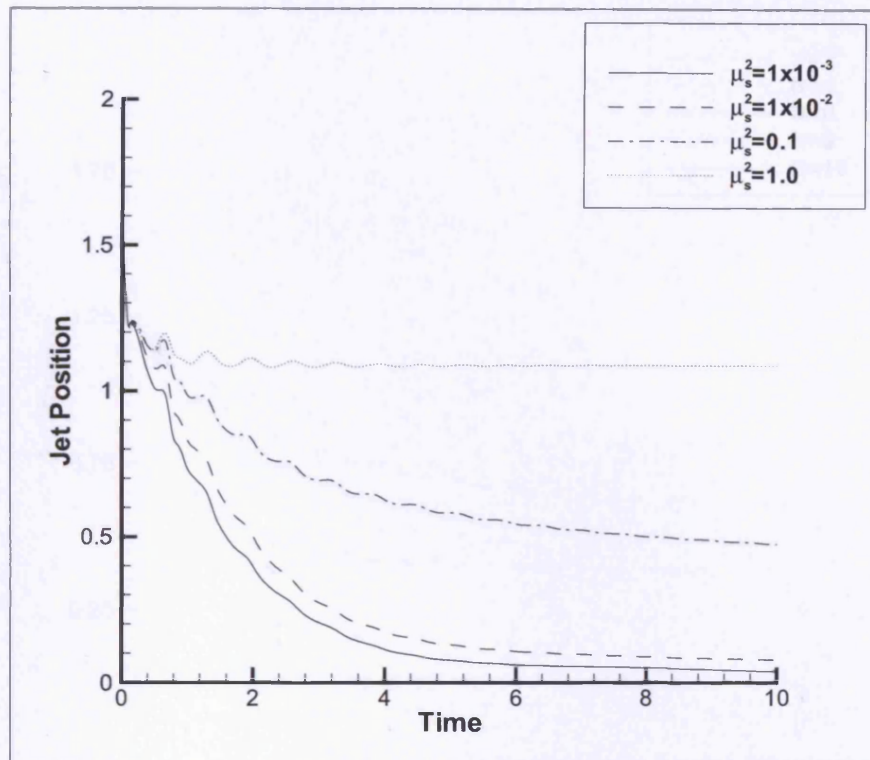
Figure 7.19: Position of jet with time for varying solvent viscosity \mu_s .
