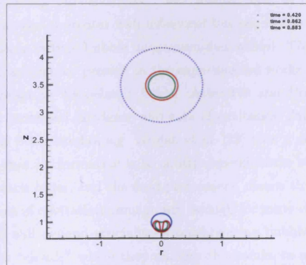
Figure 4.31: Bubble shapes for De = 1 , Re = 2 , h_1 = 1.0 , h_2 = 3.5 . Different colours indicate different instances in time.
