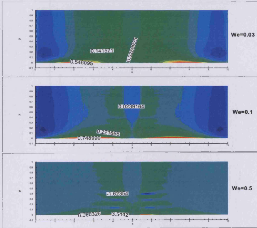
Figure 7.34: The stress contours of component T_{xx} for different Weissenberg numbers. The remaining parameters are \mu_p = \mu_s = 0.1 , h = 1.1 .
