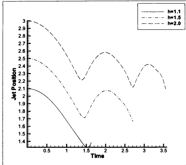
Figure 3.16: Position of jet point on z axis with time, Re = 1 , De = 1 , for varying height.
