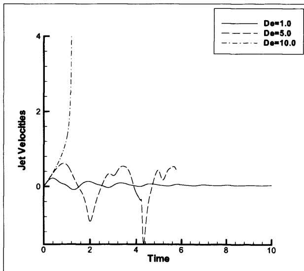
Figure 3.31: Jet velocities during collapse with varying De . Re = 0.2 and h = 1.1 .
