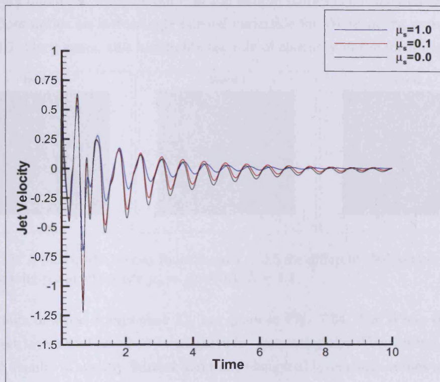
Figure 7.32: Variation of the jet velocity with time for different solvent viscosities, with \mu_p = 0.1 , We = 0.03 , and h = 1.1 .
