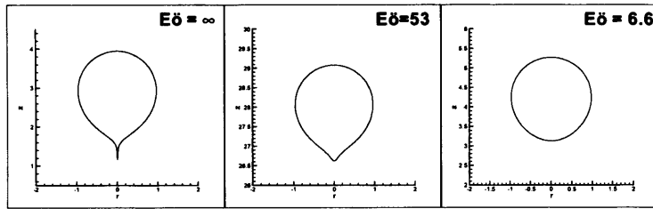
Figure 6.21: Terminal bubble profiles at varying Eötvös numbers, with Re = 1.18 and De = 0.93 .
