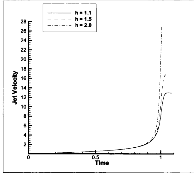
Figure 3.5: Jet velocities for the collapse of an inviscid bubble at different initial distances from a rigid wall.
