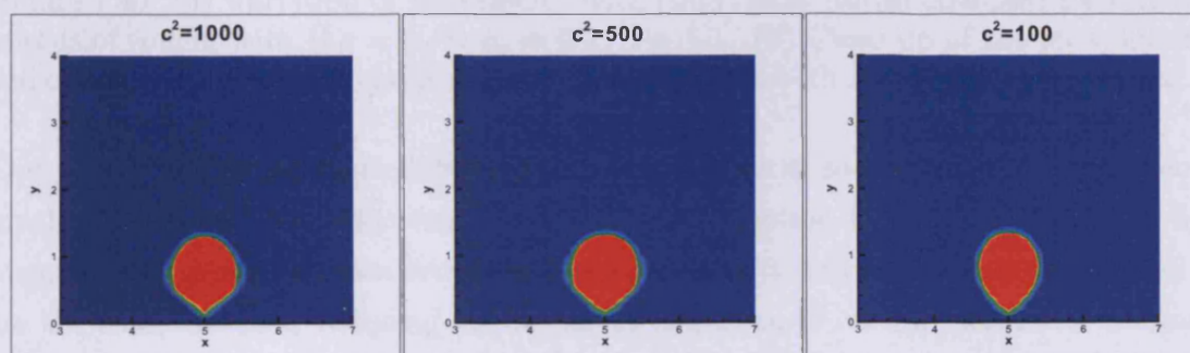
Figure 7.39: A plot of the colour function at t = 0.5 for different speeds of sound c^2 . The remaining parameters are We = \mu_s = \mu_p = 0.1 , h = 1.1 .
