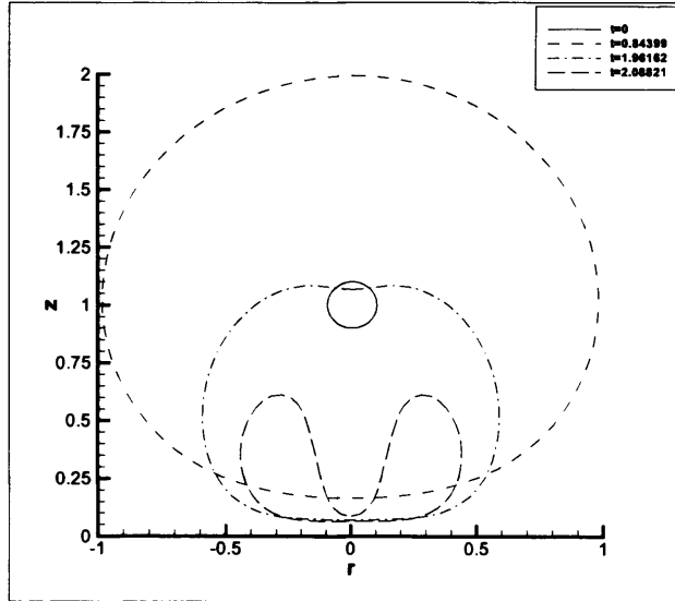
Figure 3.2: Bubble surface profiles at different stages of growth and collapse at an inception distance h = 1.0 from the boundary
