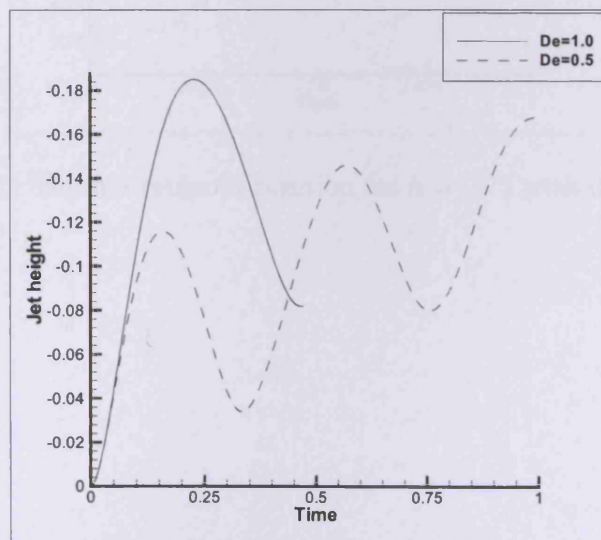
Figure 5.29: Free surface jet height for h = 0.75 with different De .
