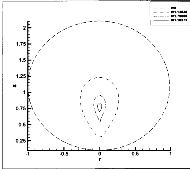
Figure 3.10: Bubble surface profiles at different stages of collapse at a distance h = 1.1 , Re = 10
