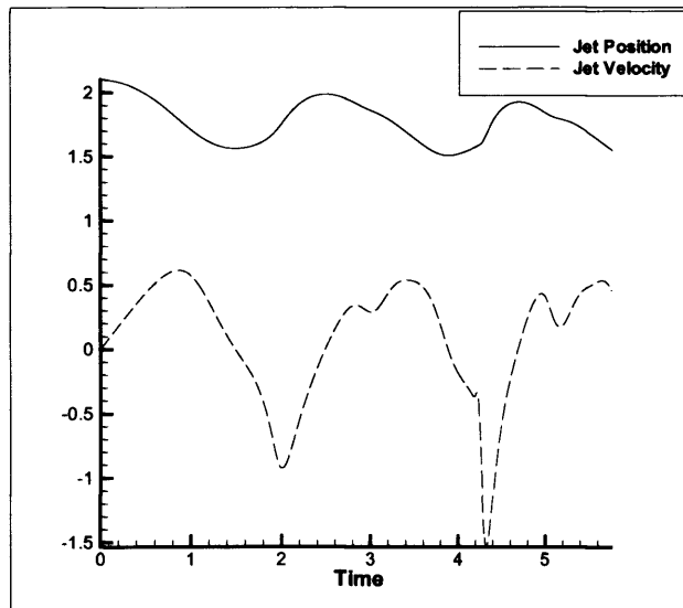
Figure 3.29: Comparison of jet positions and velocities, for h = 1.1 , Re = 0.2 and De = 5 .
