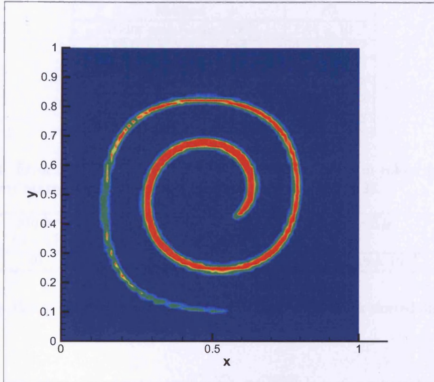
Figure 7.5: The colour function for the time reversed vortex problem at t = T_f/2 = 4.0 .
