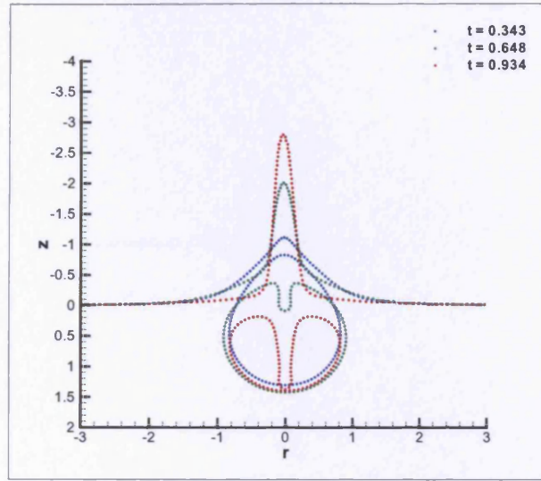
Figure 5.2: Bubble and free surface shapes for h = 0.5 . Different colours indicate different instances in time.
