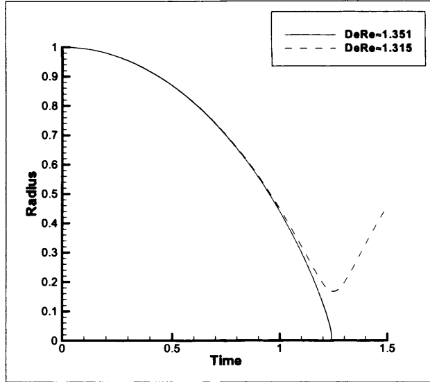
Figure 2.13: Variation of radius with time for DeRe above and below the rebound limit DeRe = 4/3 \approx 1.333 ( De = 100 ).
