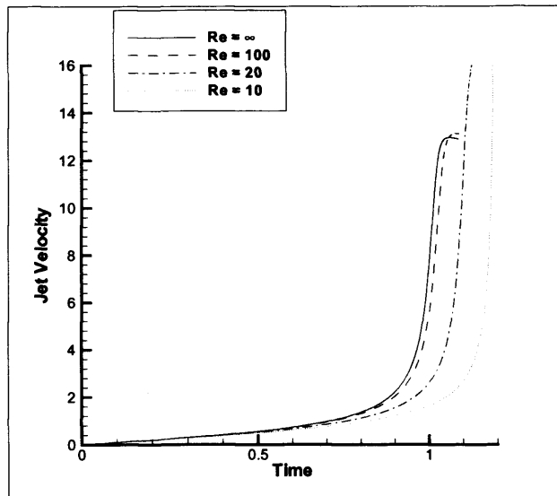
Figure 3.14: Jet velocities during collapse with varying Re . h = 1.1 .
