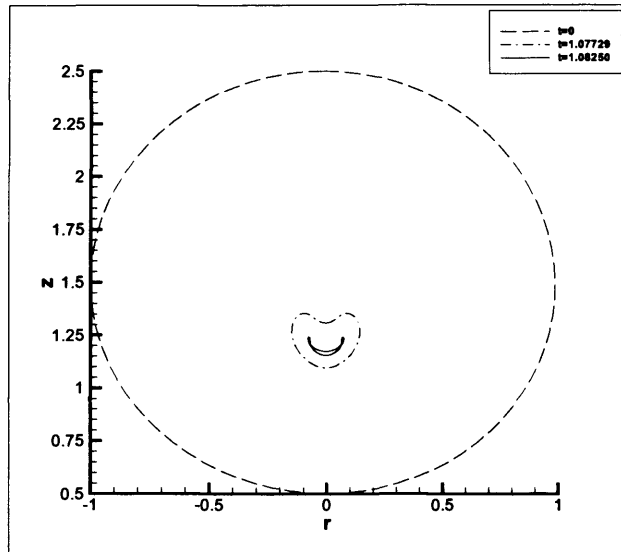
Figure 3.8: Bubble surface profiles at different stages of collapse at a distance h = 1.5 , Re = 20
