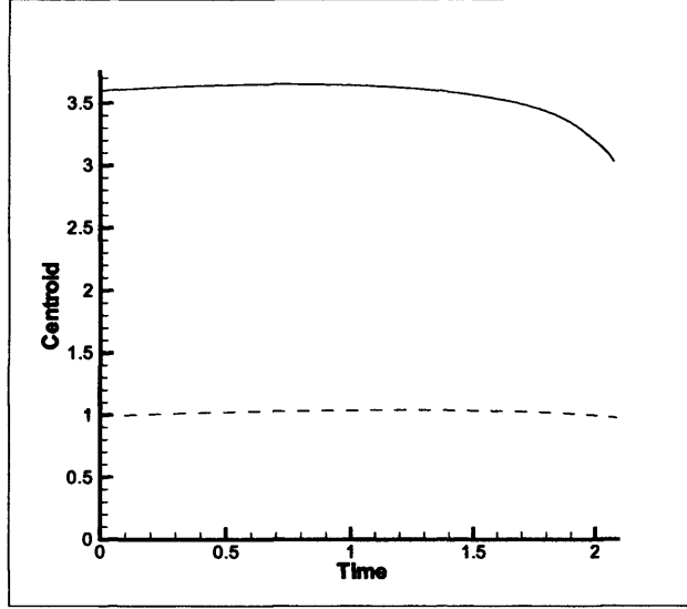
Figure 4.4: Evolution of bubble centroids. h_2 = 0.99 , h_1 = 3.60 , R_1 = 0.94
