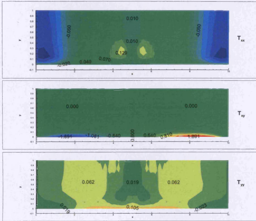
Figure 7.26: Contour plots of the extra stress components near the rigid boundary at time t = 0.5 . The fluid is Newtonian with \mu_s = 0.1 , h = 1.1 .
