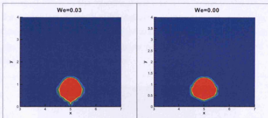
Figure 7.24: A plot of the colour functions in a UCM fluid (left) and Newtonian fluid (right) at time t = 0.5 .
