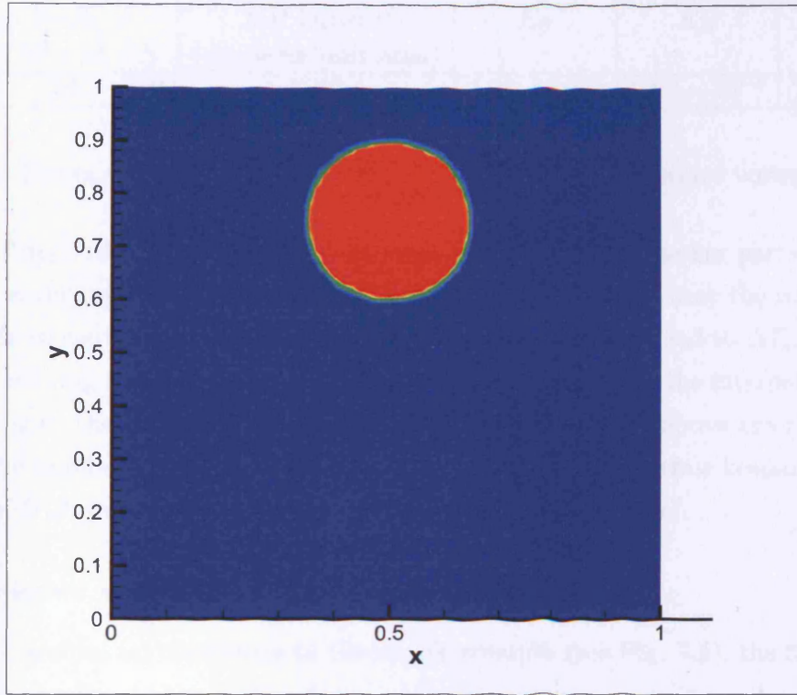
Figure 7.4: The initial colour function for the simple rotation and vortex test problems.
