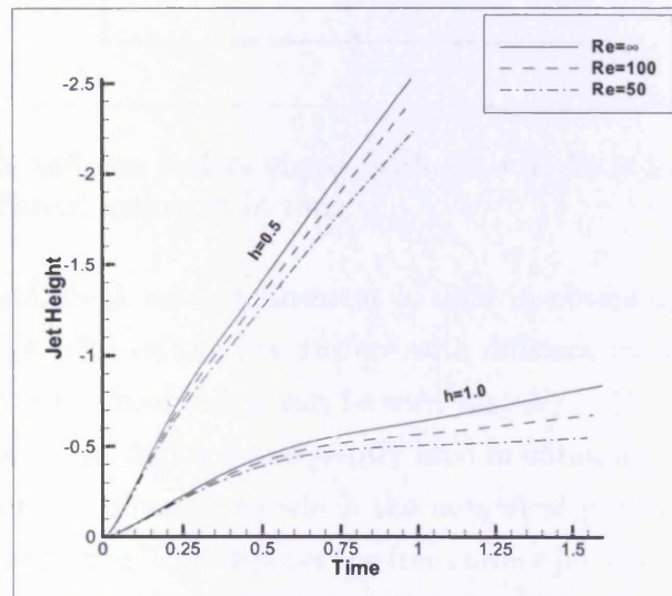
Figure 5.13: Jet height varying with time for different Reynolds number at h = 0.5 and h = 1.0 .
