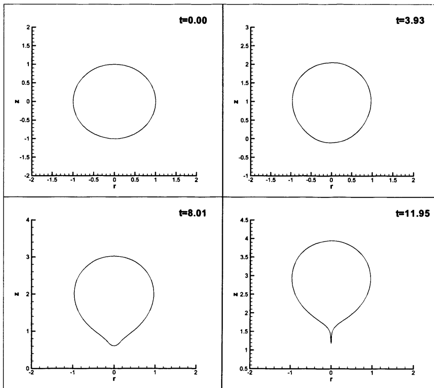
Figure 6.10: Bubble profiles at select times during ascent for De = 0.93 , Re = 1.18
