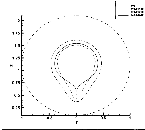
Figure 3.24: Bubble surface profiles at different stages of collapse at a distance h = 1.1 , Re = 0.2 , De = 5 .
