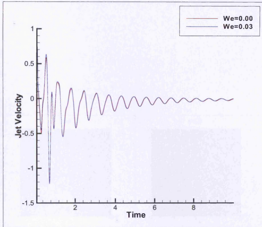
Figure 7.27: Variation of jet velocity with time (after the initial collapse) in a Newtonian and UCM fluid, \mu_p = 0.1 , h = 1.1 .
