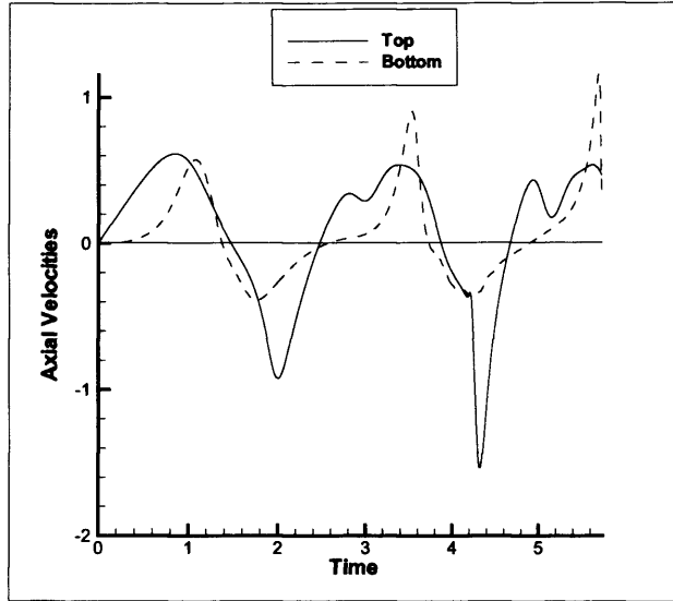
Figure 3.30: Comparison of North and South pole velocities, for h = 1.1 , Re = 0.2 and De = 5 .
