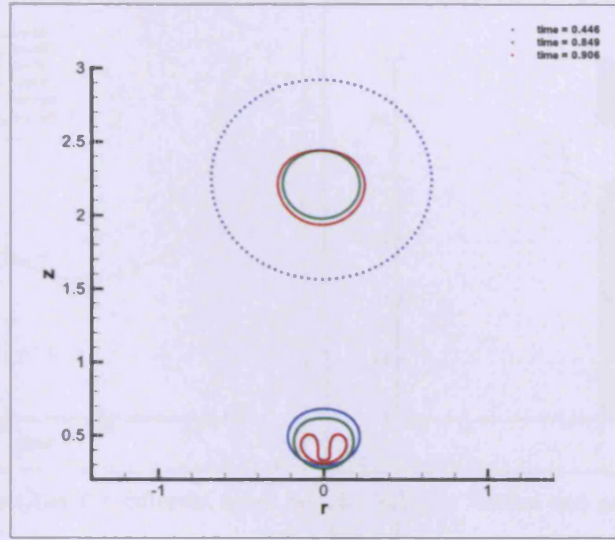
Figure 4.22: Bubble shapes for De = 1 , Re = 2 , h_1 = 0.5 , h_2 = 2.25 . Different colours indicate different instances in time.
