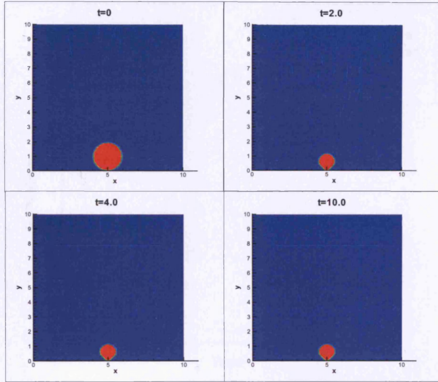
Figure 7.18: Bubble collapse near a wall in a Newtonian fluid with \mu_s = 1.0 .
