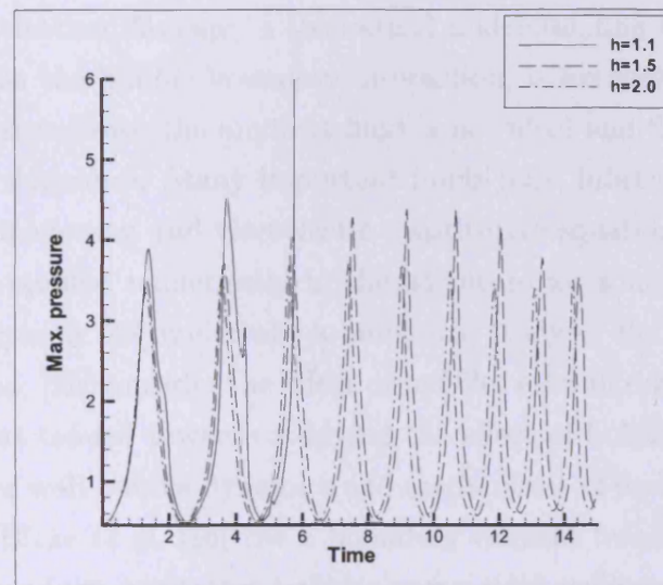
Figure 3.42: Variation of maximum pressure with time at different heights: Re = 0.2 , De = 5 .
