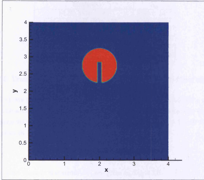
Figure 7.6: The initial colour function for the Zalesak slotted disk rotation problem.
