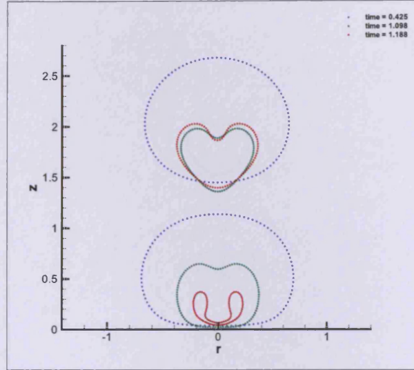
Figure 4.14: Bubble shapes for De = 1 , Re = 2 , h_1 = 0.5 , h_2 = 2.0 . Different colours indicate different instances in time.
