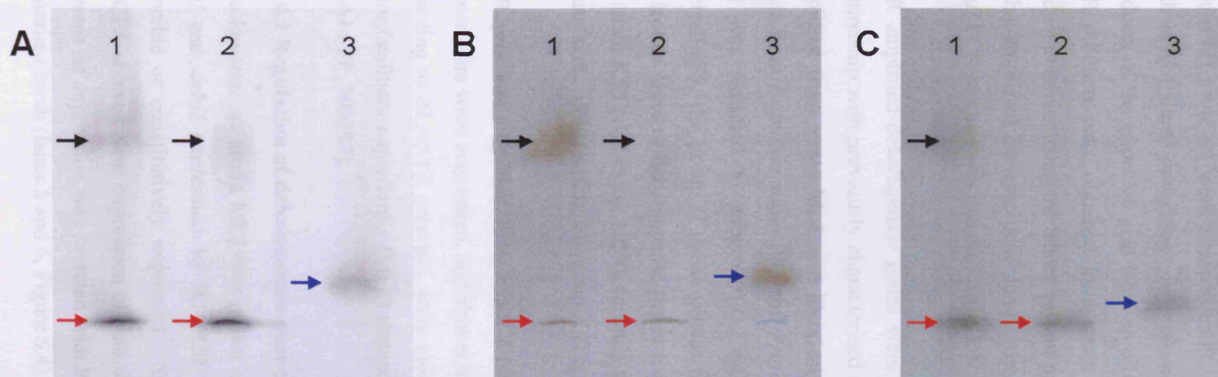
Figure 6.2 Native PAGE of cell free extracts incubated with various substrates: (A) MCA; (B) D-2MCPA; or (C) L-2MCPA, to show dehalogenase activity. Lane numbers: (1) P. putida PP3. (2) Pseudomonas sp. ML1. (3) Rhodococcus sp. R1. Black arrows mark the position of DehI PP3 for P. putida PP3 and a putative D-specific DehI (DehI ML1 ) from strain ML1. Red arrows mark the position of DehII PP3 and a putative DehII (DehII ML1 ) from strain ML1. Blue arrows represent a putative D-/L- dechlorinating dehalogenase (Deh R1 ) from strain R1.
