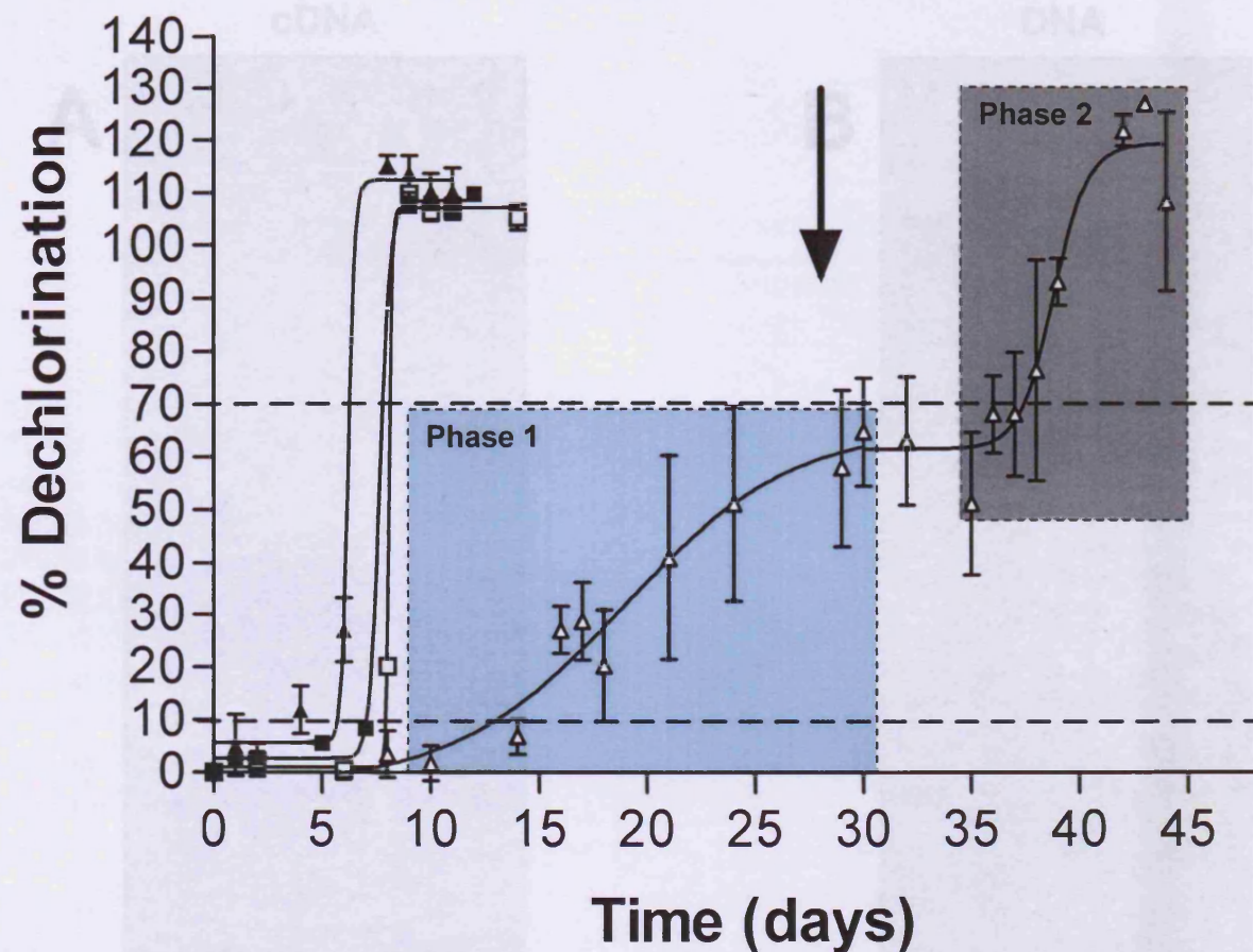
Figure 3.1 Degradation kinetics of \alpha HAs inoculated with 30 mg/l fresh (closed symbols) or lyophilised (open symbols) activated sludge: DCA (■/□); 2MCPA (▲/△). Broken horizontal lines represent biodegradation start point (10%) and pass level (70%), and the arrow indicates the 28 day cut-off for a RBT pass according to OECD guidelines. Error bars represent the standard error of the mean ( n = 3 ).
