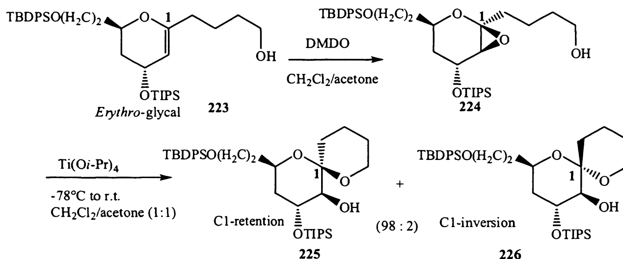
Scheme 17. Strategy for stereocontrolled synthesis of spiroketals via epoxide opening spirocyclisations with retention ( 225 ) or inversion ( 226 ) of configuration at the anomeric carbon.
