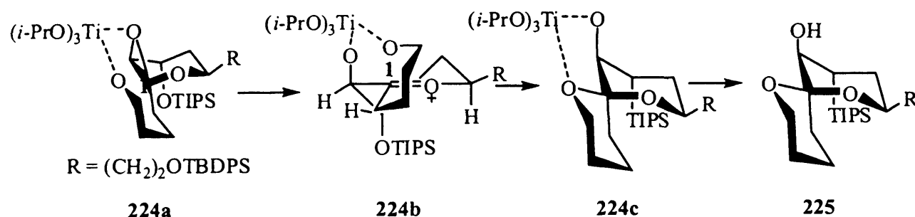
Scheme 18. Proposed tethered mechanism for kinetic spirocyclisation with retention of configuration at anomeric carbon (C-1).
