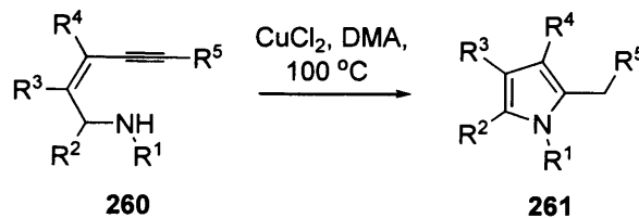
Scheme 82: Gabriele and coworkers synthesis of C-3 substituted pyrroles.
