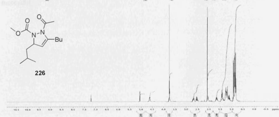
Figure 11: 1 H-NMR comparison of starting hydrazine 225 at 300 k and 367 k and of dihydropyrazole 226 at 300 k.
