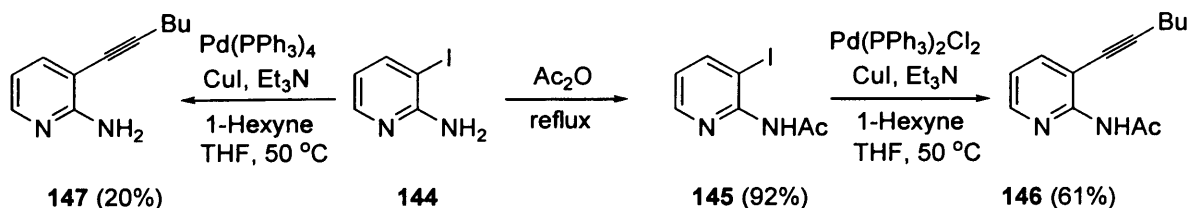
Scheme 51: Synthesis of 2-alkynyl amino-pyridines.
