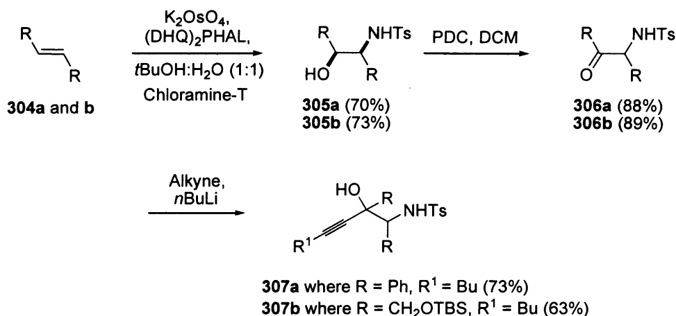
Scheme 100: Synthesis of substrates 307a and 307b . a is where R = Ph, b is where R = CH 2 OTBS.
