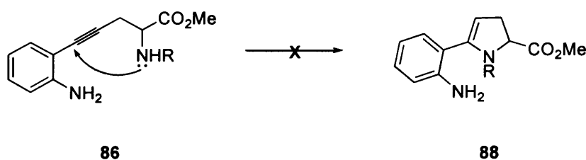
Scheme 31: Competing 5-endo-dig cyclisation (not observed).
