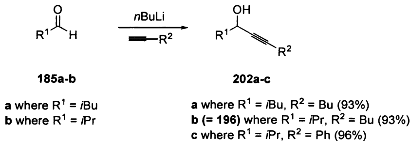
Scheme 65: Synthesis of propargylic alcohols.
