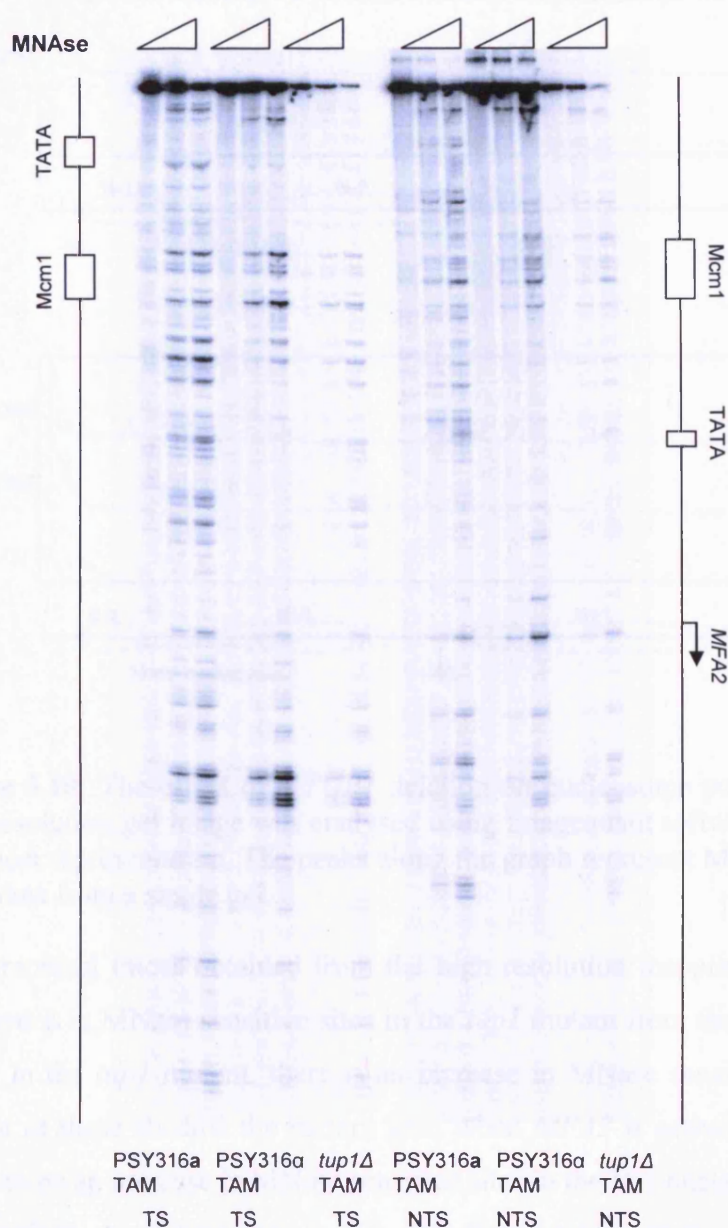
Figure 5.9: A typical high resolution nucleosome mapping gel, displaying WT a TAM, WT a TAM and tup1 \Delta TAM strains, treated with increasing amounts of MNase. The gel shows the Hae III restriction fragment, representing the MFA2 promoter region.
