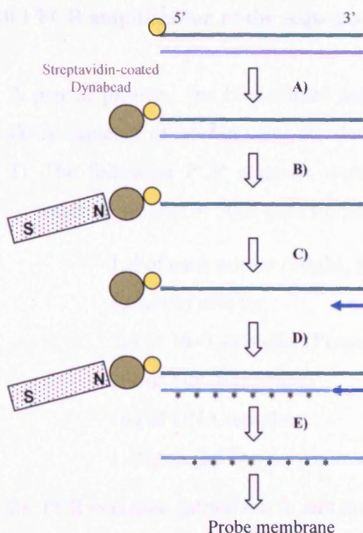
Figure 2.3: PCR directed amplification of a dsDNA fragment of choice is carried out, with primers designed to incorporate a biotin label at the 5' end of one strand. This dsDNA fragment should be between 300-500bp long for maximum efficiency. The addition of biotin allows a means of separation via Streptavidin coated Dynabeads. (B) On denaturing the dsDNA, and using a magnetic particle collector (MPC), the Dynabead and bound biotin labelled strand can be purified. This strand is then used for a sequencing reaction using a primer against the 3' end and radiolabelled dATPs (D). This results in a complementary strand of DNA interdispersed with radioactive dATPs. These strands were then denatured as previous and separated once again using the MPC (E). The supernatant was collected containing the radioactive probe against the DNA sequence (and strand) of interest, and this was used to probe a membrane.
