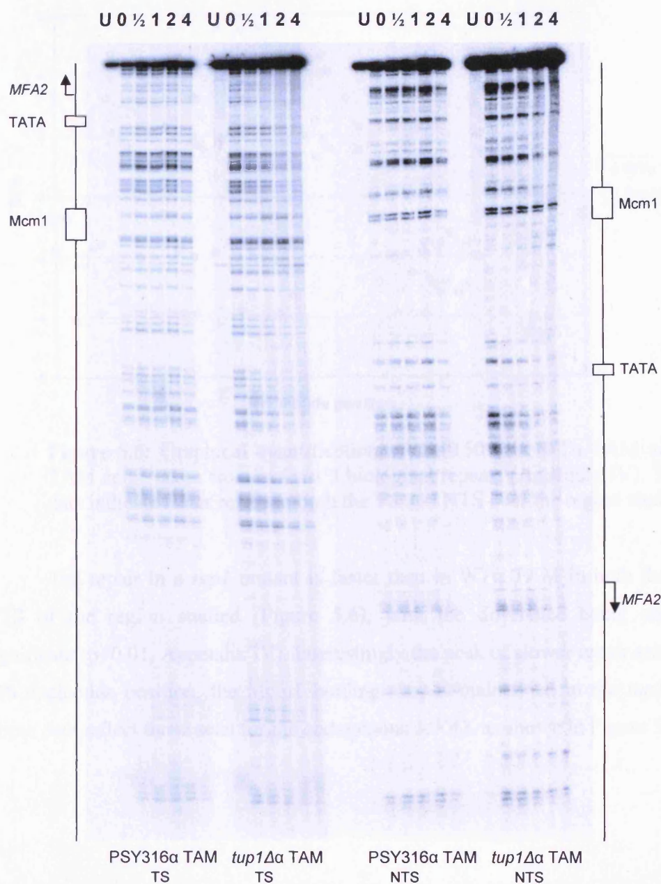
Figure 5.5: A typical high resolution gel image displaying the CPD profiles in WTα TAM and tup1Δα TAM cells. Cells were subjected to 100J/m 2 UV light and allowed to repair for various time points (U,0,0.5,1,2,4 hours) in YPD at 30°C. Following digestion with Hae III and ML endo , samples were end-labelled and resolved on a polyacrylamide gel. TS and NTS displayed.
