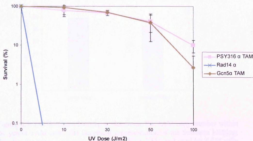
Figure 6.2: UV survival curves displaying the slightly reduced UV survival (%) of the gcn5α TAM strain (Appendix V).
