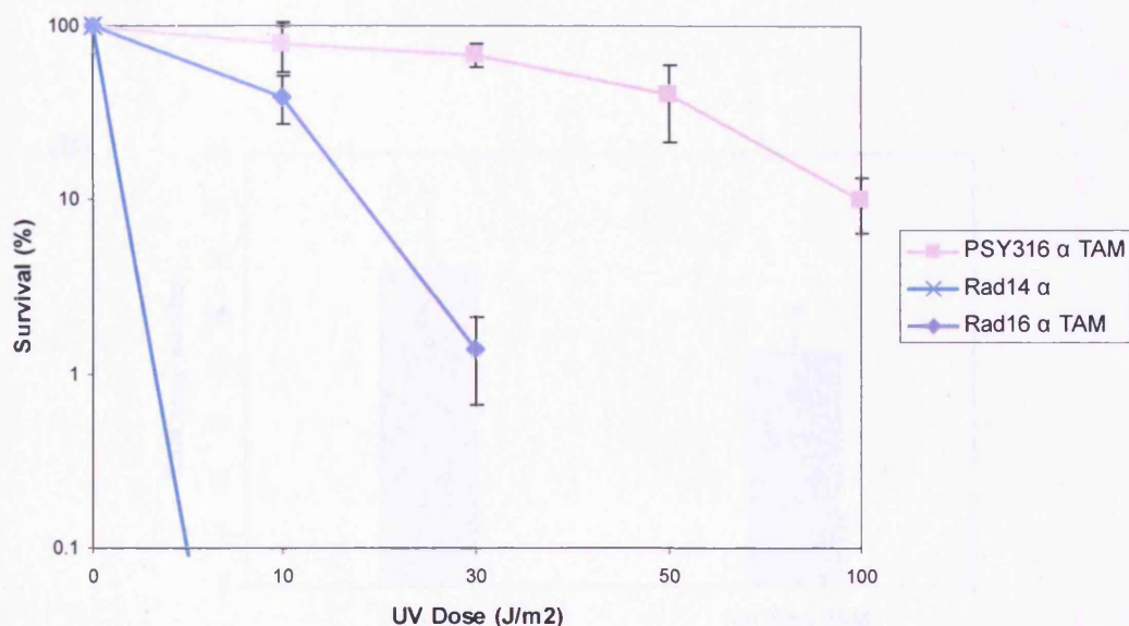
Figure 7.3: The UV survival was calculated for the rad16α TAM strain. Also shown is the WTα TAM strain, and the UV sensitive The rad14α strain for comparison. Rad14 is an essential NER factor, conferring considerable UV sensitivity (Appendix VI).
