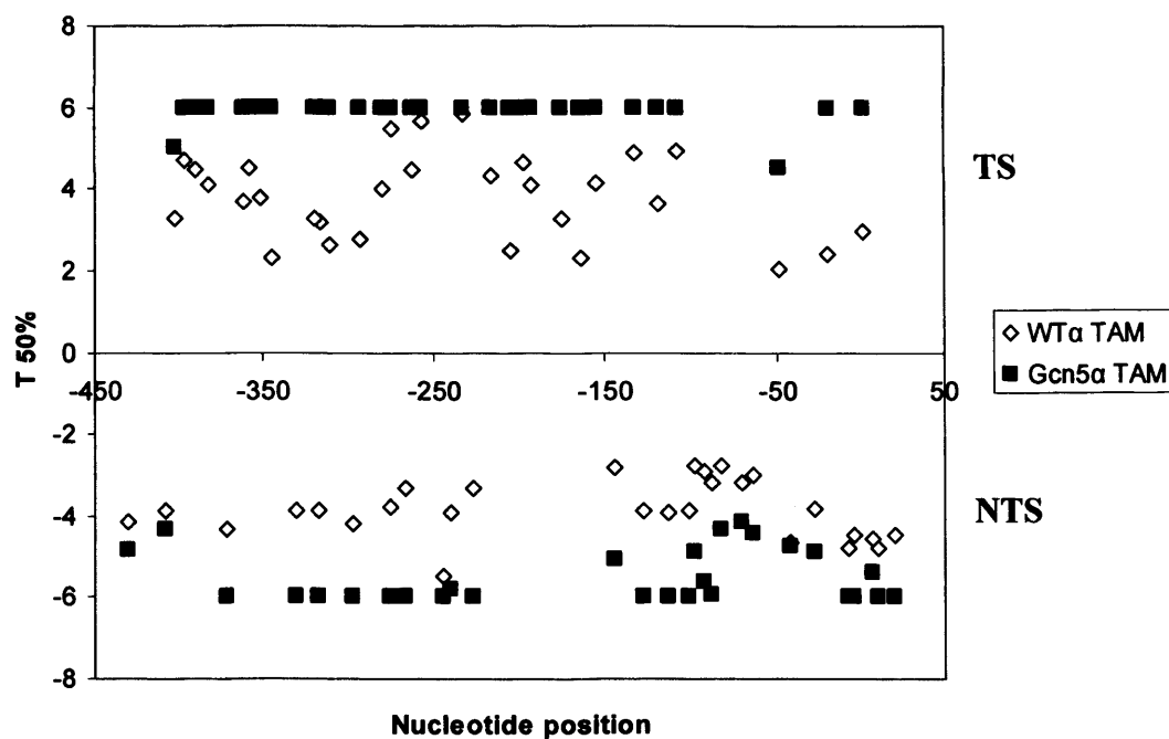
Figure 6.6: Graphical quantification of the T50% in WTα TAM and gcn5Δα cells, taken from 3 biological repeats (Appendix V). Little or no repair is seen in both strands of the MFA2 promoter region after 6 hours when GCN5 is absent.
