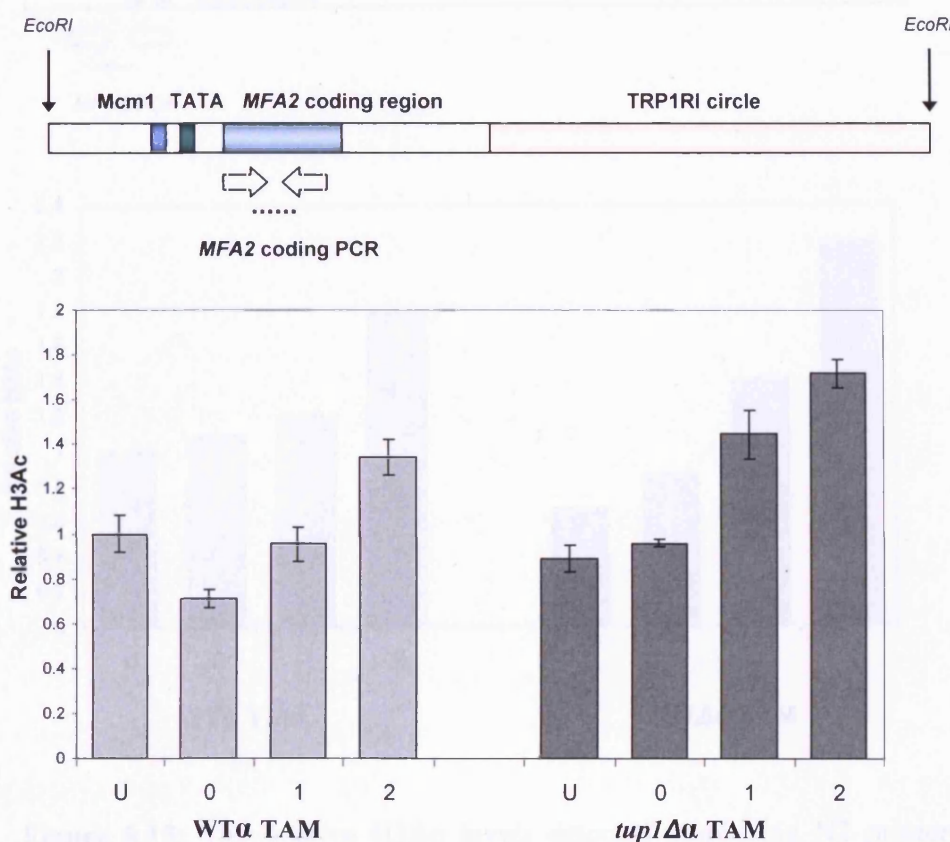
Figure 5.12: Relative H3Ac levels in WTα TAM and tup1Δα TAM cells for the MFA2 coding region, employing N1 primers, from 3 repeats (Appendix IV), normalised to WTα TAM U sample.
