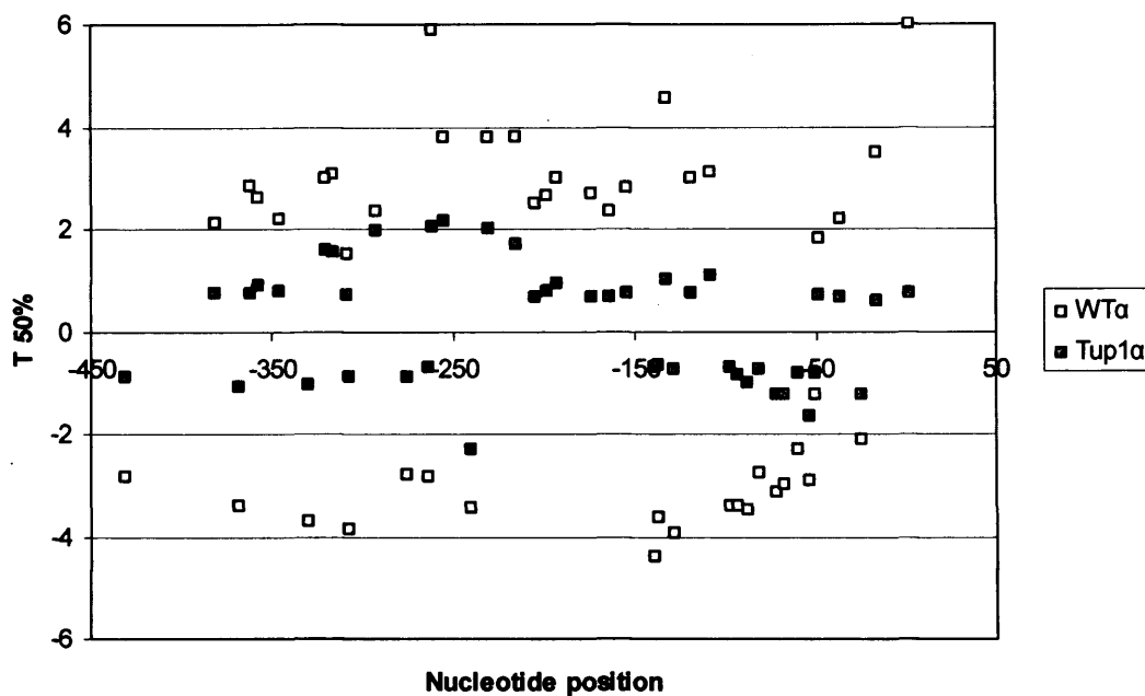
Figure 5.7: Repair profile for the endogenous MFA2 region of interest in WTα and tup1α cells (Appendix IV).
