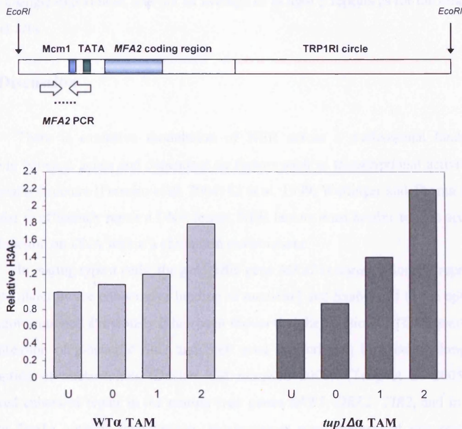
Figure 5.13: The relative H3Ac levels detected employing N2 primers, to amplify the MFA2 promoter region. Data taken from a single experiment (Appendix IV), normalised to WT \alpha TAM U sample.
