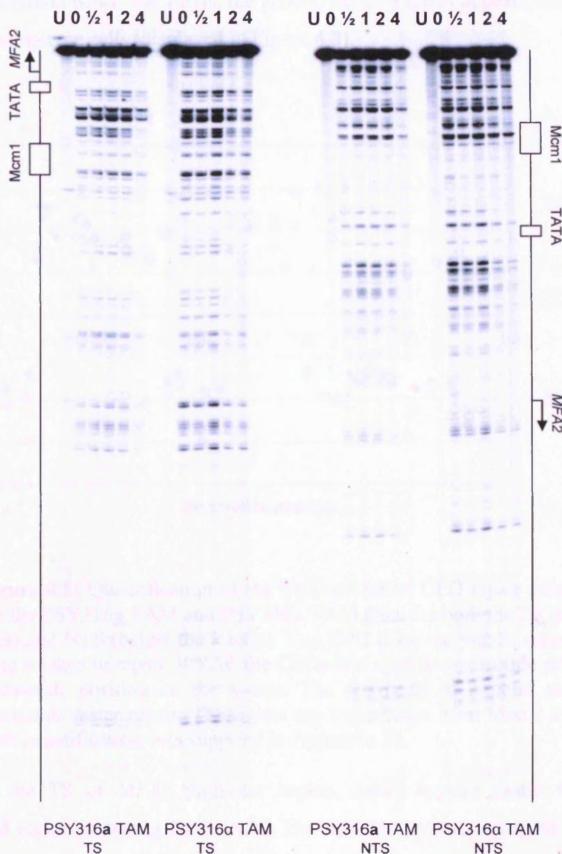
Figure 4.7: A typical gel image of high resolution CPD repair in PSY316a TAM and PSY316α TAM cells. The cells were subjected to 100\text{J/m}^2 UV light and allowed to repair for various time points (U: untreated, 0, 0.5, 1, 2, 4 hours repair) in YPD at 30^\circ\text{C} . DNA was isolated and digested with HaeIII , and cleaved specifically at CPD sites using ML endo . The purified DNA fragments were end-labelled with [\alpha\text{-}^{32}\text{P}]\text{dATP} and resolved by electrophoresis on a polyacrylamide gel. Displayed are the gels showing the transcribed strand (TS) on the left and non-transcribed strand (NTS) on the right.
