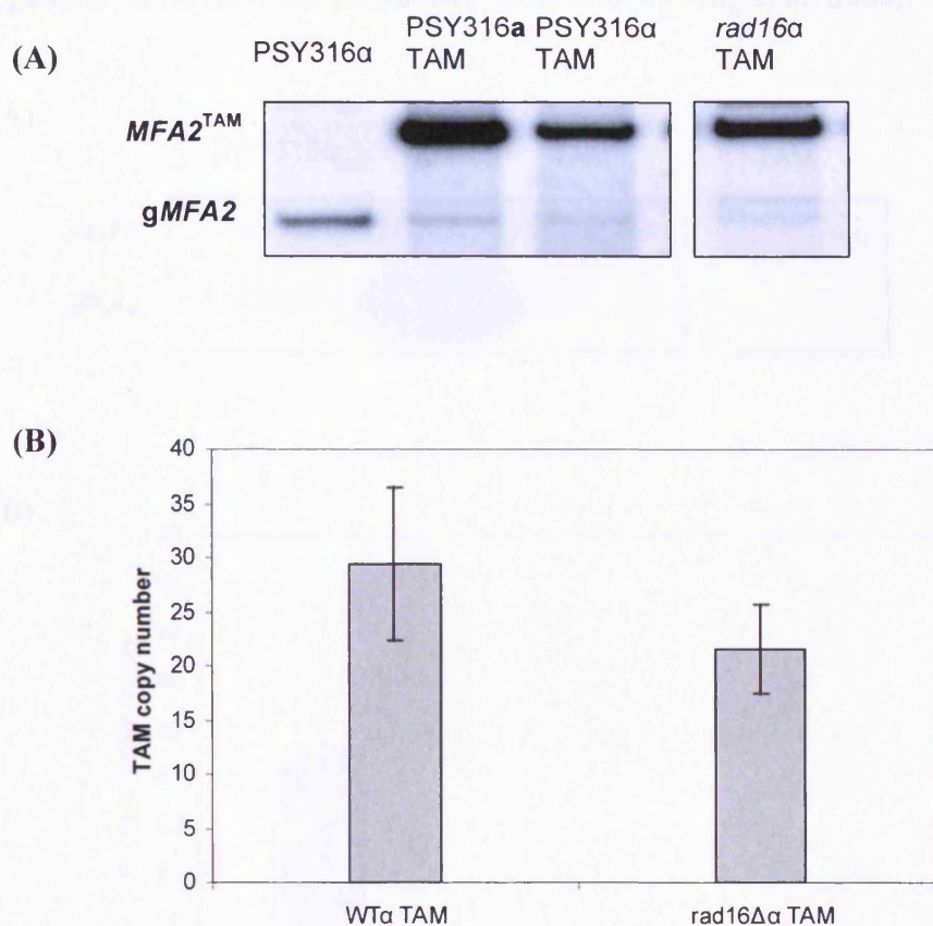
Figure 7.4: (A) Southern blot analysis, using a probe for MFA2 , to determine the relative copy number of the TAM plasmid within the various strains. (B) Graphical representation of the mean copy number in WT \alpha TAM and rad16 \alpha cells (Appendix VI).
