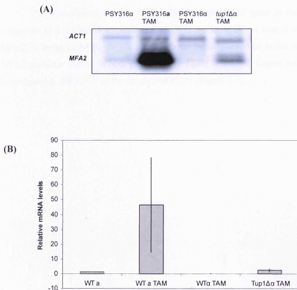
Figure 5.4: Northern blot analysis of relative MFA2 mRNA levels. A de-repression of MFA2 is seen, however, not to the expected levels seen in WT \alpha cells (Appendix IV).
