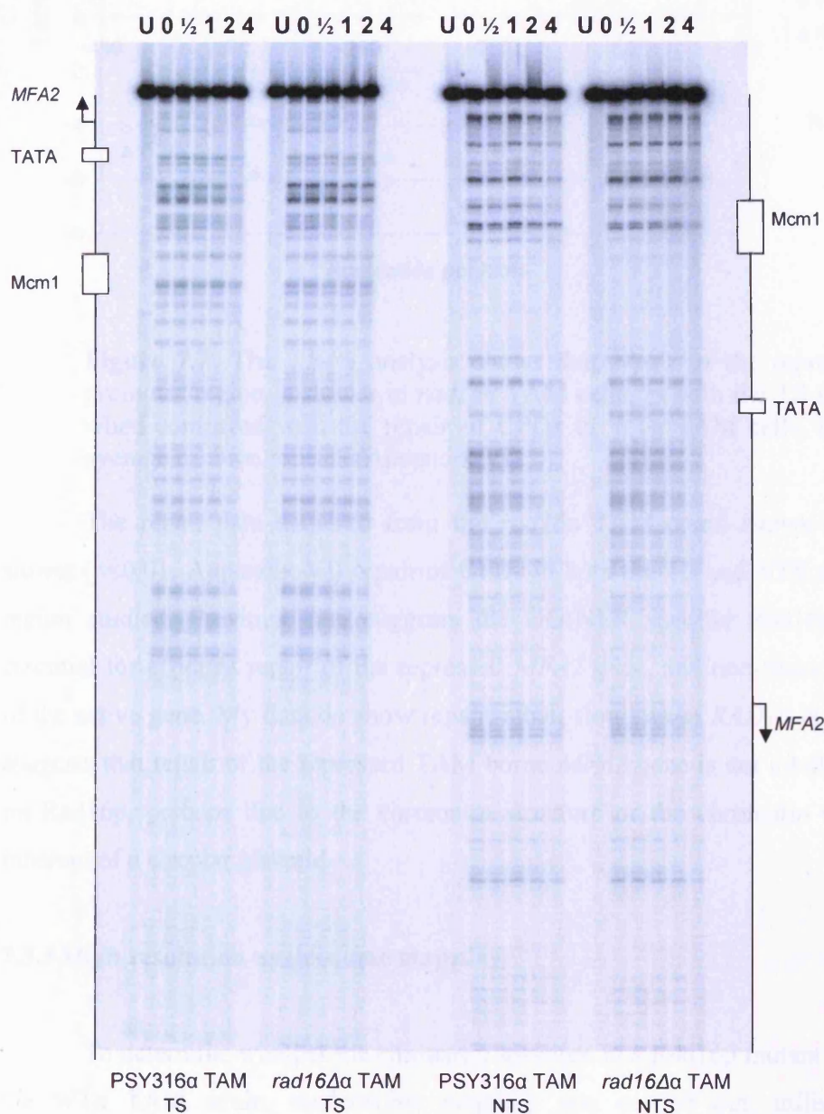
Figure 7.6: A typical high resolution gel to detect CPD repair in WTα TAM and rad16α TAM cells. A decrease in signal across a specific CPD-indicating band is representative of repair at that lesion. However, precise extents of repair are only arrived at following quantification of bands, and these images should not be used as indications of repair extents. TS and NTS displayed.
