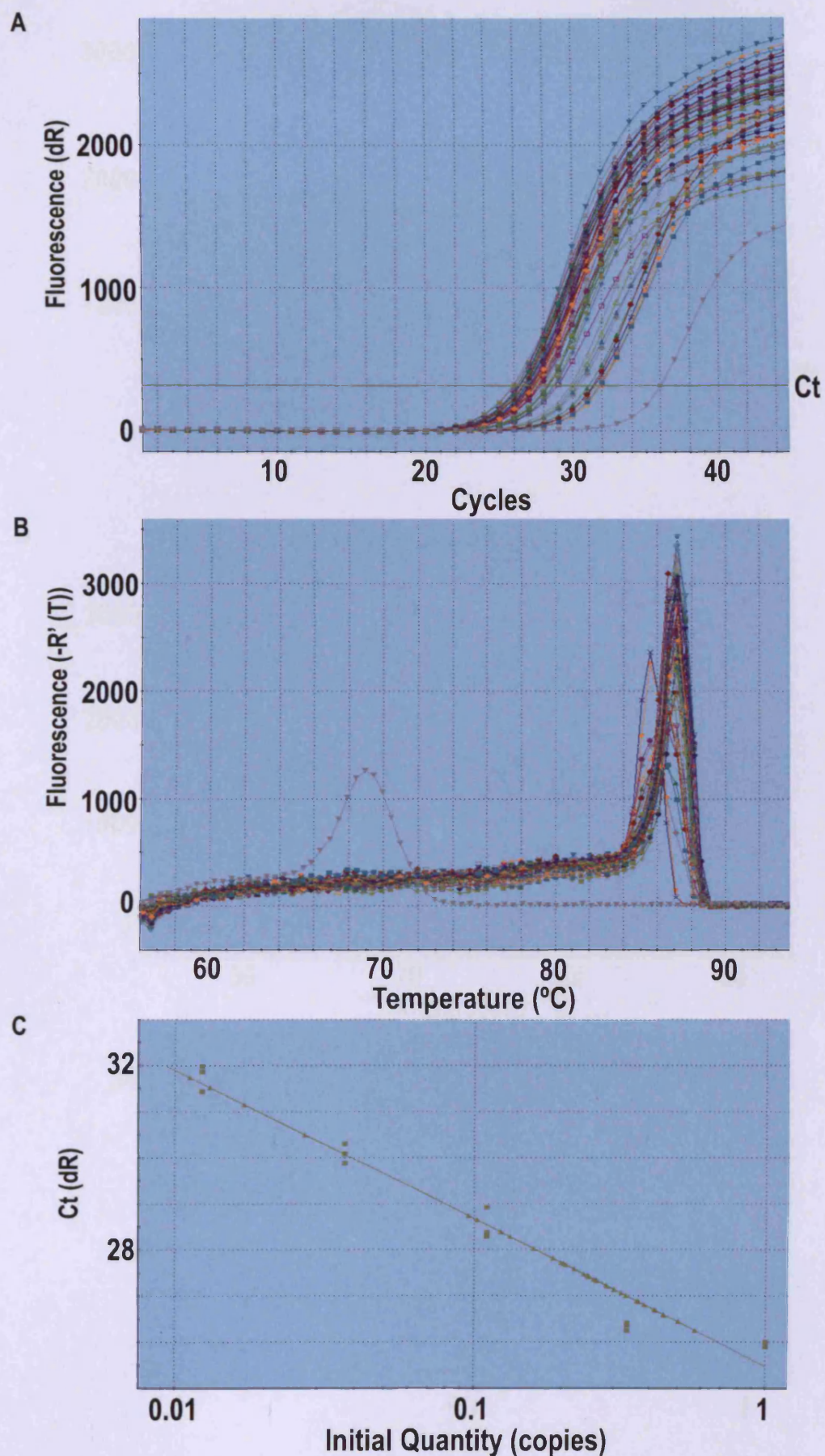
Figure 2. UBC QPCR consolidation experiment 1. (A) Amplification plot. (B) Dissociation curve. (C) Standard curve. Ct, Cycle threshold; dR, magnitude of fluorescence of Reporter dye; -R' (T) , negative first-derivative of the melting curve; T, Temperature.
