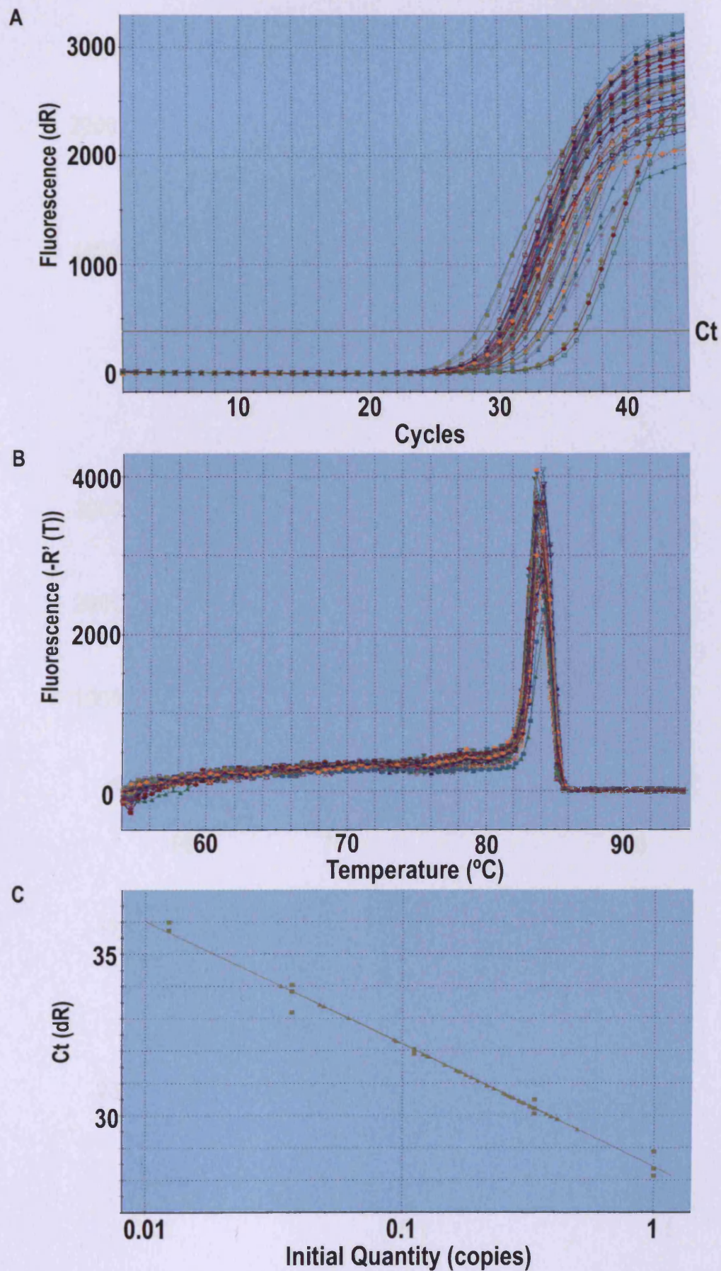
Figure 1. EGR3 QPCR consolidation experiment 1. (A) Amplification plot. (B) Dissociation curve. (C) Standard curve. Ct, Cycle threshold; dR, magnitude of fluorescence of Reporter dye; -R' (T) , negative first-derivative of the melting curve; T, Temperature.
