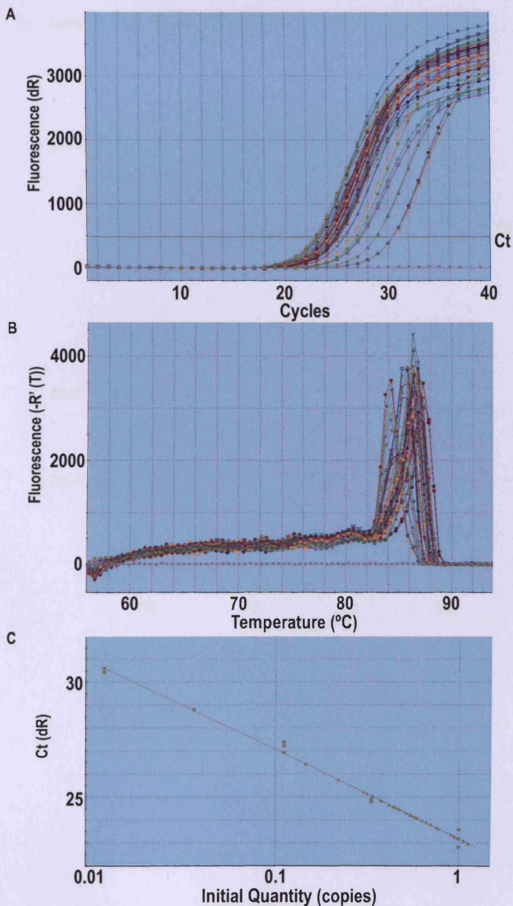
Figure 5. UBC QPCR consolidation experiment 2. (A) Amplification plot. (B) Dissociation curve. (C) Standard curve. Ct, Cycle threshold; dR, magnitude of fluorescence of Reporter dye; -R' (T), negative first-derivative of the melting curve; T, Temperature.
