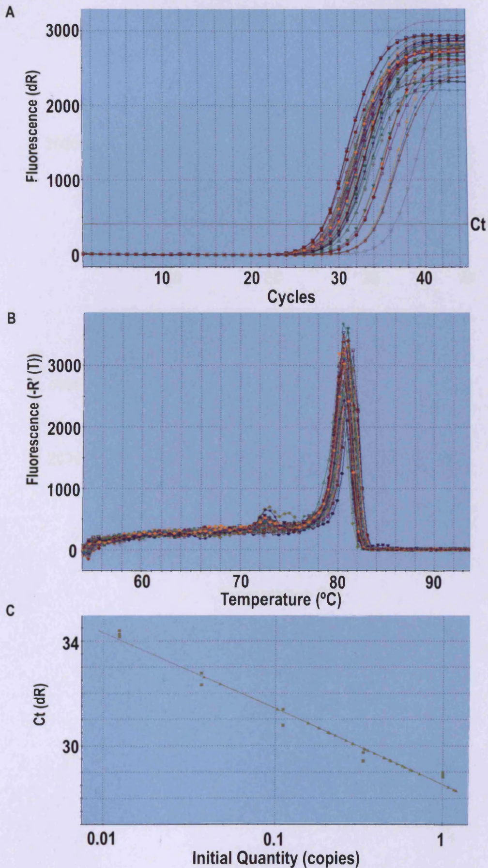
Figure 3. SDHA QPCR consolidation experiment 1. (A) Amplification plot. (B) Dissociation curve. (C) Standard curve. Ct, Cycle threshold; dR, magnitude of fluorescence of Reporter dye; -R'(T) , negative first-derivative of the melting curve; T, Temperature.
