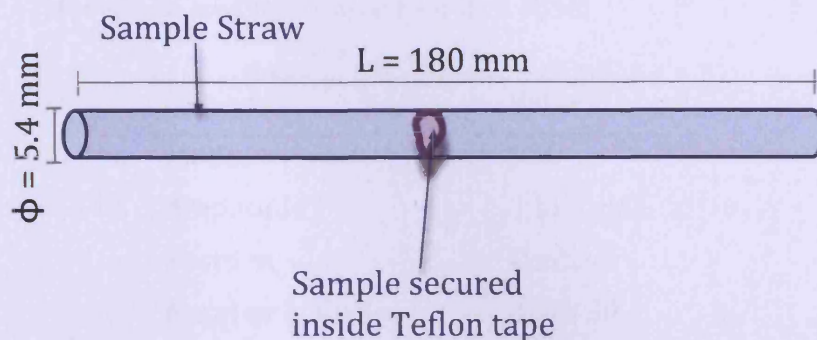
Figure 3-2 An illustration of how the sample was mounted inside the sample straw provided by Quantum Design.
