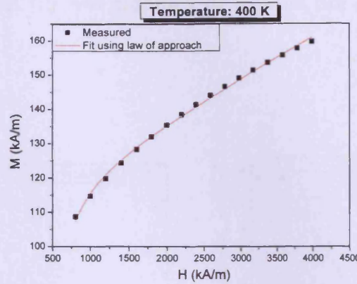
Figure 4-17 Fitting high field region M-H data for \text{CoGa}_{0.8}\text{Fe}_{1.2}\text{O}_4 at temperatures in the range 10 - 400 K.
