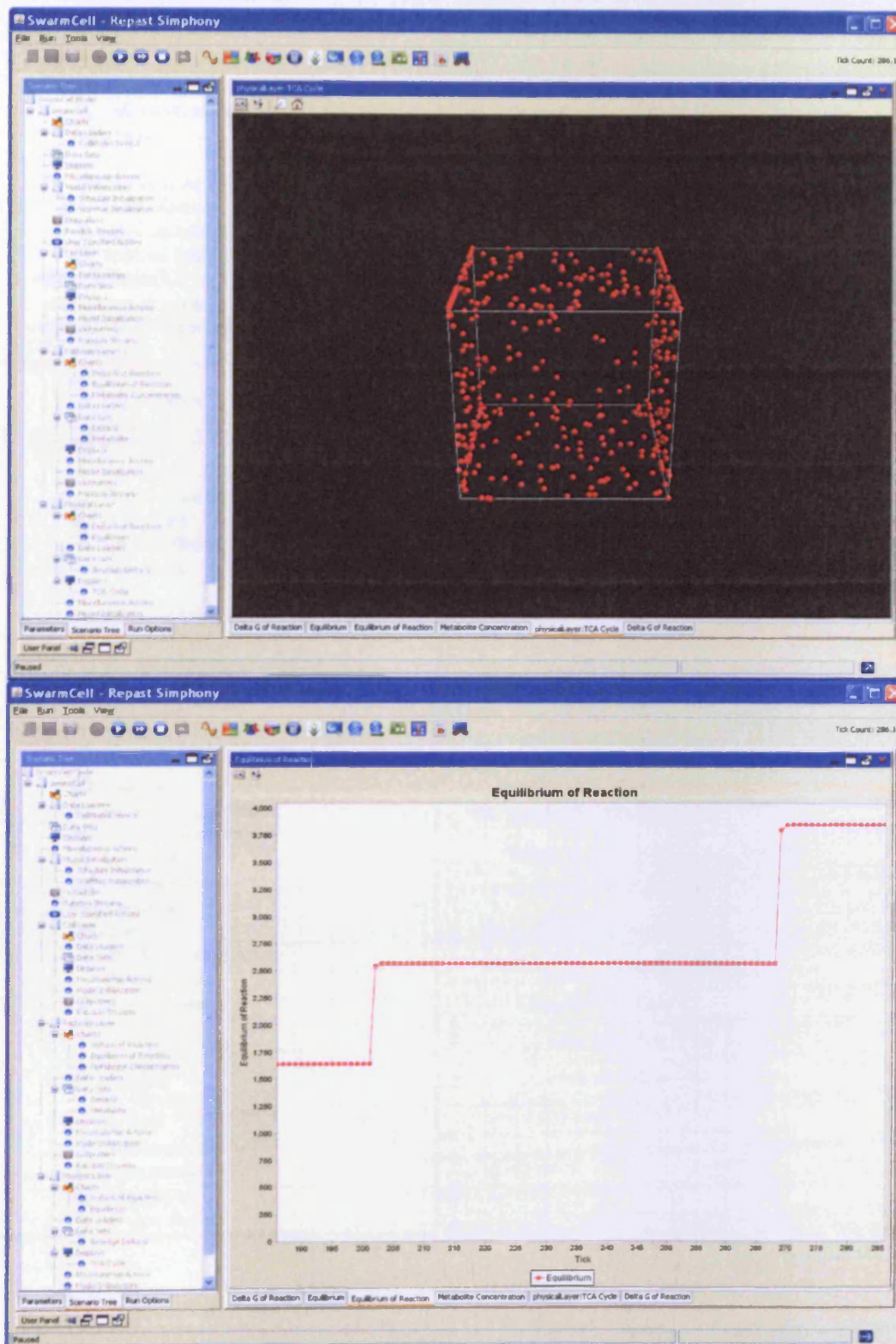
Figure 6.8: SwarmCell Interface.
